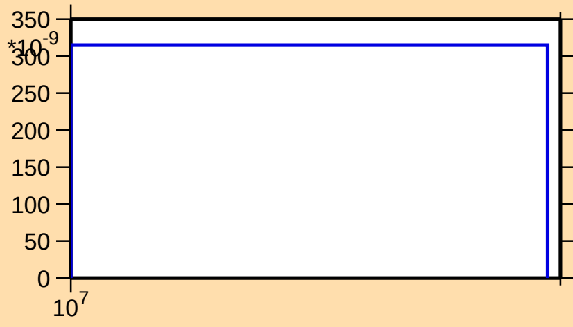
\sigma vs. E for ^{134}\text{Cs}(n,\text{nd})
