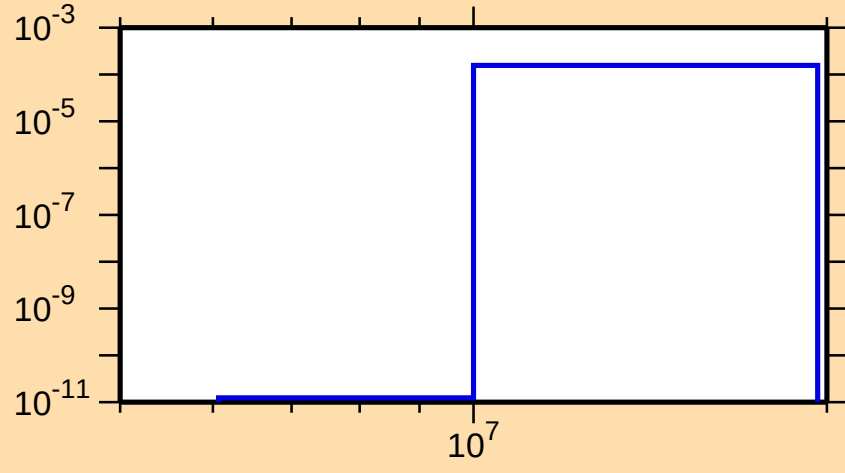
\sigma vs. E for ^{134}\text{Cs}(n,t)
