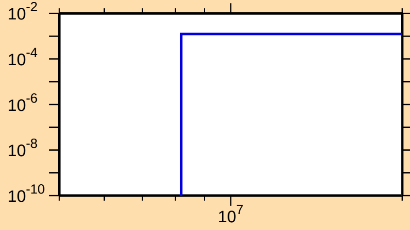
\sigma vs. E for ^{134}\text{Cs}(n,np)
