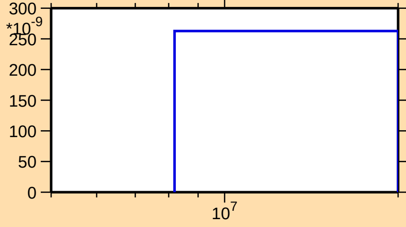
\sigma vs. E for ^{134}\text{Cs}(n,\text{nd})
