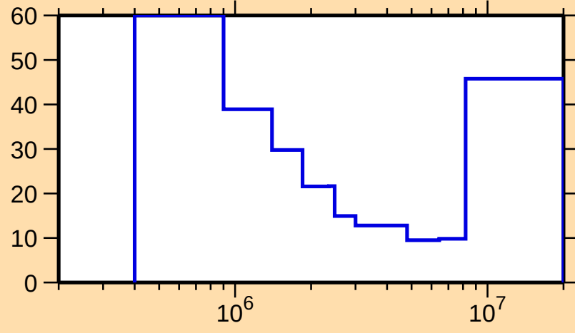
\Delta\sigma/\sigma vs. E for ^{134}\text{Cs}(n,n\text{cont.})
