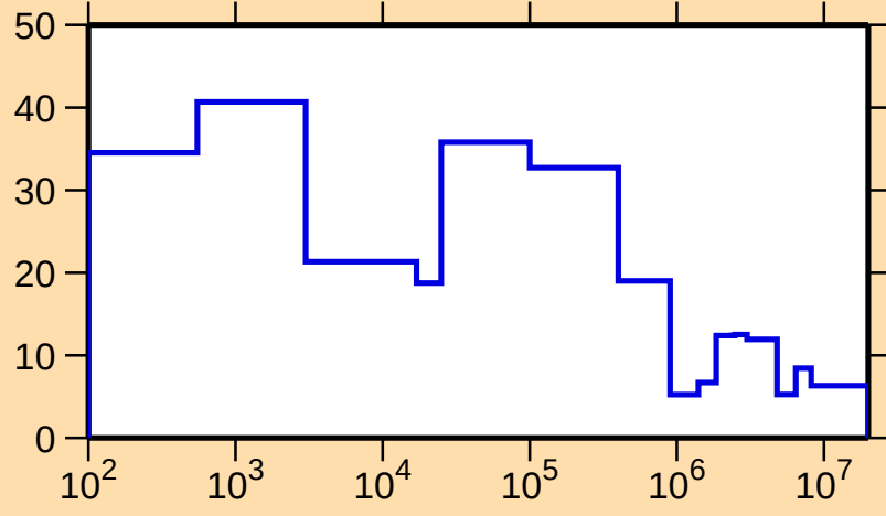
\Delta\sigma/\sigma vs. E for ^{134}\text{Cs}(n,\text{el.})
