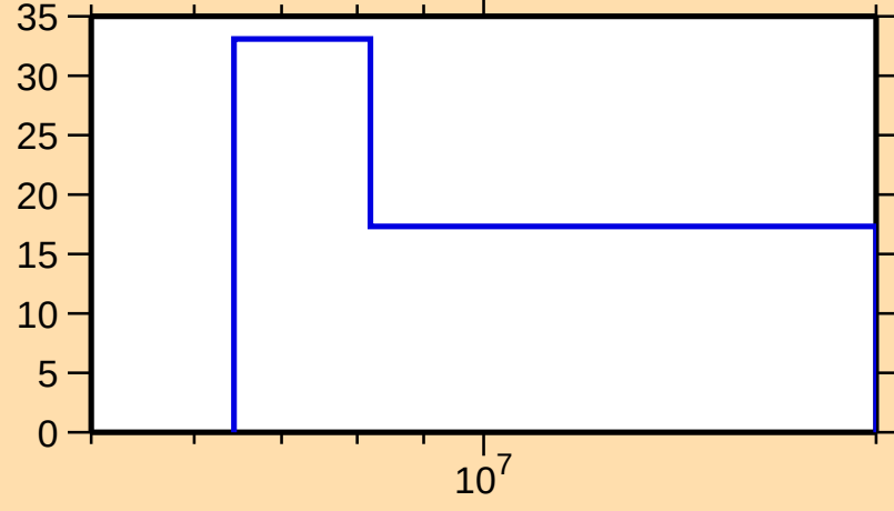
\Delta\sigma/\sigma vs. E for ^{134}\text{Cs}(n,2n)
