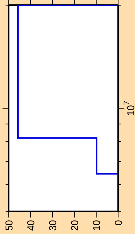
\Delta\sigma/\sigma vs. E for ^{134}\text{Cs}(n,n\text{cont.})
