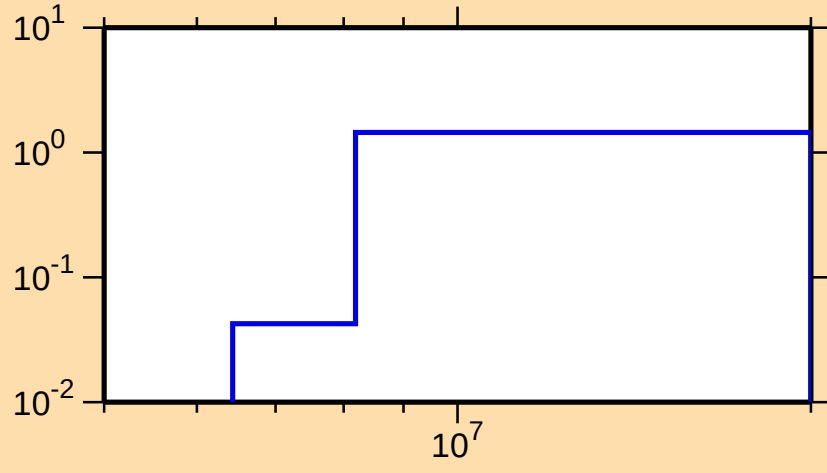
\sigma vs. E for ^{134}\text{Cs}(n,2n)
