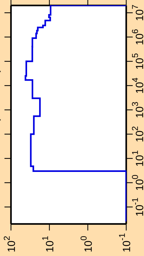
\Delta\sigma/\sigma vs. E for ^{134}\text{Cs}(n,\text{nonel.})
