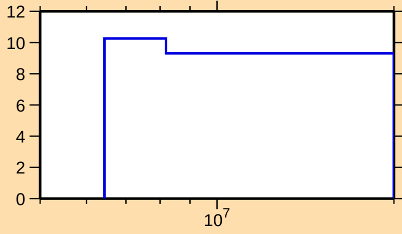
\Delta\sigma/\sigma vs. E for ^{134}\text{Cs}(n,\text{nonel.})
