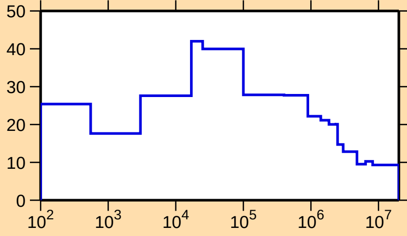
\Delta\sigma/\sigma vs. E for ^{134}\text{Cs}(n,\text{nonel.})
