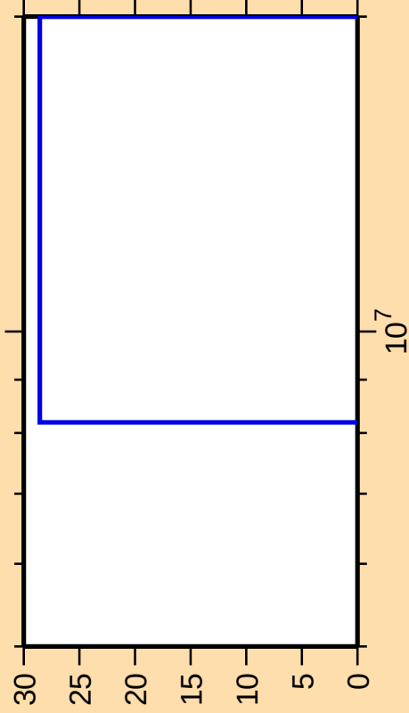
\Delta\sigma/\sigma vs. E for ^{134}\text{Cs}(n,3n)
