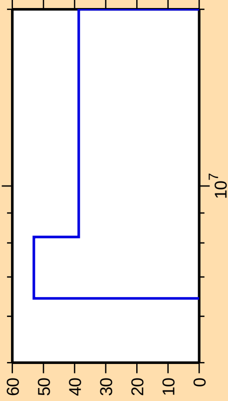
\Delta\sigma/\sigma vs. E for ^{134}\text{Cs}(n,\gamma)
