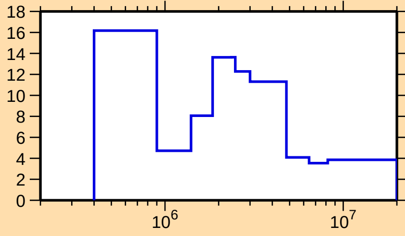
\Delta\sigma/\sigma vs. E for ^{134}\text{Cs}(n,\text{tot.})
