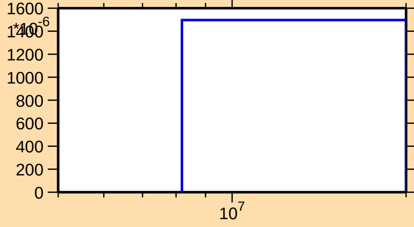
\sigma vs. E for ^{134}\text{Cs}(n,3n)
