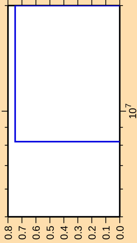
\Delta\sigma/\sigma vs. E for ^{134}\text{Cs}(n,p\alpha)
