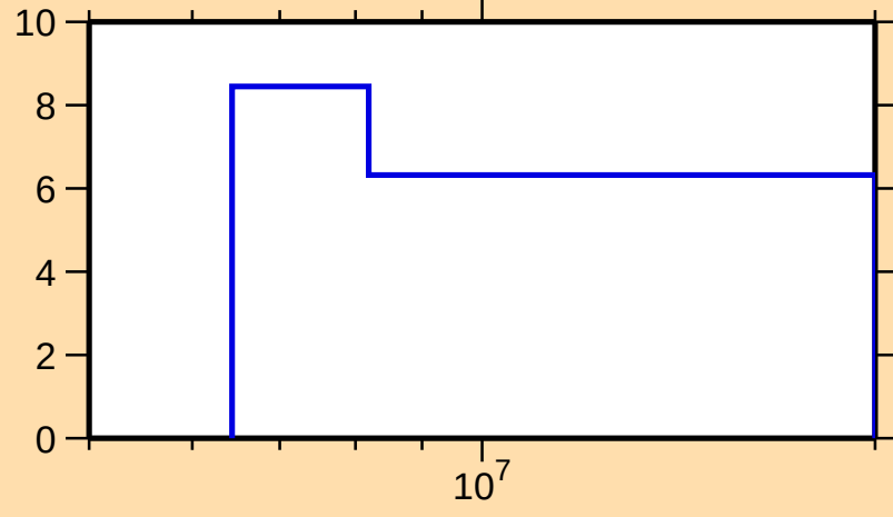
\Delta\sigma/\sigma vs. E for ^{134}\text{Cs}(n,\text{el.})
