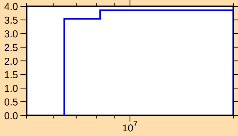
\Delta\sigma/\sigma vs. E for ^{134}\text{Cs}(n,\text{tot.})
