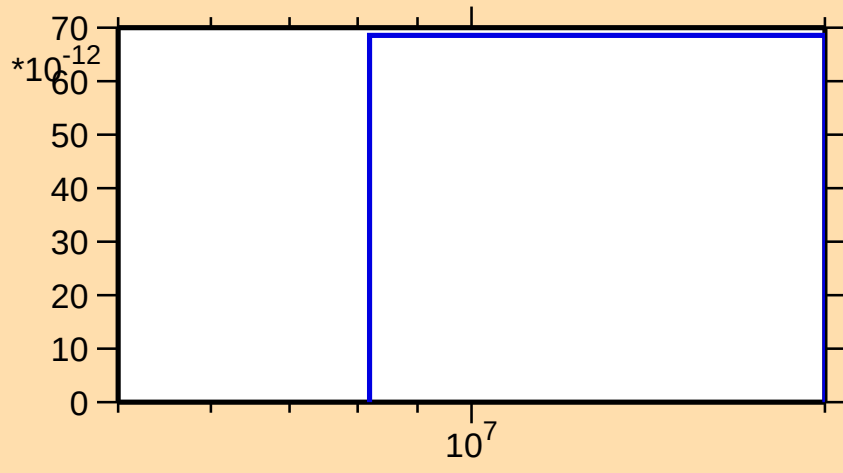
\sigma vs. E for ^{134}\text{Cs}(n,\text{He}3)
