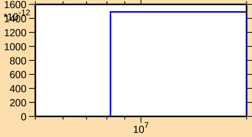
\sigma vs. E for ^{134}\text{Cs}(n,nt)
