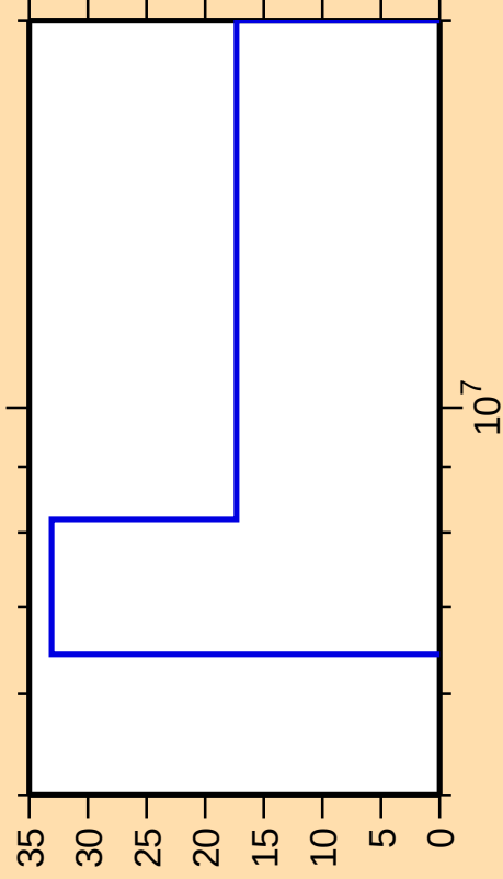
\Delta\sigma/\sigma vs. E for ^{134}\text{Cs}(n,2n)
