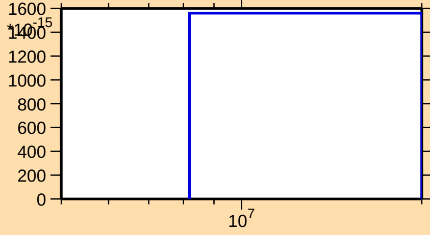
\sigma vs. E for ^{134}\text{Cs}(n,p\alpha)
