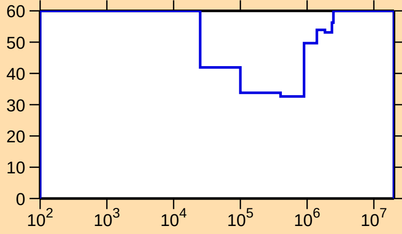
\Delta\sigma/\sigma vs. E for ^{134}\text{Cs}(n,n_1)
