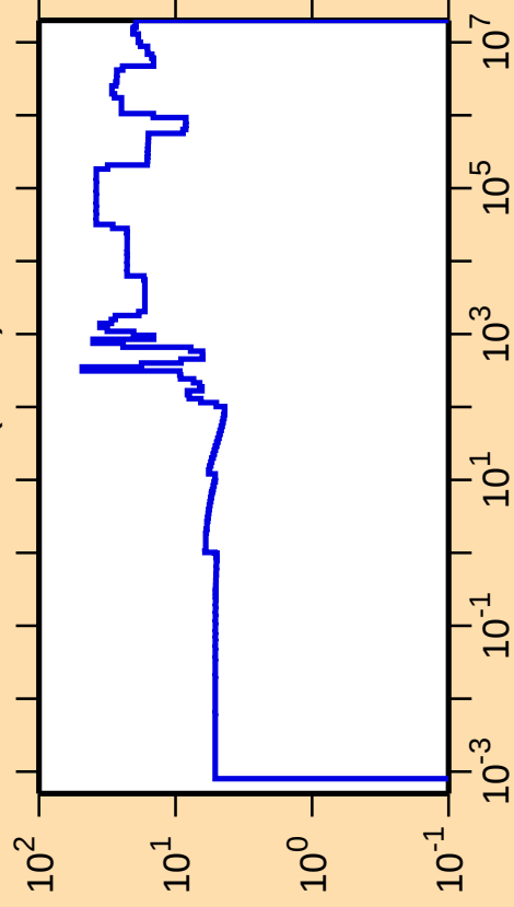
\Delta\sigma/\sigma vs. E for ^{135}\text{Cs}(n,\text{el.})
