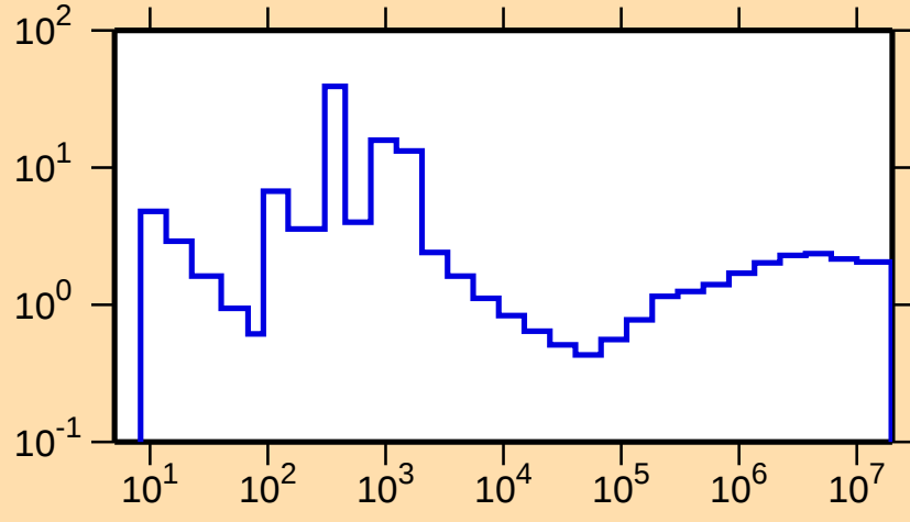
\sigma vs. E for ^{135}\text{Cs}(n,\text{nonel.})
