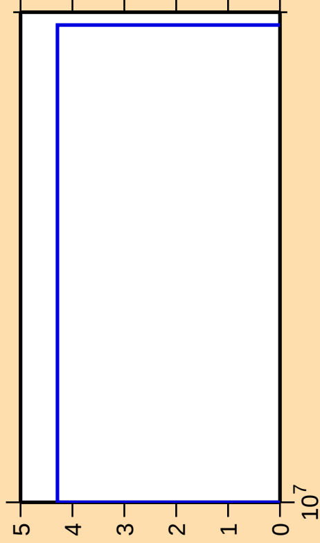
\Delta\sigma/\sigma vs. E for ^{135}\text{Cs}(n,p\alpha)
