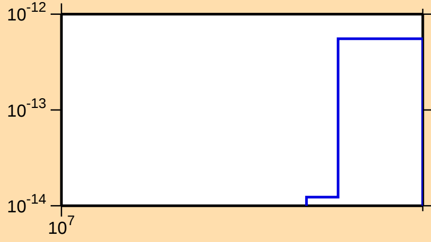
\sigma vs. E for ^{137}\text{Cs}(n,p\alpha)
