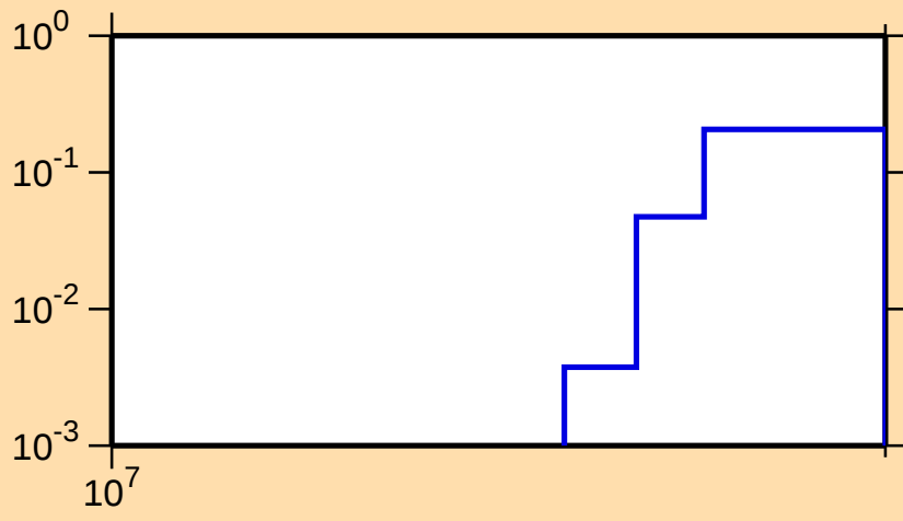
\sigma vs. E for ^{137}\text{Cs}(n,3n)
