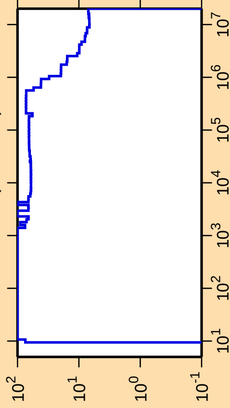
\Delta\sigma/\sigma vs. E for ^{137}\text{Cs}(n,\text{nonel.})
