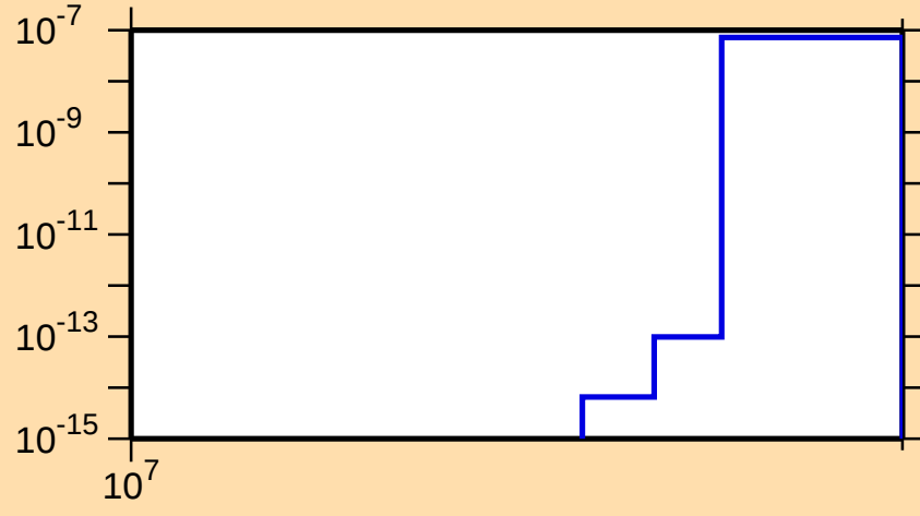
\sigma vs. E for ^{137}\text{Cs}(n,2np)
