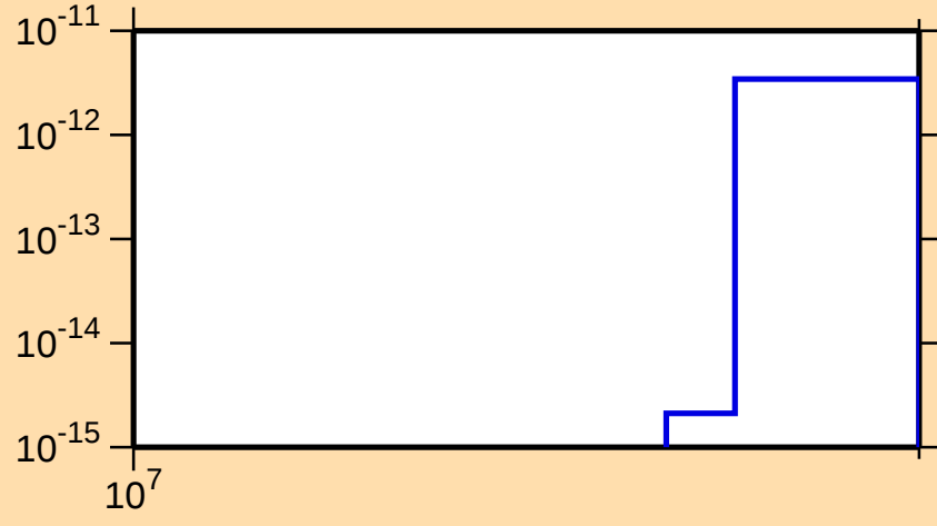
\sigma vs. E for ^{137}\text{Cs}(n,\text{He}3)
