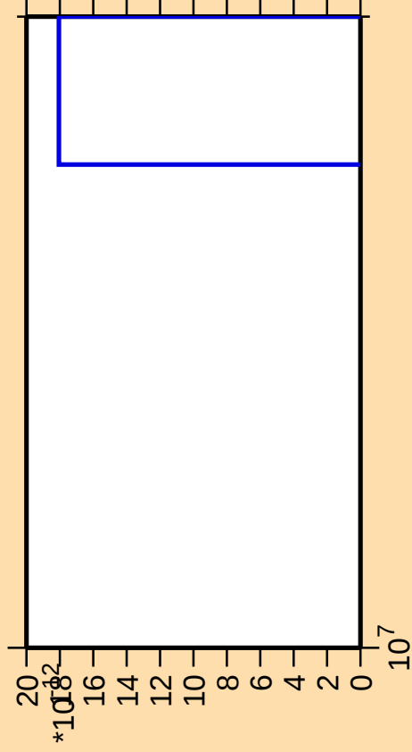
\Delta\sigma/\sigma vs. E for ^{137}\text{Cs} (mt 11)
