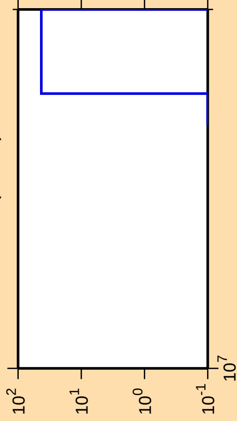
\Delta\sigma/\sigma vs. E for ^{137}\text{Cs}(n,2n\alpha)
