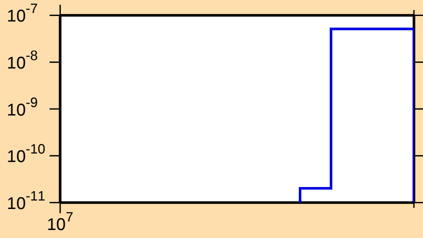
\sigma vs. E for ^{137}\text{Cs}(n,nt)
