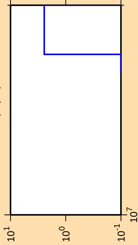
\Delta\sigma/\sigma vs. E for ^{137}\text{Cs}(n,p\alpha)
