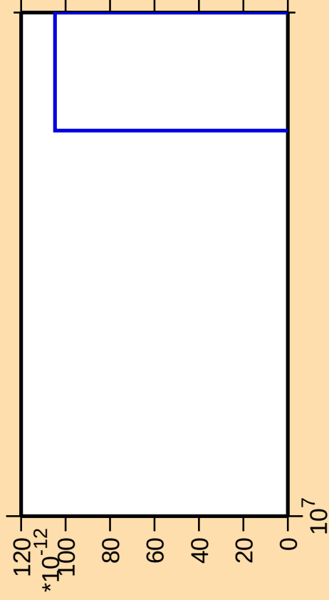
\Delta\sigma/\sigma vs. E for ^{138}\text{Cs} (mt 42)
