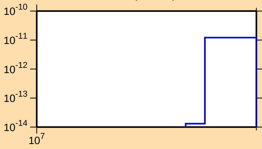
\sigma vs. E for ^{138}\text{Cs}(n,\text{He}3)
