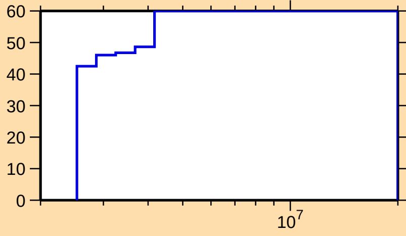
\Delta\sigma/\sigma vs. E for ^{138}\text{Cs}(n,\gamma)
