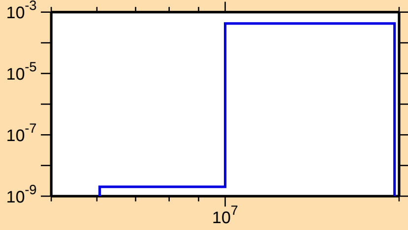
\sigma vs. E for ^{138}\text{Cs}(n,t)
