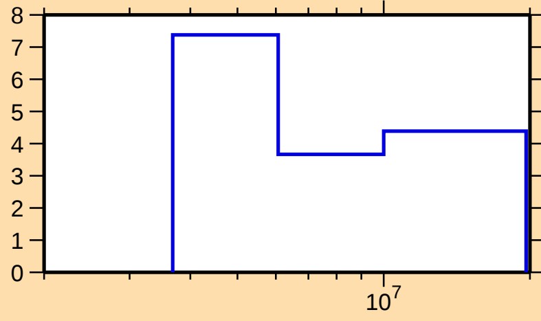
\Delta\sigma/\sigma vs. E for ^{138}\text{Cs}(n,\text{el.})
