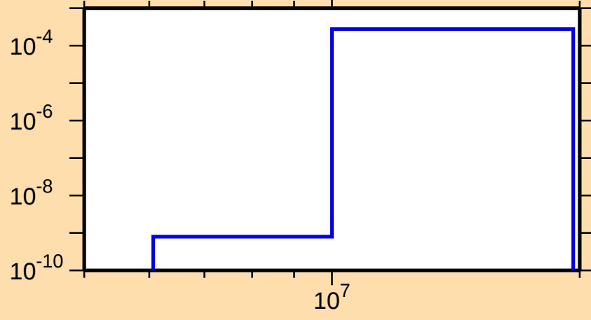
\sigma vs. E for ^{138}\text{Cs}(n,n\alpha)
