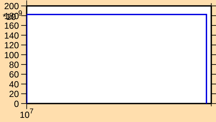
\sigma vs. E for ^{138}\text{Cs}(n,\text{nt})
