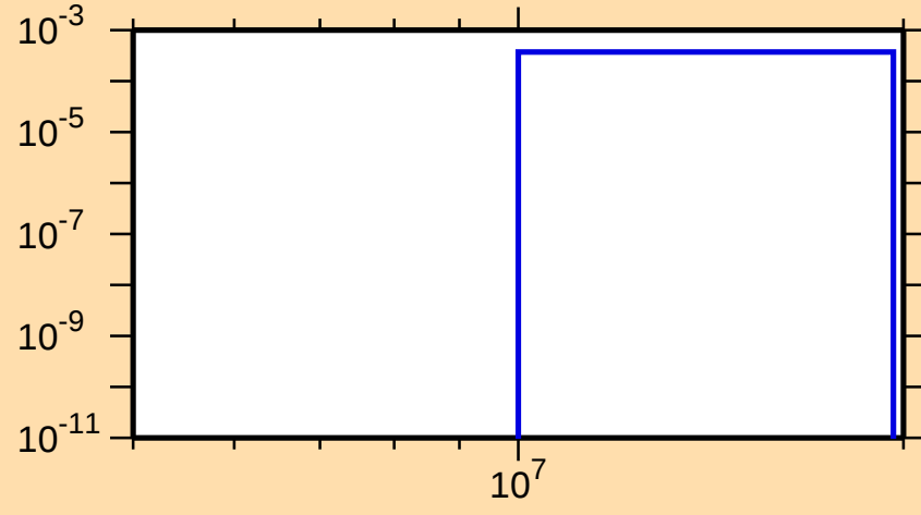
\sigma vs. E for ^{138}\text{Cs}(n,np)
