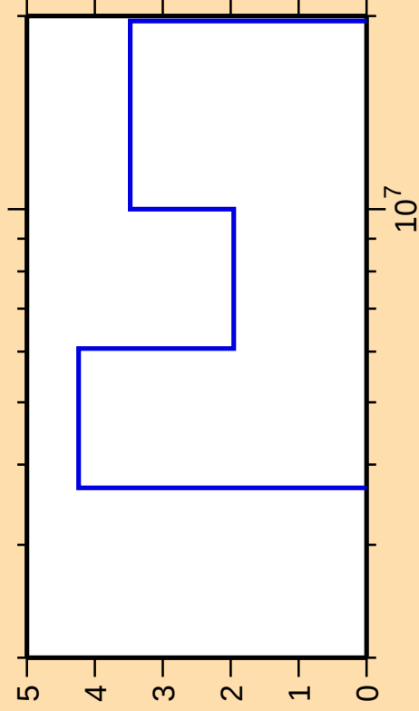
\Delta\sigma/\sigma vs. E for ^{138}\text{Cs}(n,2n)
