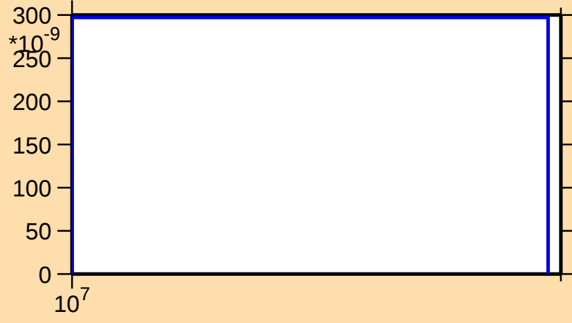
\sigma vs. E for ^{138}\text{Cs}(n,2np)
