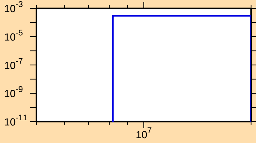
\sigma vs. E for ^{138}\text{Cs}(n,np)
