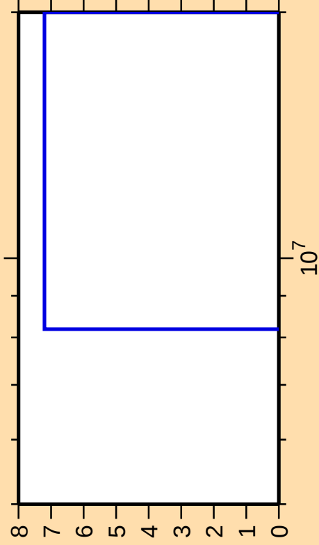
\Delta\sigma/\sigma vs. E for ^{138}\text{Cs}(n,3n)
