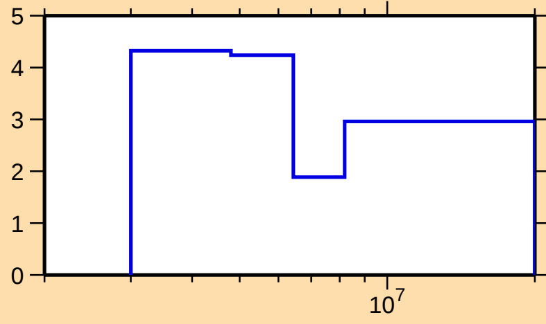
\Delta\sigma/\sigma vs. E for ^{138}\text{Cs}(n,2n)
