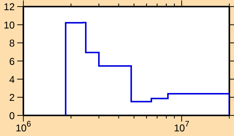
\Delta\sigma/\sigma vs. E for ^{138}\text{Cs}(n,\text{tot.})
