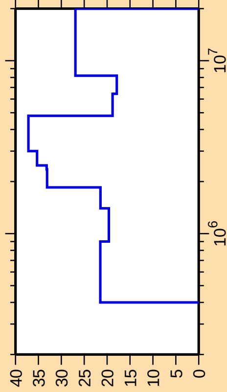
\Delta\sigma/\sigma vs. E for ^{139}\text{Cs}(n,n_4)
