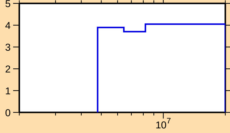
\Delta\sigma/\sigma vs. E for ^{139}\text{Cs}(n,\text{nonel.})
