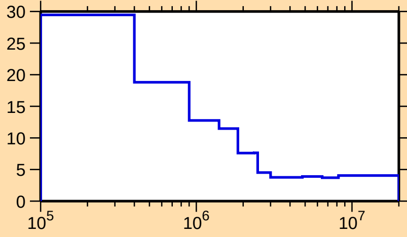
\Delta\sigma/\sigma vs. E for ^{139}\text{Cs}(n,\text{nonel.})
