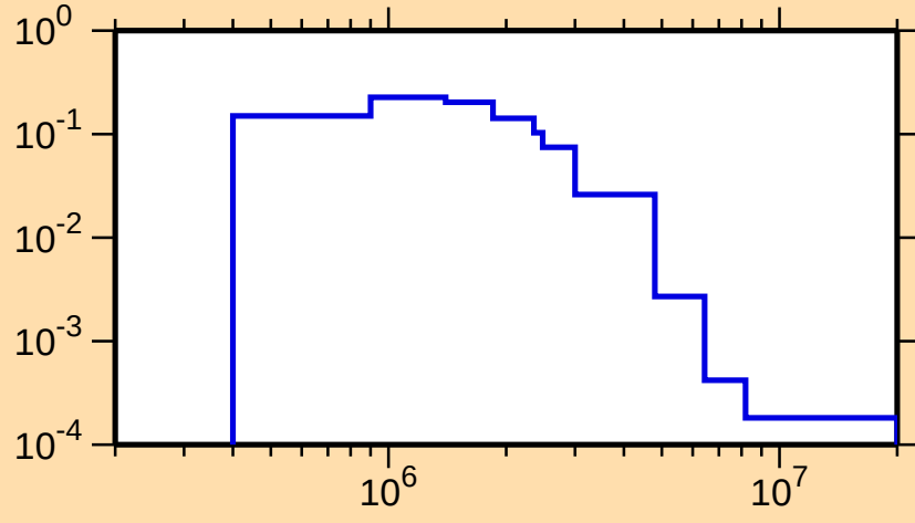
\sigma vs. E for ^{139}\text{Cs}(n,n_4)
