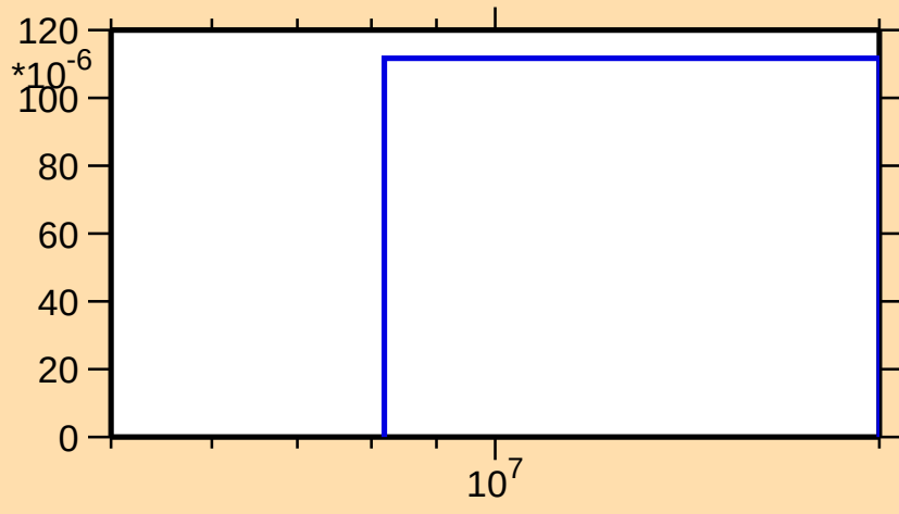
\sigma vs. E for ^{139}\text{Cs}(n,np)
