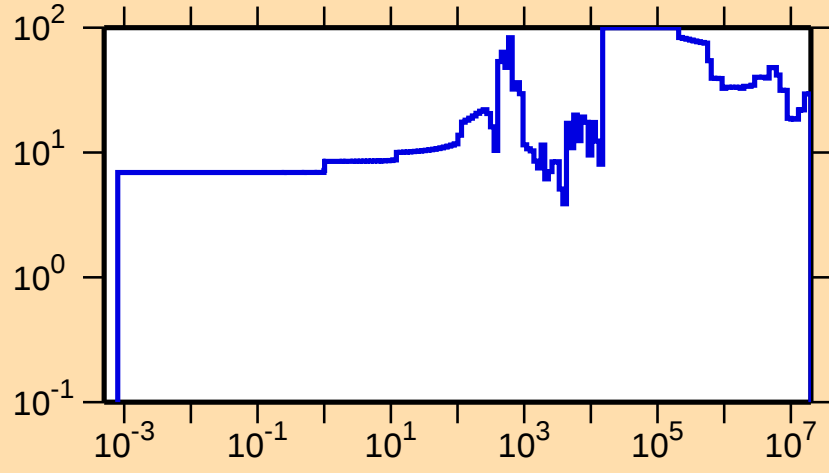
\Delta\sigma/\sigma vs. E for ^{140}\text{Cs}(n,\text{el.})
