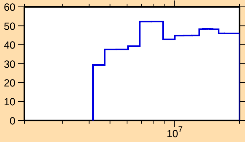
\Delta\sigma/\sigma vs. E for ^{140}\text{Cs}(n,\text{inel.})
