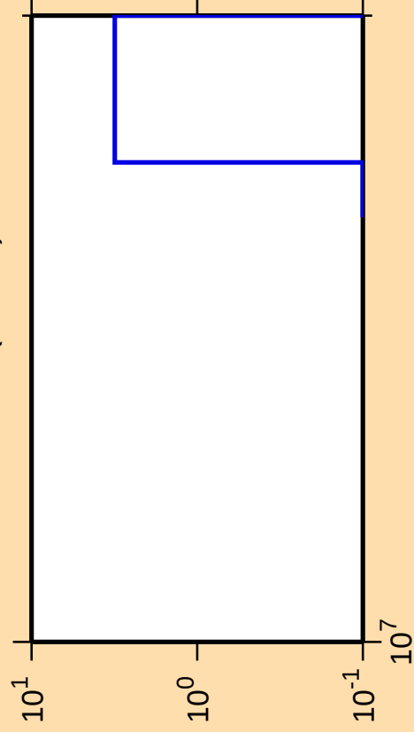
\Delta\sigma/\sigma vs. E for ^{140}\text{Cs}(n,3n\alpha)
