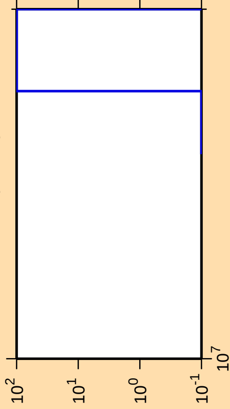
\Delta\sigma/\sigma vs. E for ^{140}\text{Cs} (mt 11)
