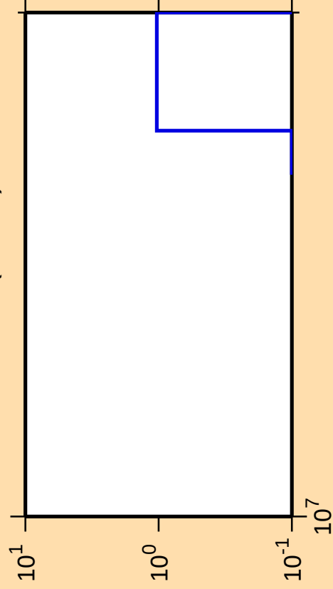
\Delta\sigma/\sigma vs. E for ^{140}\text{Cs}(n,\text{He}3)
