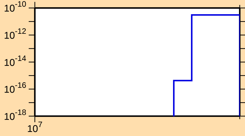
\sigma vs. E for ^{140}\text{Cs} (mt 11)
