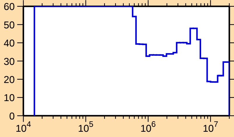
\Delta\sigma/\sigma vs. E for ^{140}\text{Cs}(n,\text{el.})
