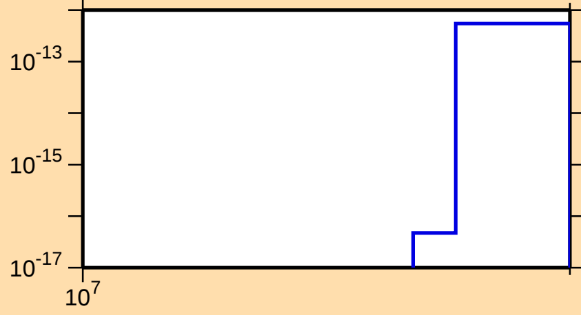
\sigma vs. E for ^{140}\text{Cs}(n,3n\alpha)
