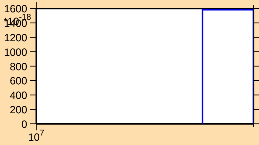
\sigma vs. E for ^{140}\text{Cs} (mt 42)
