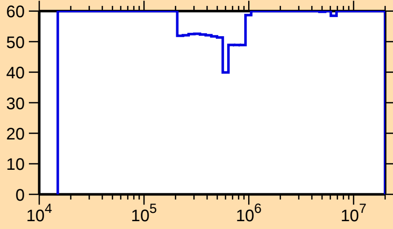
\Delta\sigma/\sigma vs. E for ^{140}\text{Cs}(n,n_1)
