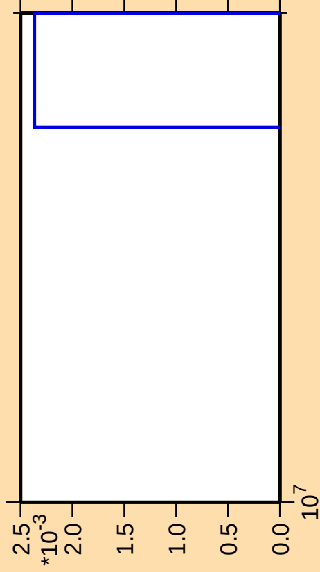
\Delta\sigma/\sigma vs. E for ^{140}\text{Cs} (mt 42)
