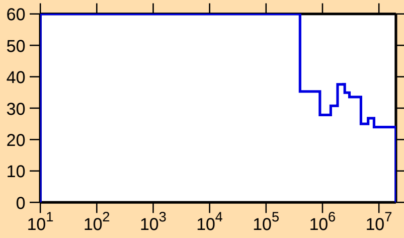
\Delta\sigma/\sigma vs. E for ^{140}\text{Cs}(n,\text{nonel.})
