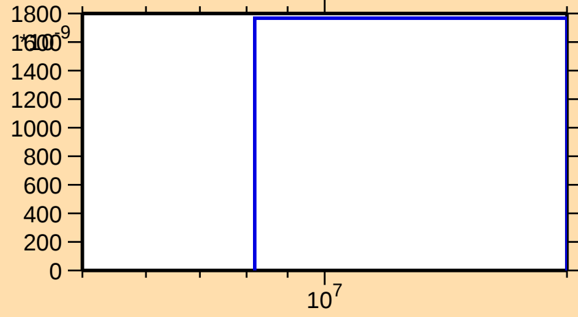
\sigma vs. E for ^{140}\text{Cs}(n,\text{nd})
