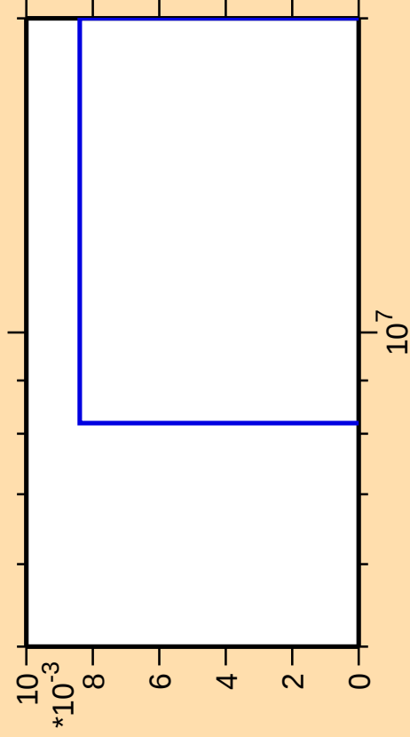
\Delta\sigma/\sigma vs. E for ^{140}\text{Cs}(n,\text{He}3)
