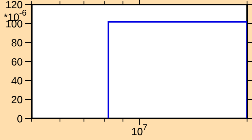
\sigma vs. E for ^{140}\text{Cs}(n,np)
