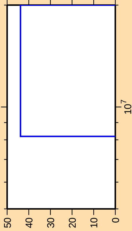
\Delta\sigma/\sigma vs. E for ^{140}\text{Cs}(n,3n)
