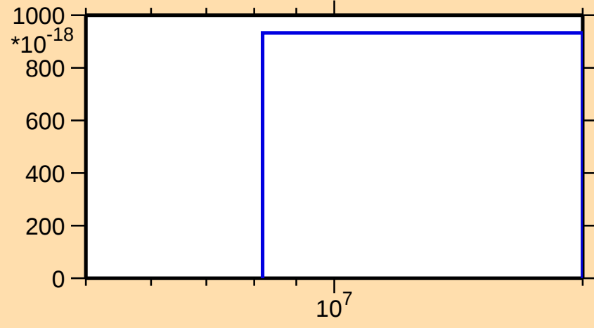
\sigma vs. E for ^{140}\text{Cs}(n,\text{He}3)
