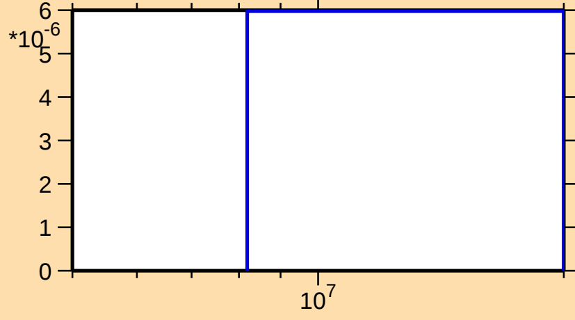
\sigma vs. E for ^{140}\text{Cs}(n,nt)
