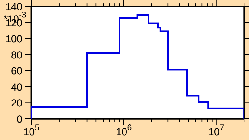
\sigma vs. E for ^{141}\text{Cs}(n,n_4)
