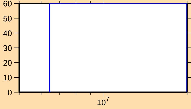
\Delta\sigma/\sigma vs. E for ^{141}\text{Cs}(n,n_1)
