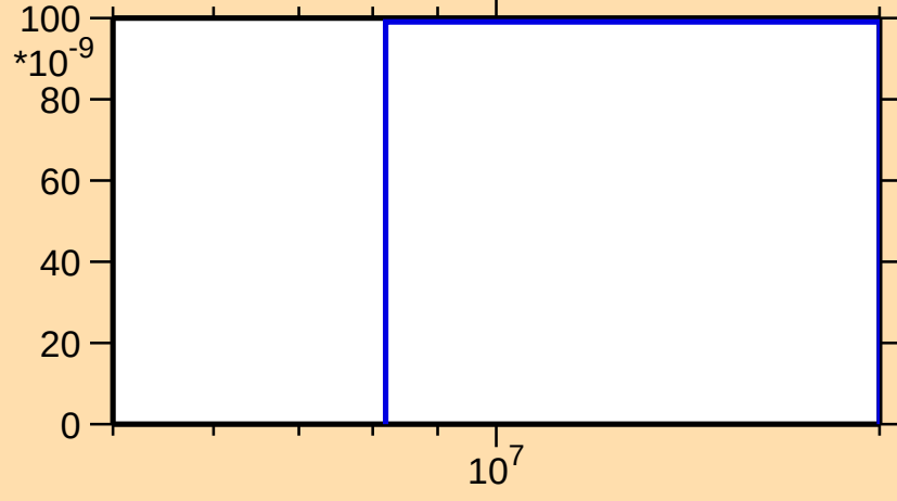
\sigma vs. E for ^{141}\text{Cs}(n,\text{nd})
