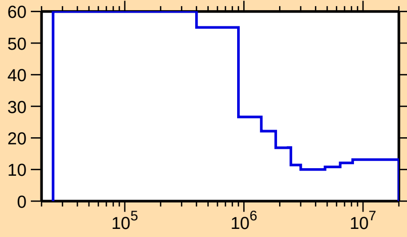
\Delta\sigma/\sigma vs. E for ^{141}\text{Cs}(n,\text{nonel.})
