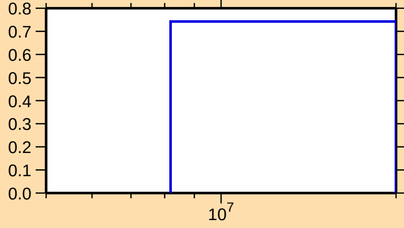
\sigma vs. E for ^{141}\text{Cs}(n,3n)
