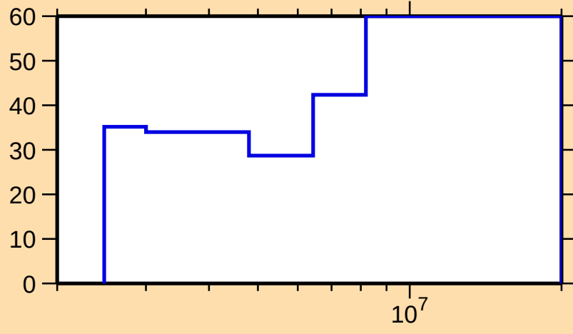
\Delta\sigma/\sigma vs. E for ^{141}\text{Cs}(n,n\text{cont.})
