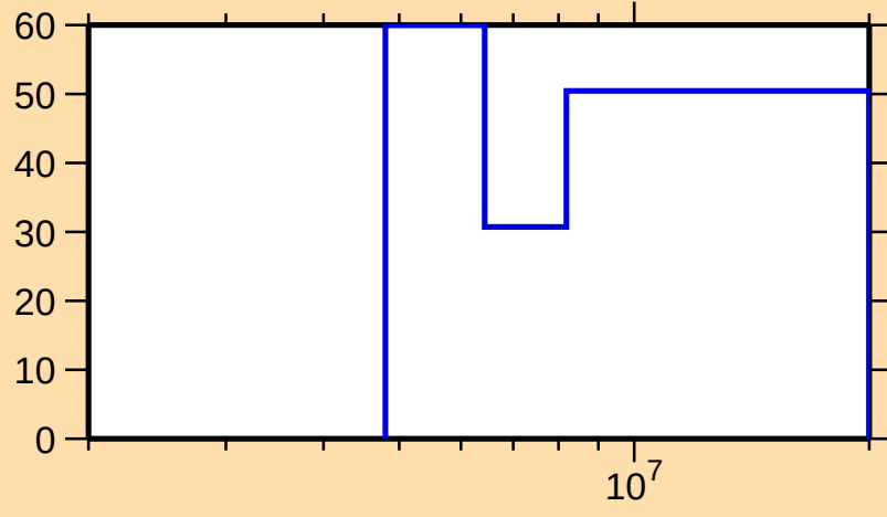
\Delta\sigma/\sigma vs. E for ^{141}\text{Cs}(n,2n)
