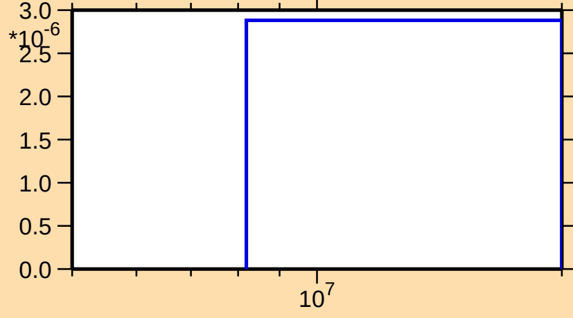
\sigma vs. E for ^{141}\text{Cs}(n,nt)
