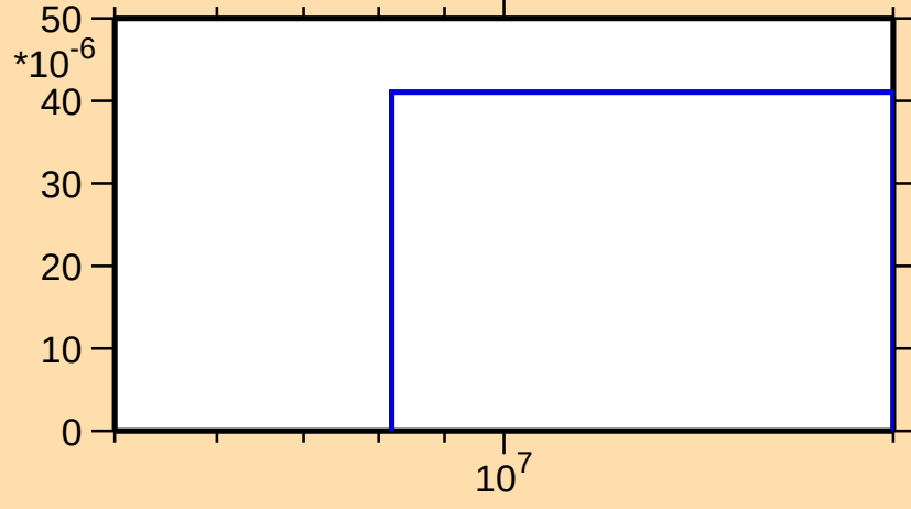
\sigma vs. E for ^{141}\text{Cs}(n,np)
