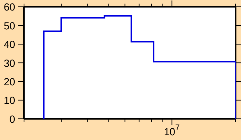
\Delta\sigma/\sigma vs. E for ^{141}\text{Cs}(n,\text{el.})
