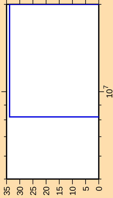
\Delta\sigma/\sigma vs. E for ^{141}\text{Cs}(n,3n)
