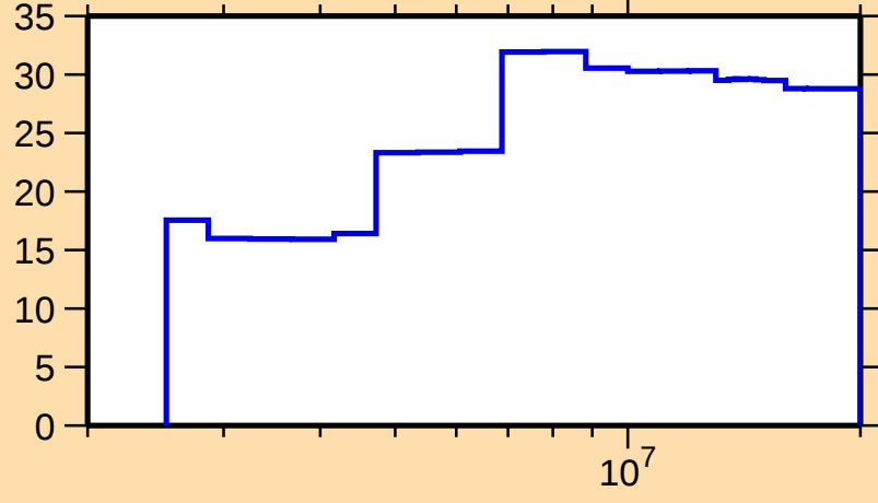
\Delta\sigma/\sigma vs. E for ^{142}\text{Cs}(n,n\text{cont.})
