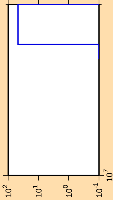
\Delta\sigma/\sigma vs. E for ^{142}\text{Cs} (mt 11)
