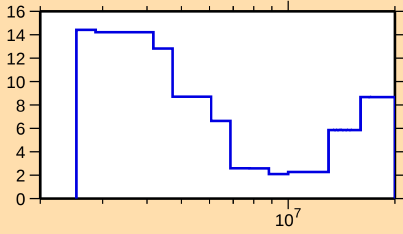
\Delta\sigma/\sigma vs. E for ^{142}\text{Cs}(n,\text{tot.})
