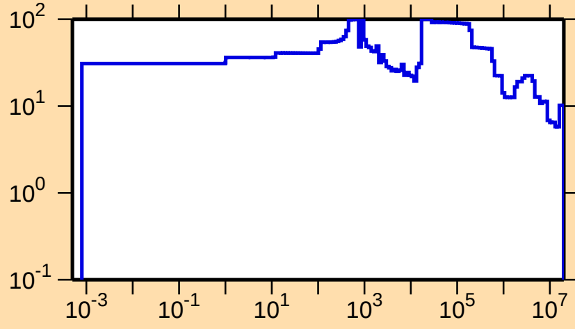
\Delta\sigma/\sigma vs. E for ^{142}\text{Cs}(n,\text{el.})
