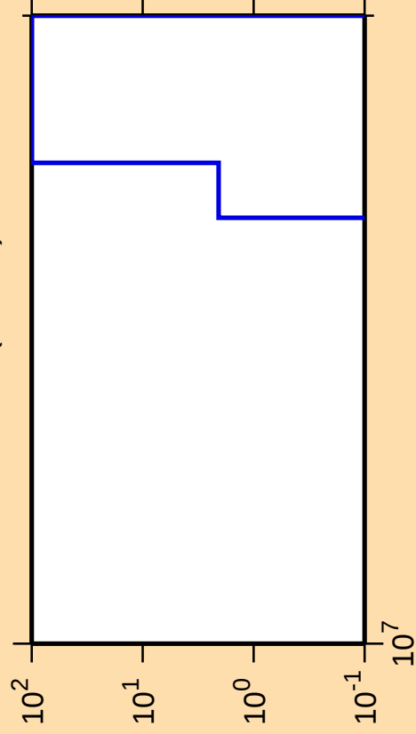
\Delta\sigma/\sigma vs. E for ^{142}\text{Cs}(n,3n\alpha)
