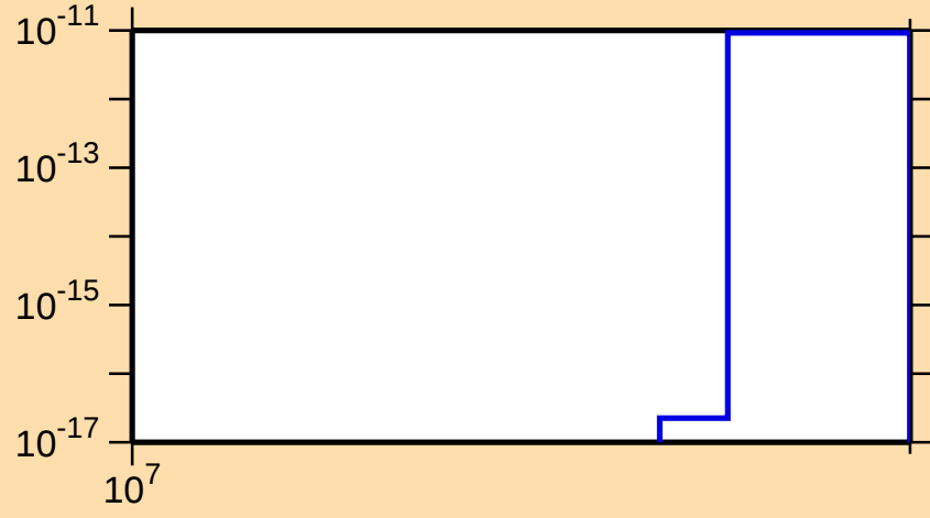
\sigma vs. E for ^{142}\text{Cs} (mt 11)
