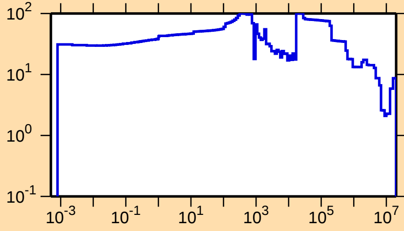
\Delta\sigma/\sigma vs. E for ^{142}\text{Cs}(n,\text{tot.})
