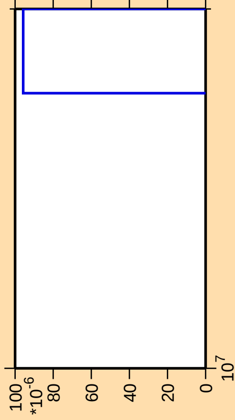
\Delta\sigma/\sigma vs. E for ^{142}\text{Cs} (mt 42)
