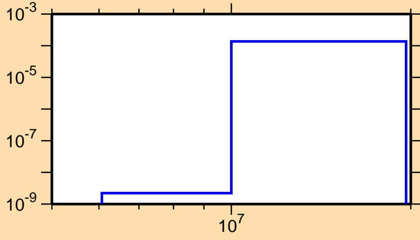
\sigma vs. E for ^{142}\text{Cs}(n,t)
