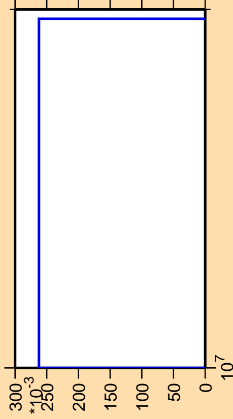
\Delta\sigma/\sigma vs. E for ^{142}\text{Cs} (mt 11)
