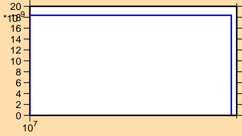
\sigma vs. E for ^{142}\text{Cs}(n,2np)
