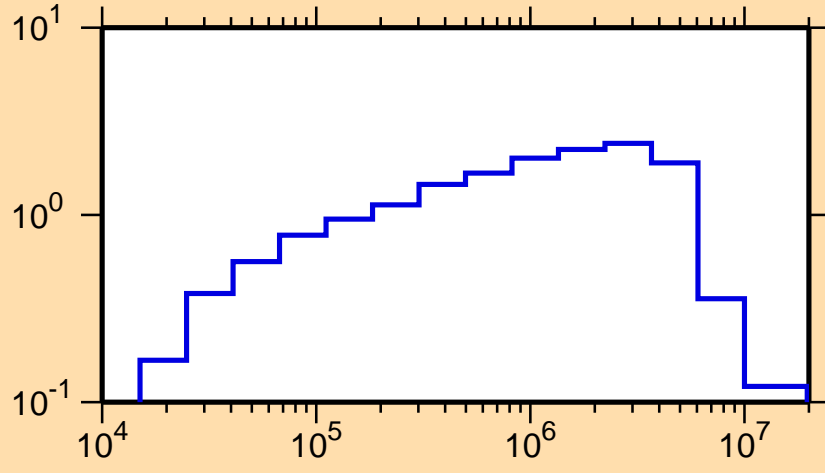
\sigma vs. E for ^{142}\text{Cs}(n,\text{inel.})
