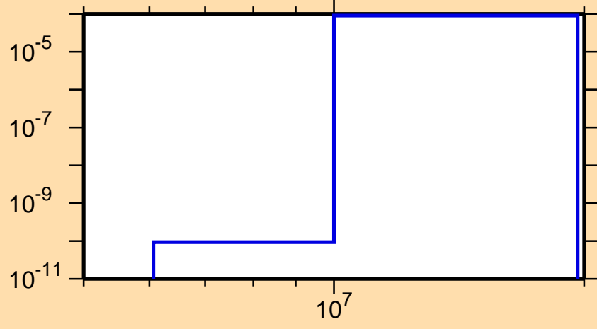
\sigma vs. E for ^{142}\text{Cs}(n,n\alpha)
