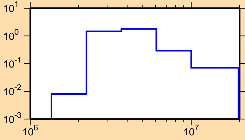
\sigma vs. E for ^{142}\text{Cs}(n,n\text{cont.})
