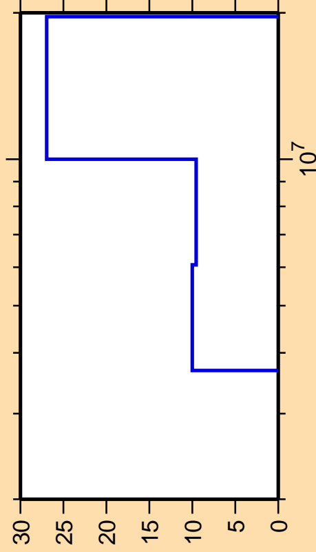
\Delta\sigma/\sigma vs. E for ^{142}\text{Cs}(n,2n)
