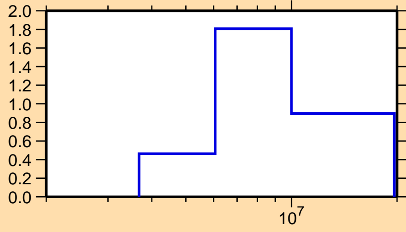
\sigma vs. E for ^{142}\text{Cs}(n,2n)
