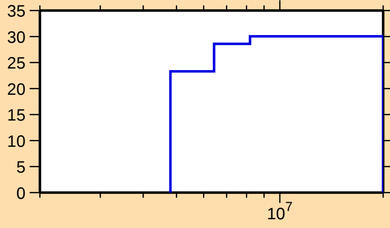
\Delta\sigma/\sigma vs. E for ^{142}\text{Cs}(n,n\text{cont.})
