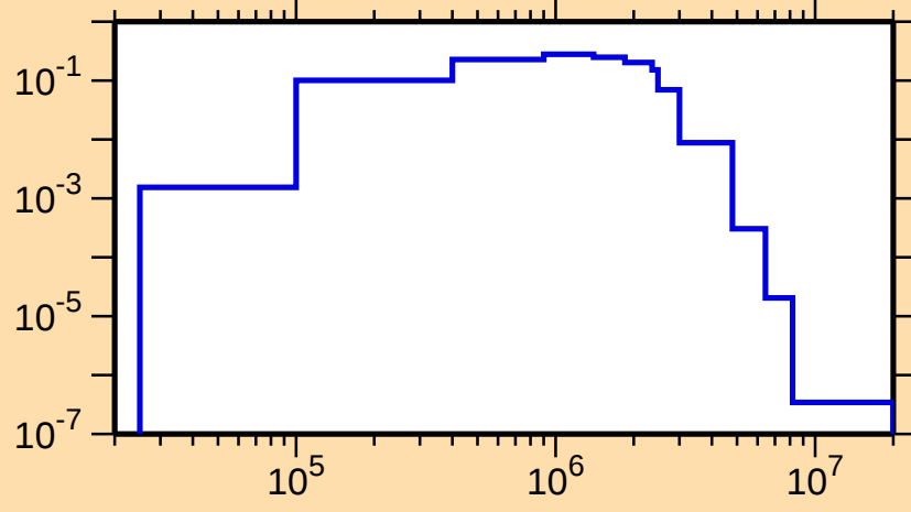
\sigma vs. E for ^{142}\text{Cs}(n,n_4)
