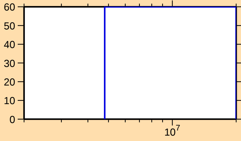
\Delta\sigma/\sigma vs. E for ^{142}\text{Cs}(n,n_1)
