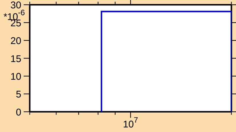
\sigma vs. E for ^{142}\text{Cs}(n,np)
