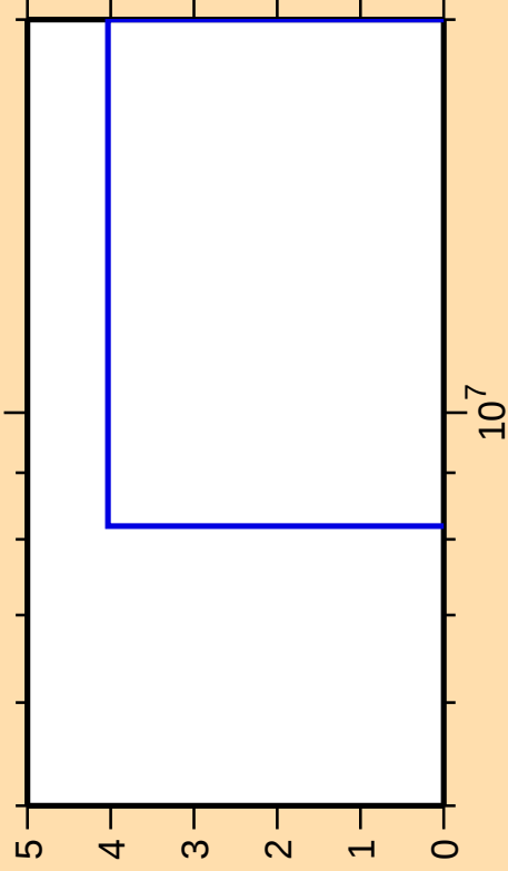
\Delta\sigma/\sigma vs. E for ^{142}\text{Cs}(n,3n\alpha)
