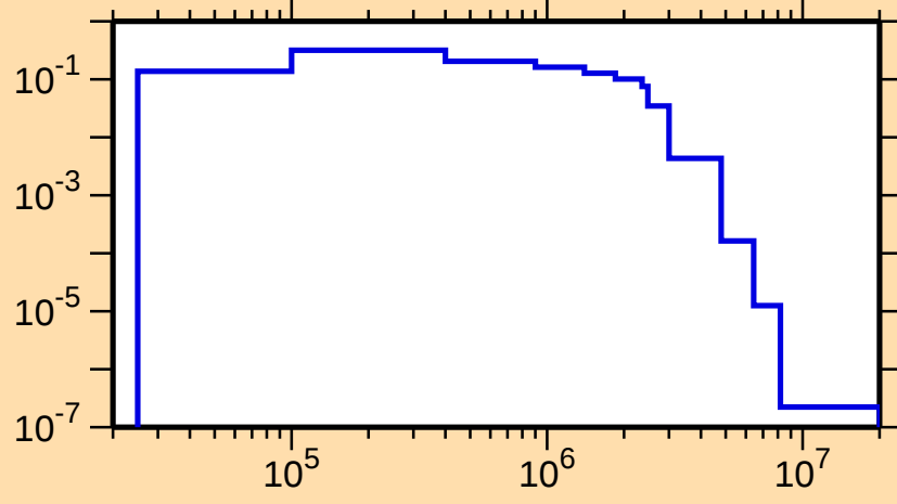
\sigma vs. E for ^{142}\text{Cs}(n,n_2)
