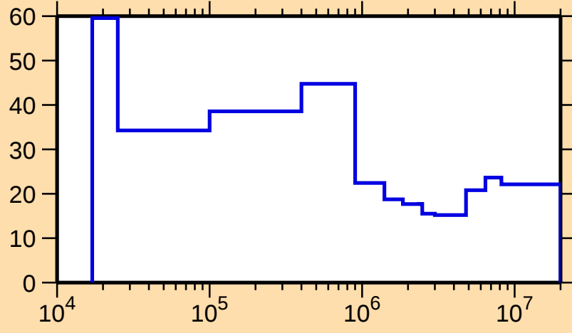
\Delta\sigma/\sigma vs. E for ^{142}\text{Cs}(n,\text{inel.})
