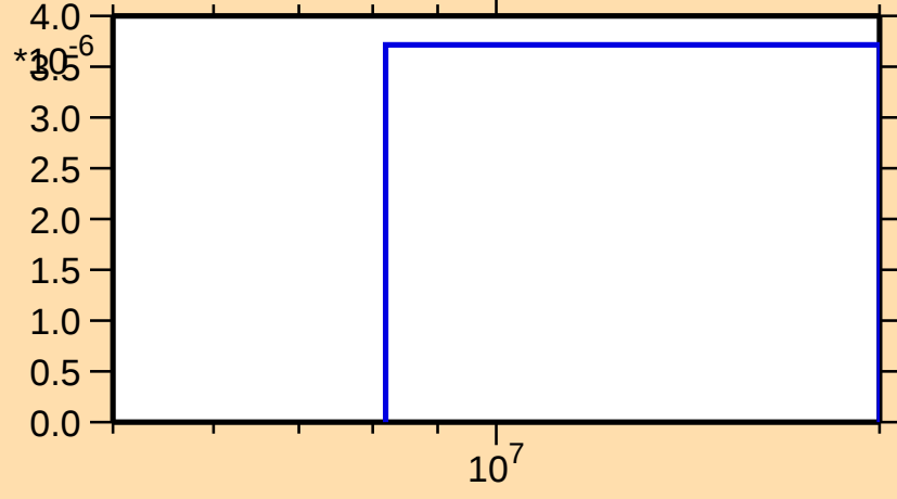
\sigma vs. E for ^{142}\text{Cs}(n,nt)
