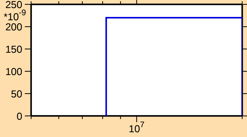
\sigma vs. E for ^{142}\text{Cs}(n,2n\alpha)
