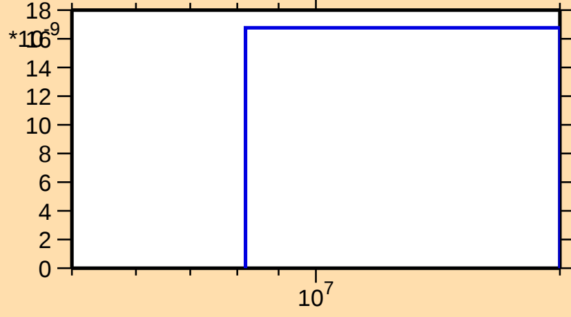
\sigma vs. E for ^{142}\text{Cs}(n,2np)
