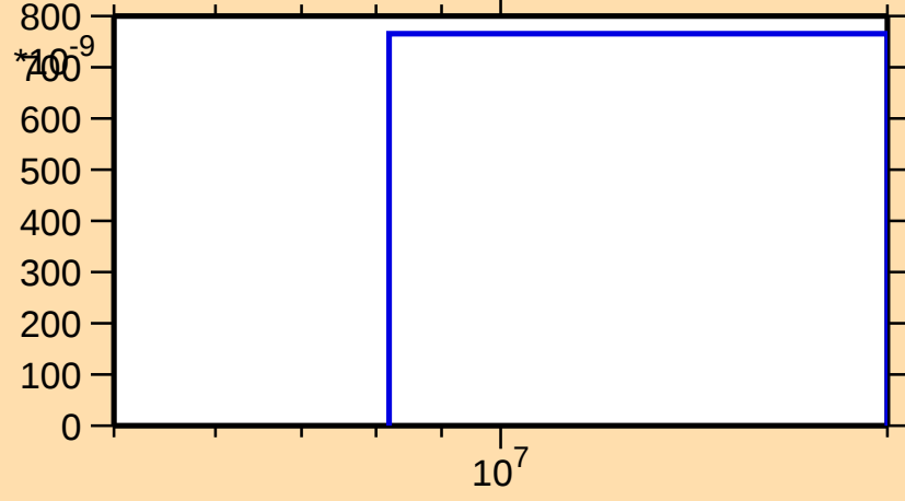
\sigma vs. E for ^{142}\text{Cs}(n,\text{nd})
