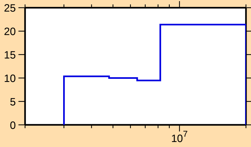
\Delta\sigma/\sigma vs. E for ^{142}\text{Cs}(n,2n)
