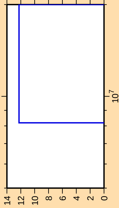
\Delta\sigma/\sigma vs. E for ^{142}\text{Cs}(n,3n)
