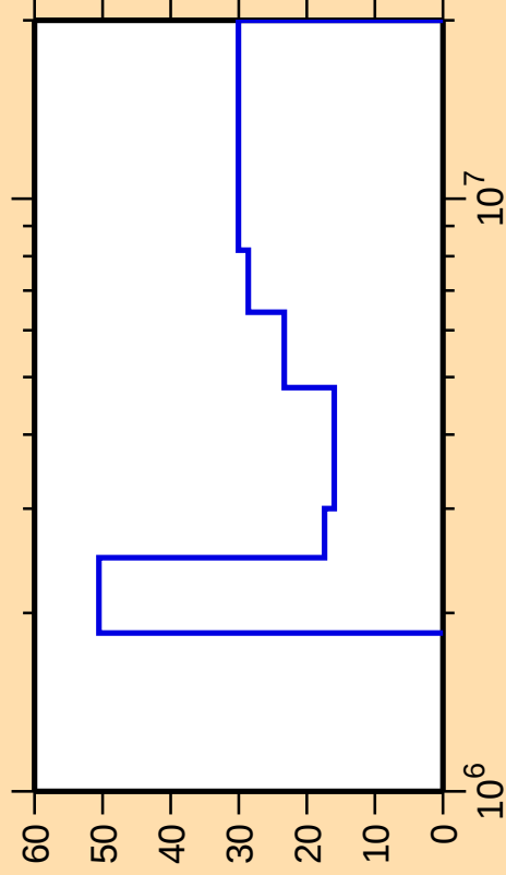
\Delta\sigma/\sigma vs. E for ^{142}\text{Cs}(n,n_{\text{cont}})
