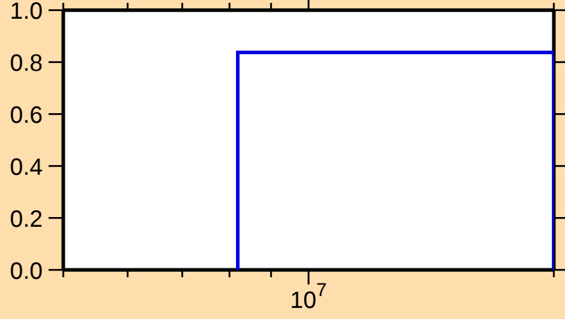
\sigma vs. E for ^{142}\text{Cs}(n,3n)
