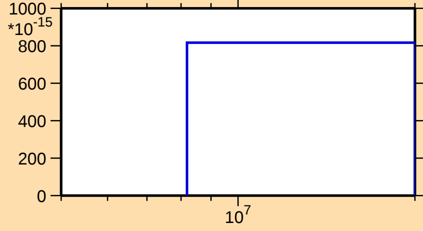
\sigma vs. E for ^{142}\text{Cs}(n,3n\alpha)
