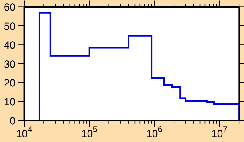
\Delta\sigma/\sigma vs. E for ^{142}\text{Cs}(n,\text{nonel.})
