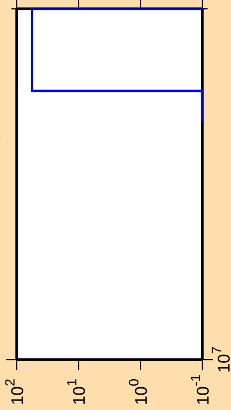
\Delta\sigma/\sigma vs. E for ^{143}\text{Cs} (mt 11)
