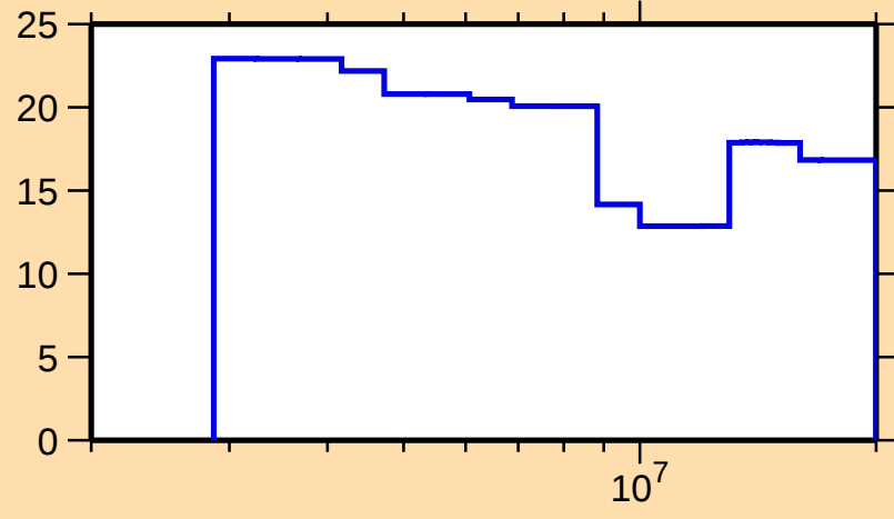
\Delta\sigma/\sigma vs. E for ^{143}\text{Cs}(n,\text{nonel.})
