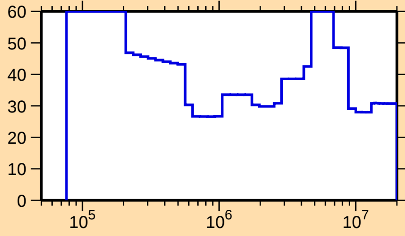
\Delta\sigma/\sigma vs. E for ^{143}\text{Cs}(n,\text{el.})
