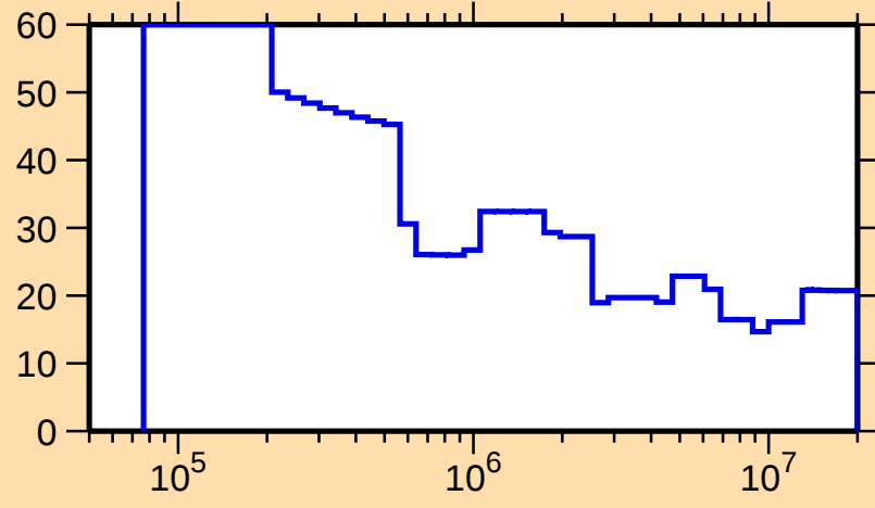
\Delta\sigma/\sigma vs. E for ^{143}\text{Cs}(n,\text{tot.})
