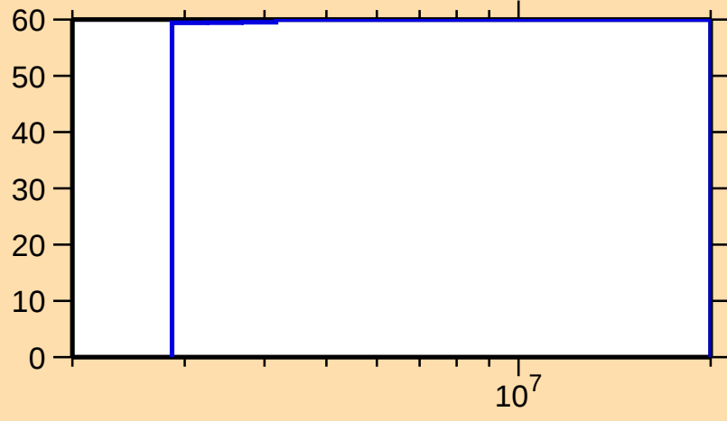
\Delta\sigma/\sigma vs. E for ^{143}\text{Cs}(n,n_1)
