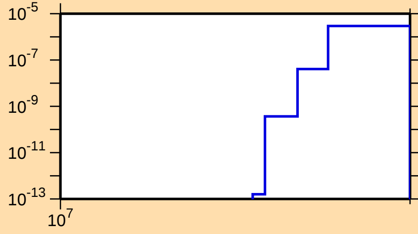
\sigma vs. E for ^{143}\text{Cs}(n,\text{nd})
