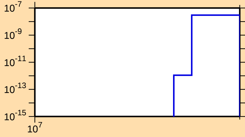
\sigma vs. E for ^{143}\text{Cs}(n,2np)
