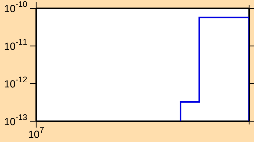
\sigma vs. E for ^{143}\text{Cs}(n,3n\alpha)
