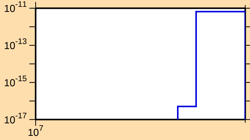
\sigma vs. E for ^{143}\text{Cs} (mt 11)
