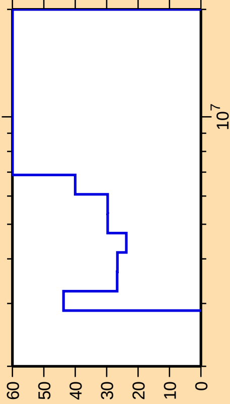
\Delta\sigma/\sigma vs. E for ^{143}\text{Cs}(n,n\text{cont.})
