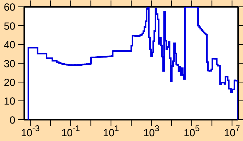
\Delta\sigma/\sigma vs. E for ^{143}\text{Cs}(n,\text{tot.})
