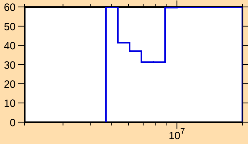
\Delta\sigma/\sigma vs. E for ^{143}\text{Cs}(n,2n)
