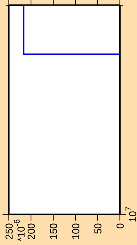
\Delta\sigma/\sigma vs. E for ^{143}\text{Cs} (mt 42)
