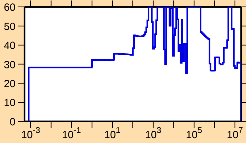
\Delta\sigma/\sigma vs. E for ^{143}\text{Cs}(n,\text{el.})
