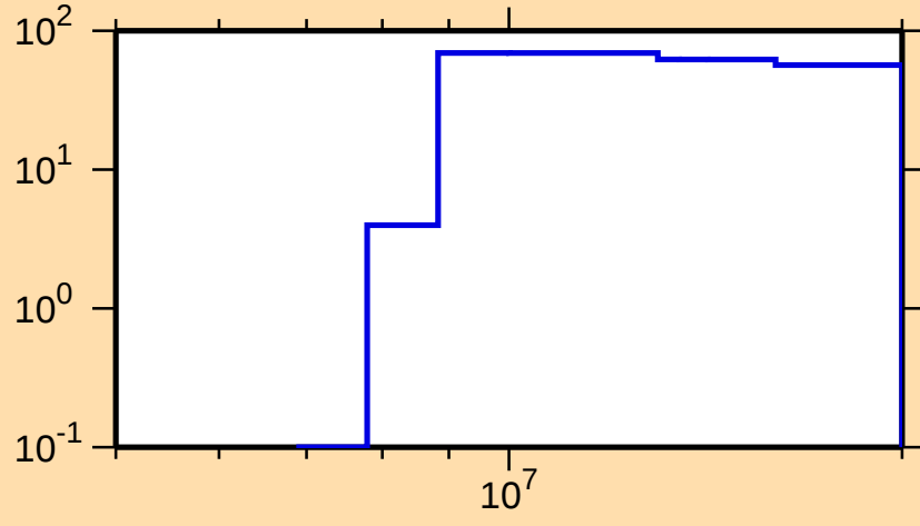
\Delta\sigma/\sigma vs. E for ^{143}\text{Cs}(n,p)
