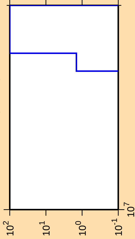
\Delta\sigma/\sigma vs. E for ^{143}\text{Cs}(n,3n\alpha)
