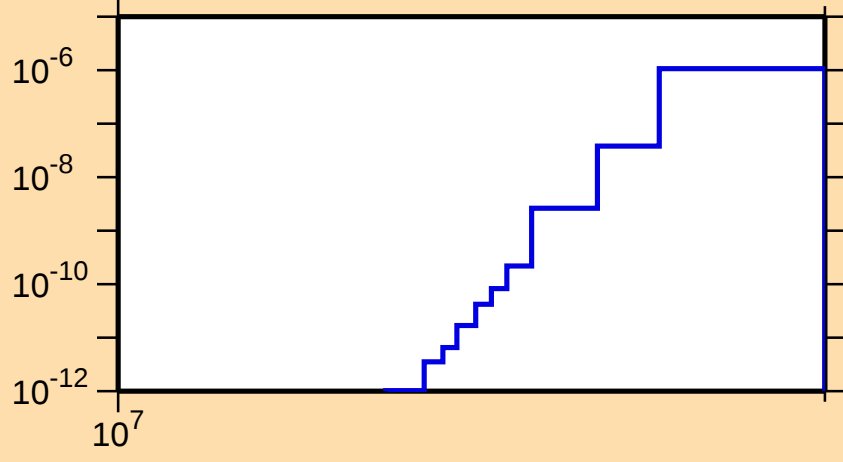
\sigma vs. E for ^{143}\text{Cs}(n,2n\alpha)
