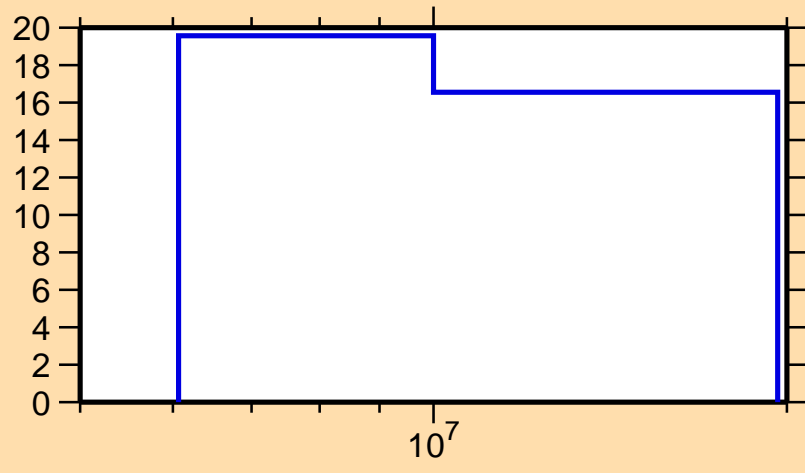
\Delta\sigma/\sigma vs. E for ^{143}\text{Cs}(n,\text{nonel.})
