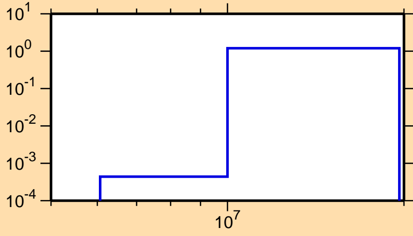
\sigma vs. E for ^{143}\text{Cs}(n,3n)
