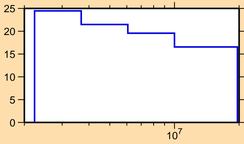
\Delta\sigma/\sigma vs. E for ^{143}\text{Cs}(n,n\text{onel.})
