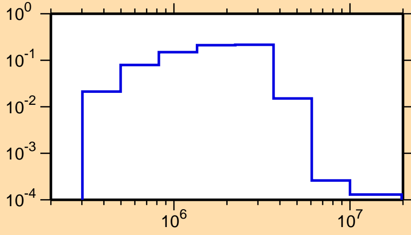
\sigma vs. E for ^{143}\text{Cs}(n,n_3)
