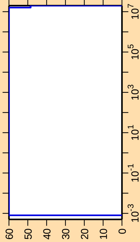
\Delta\sigma/\sigma vs. E for ^{144}\text{Dy}(n,\alpha)
