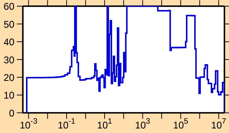
\Delta\sigma/\sigma vs. E for ^{144}\text{Dy}(n,\text{el.})
