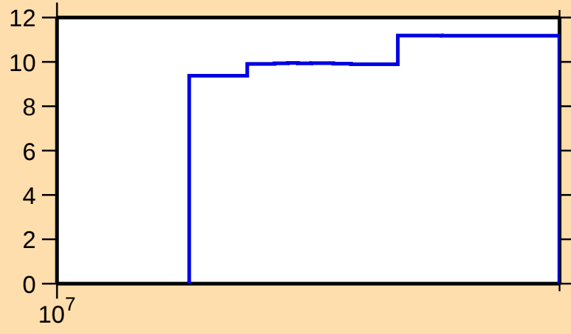
\Delta\sigma/\sigma vs. E for ^{144}\text{Dy}(n,\text{nonel.})
