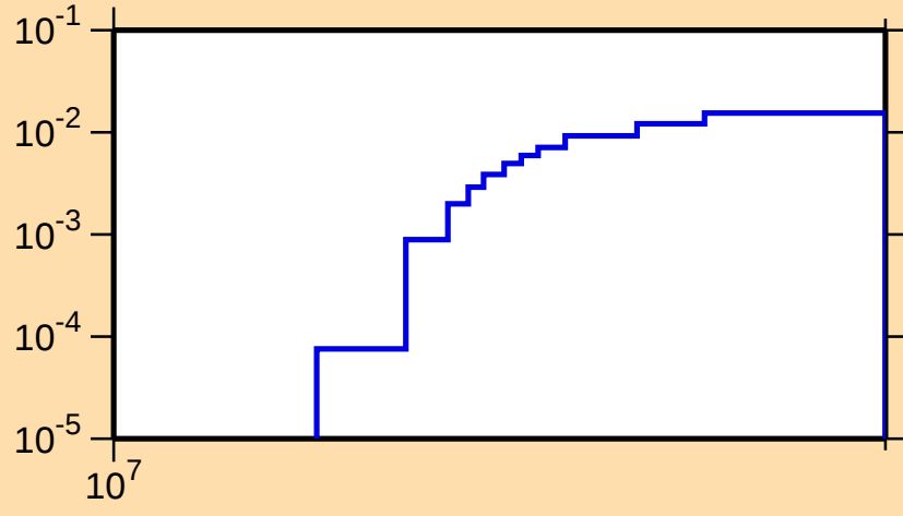
\sigma vs. E for ^{144}\text{Dy}(n,2n)
