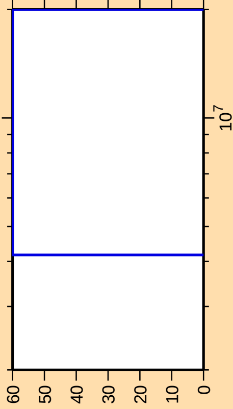
\Delta\sigma/\sigma vs. E for ^{144}\text{Dy}(n,n\text{cont.})
