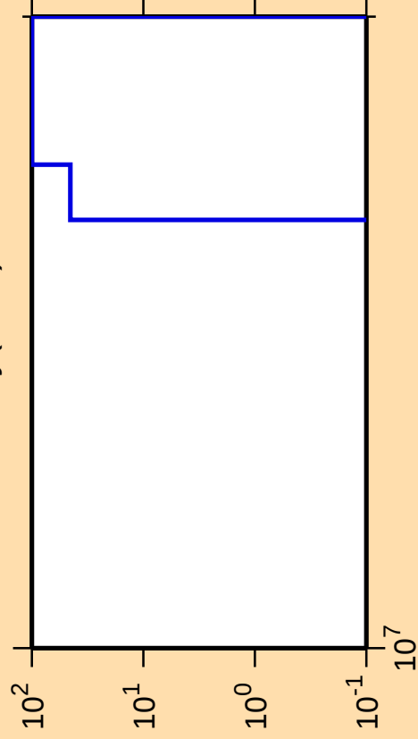
\Delta\sigma/\sigma vs. E for ^{144}\text{Dy}(n,\text{nd})
