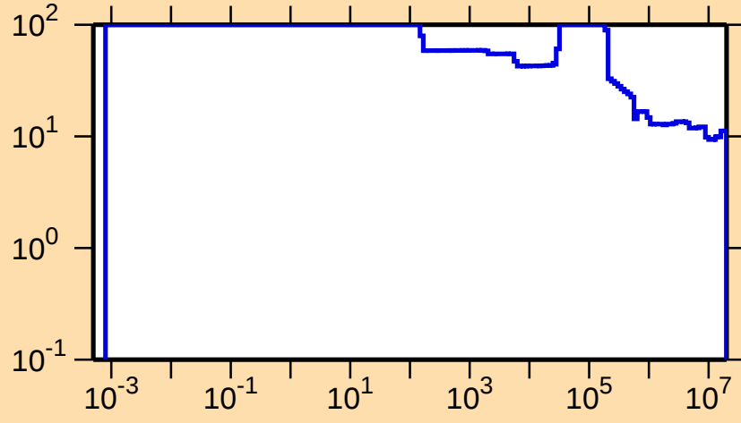
\Delta\sigma/\sigma vs. E for ^{144}\text{Dy}(n,\text{nonel.})
