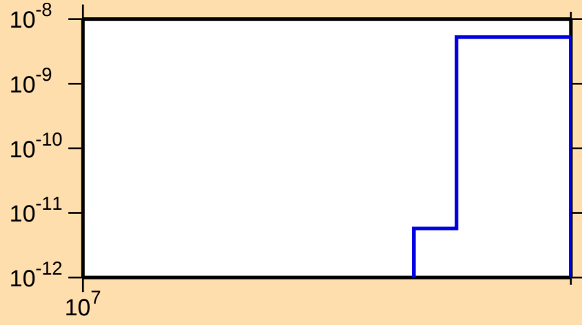
\sigma vs. E for ^{144}\text{Dy}(n,\text{nd})
