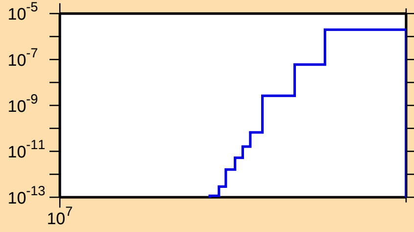
\sigma vs. E for ^{144}\text{Dy}(n,\text{pt})
