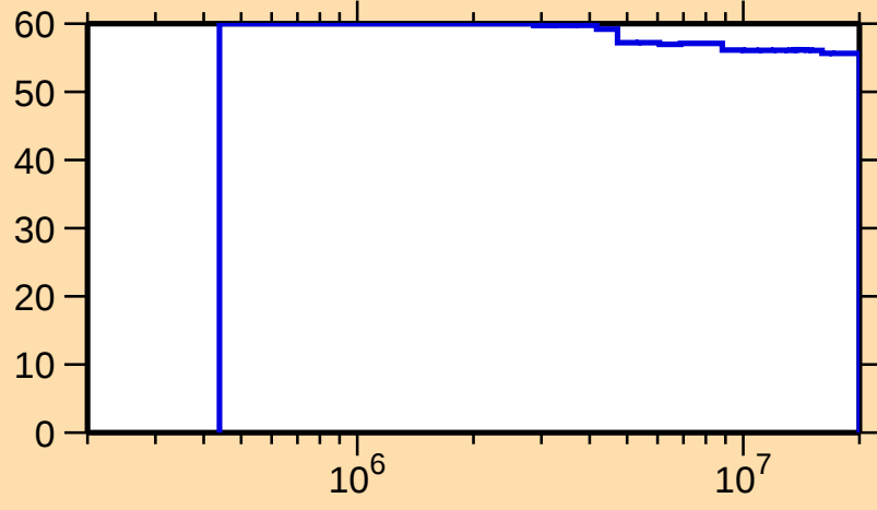
\Delta\sigma/\sigma vs. E for ^{144}\text{Dy}(n,n_1)
