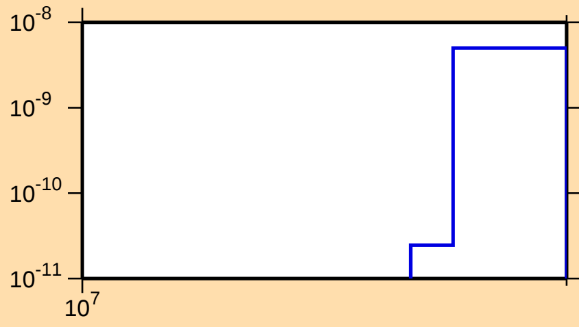
\sigma vs. E for ^{144}\text{Dy}(n,2n\alpha)
