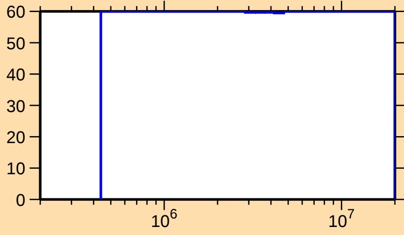
\Delta\sigma/\sigma vs. E for ^{144}\text{Dy}(n,\text{inel.})
