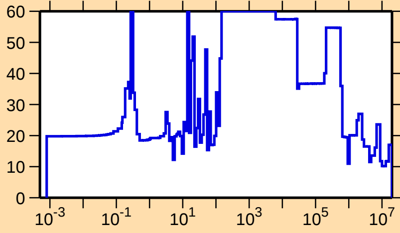
\Delta\sigma/\sigma vs. E for ^{144}\text{Dy}(n,\text{el.})
