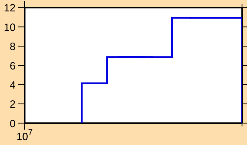
\Delta\sigma/\sigma vs. E for ^{144}\text{Dy}(n,\text{tot.})
