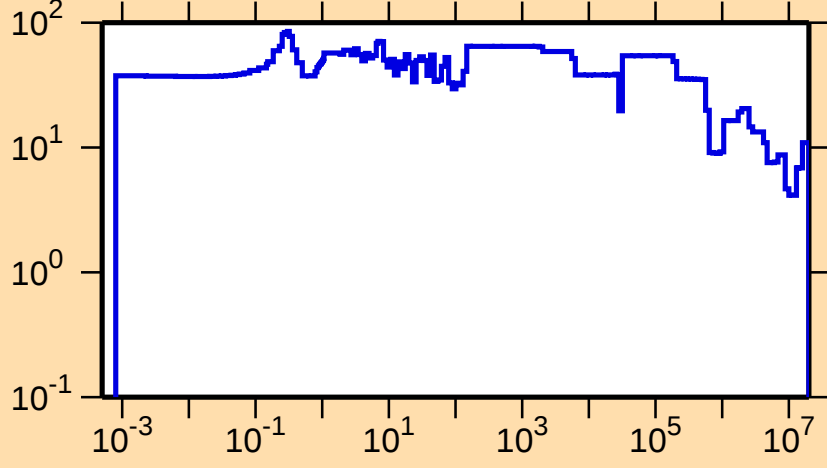
\Delta\sigma/\sigma vs. E for ^{144}\text{Dy}(n,\text{tot.})
