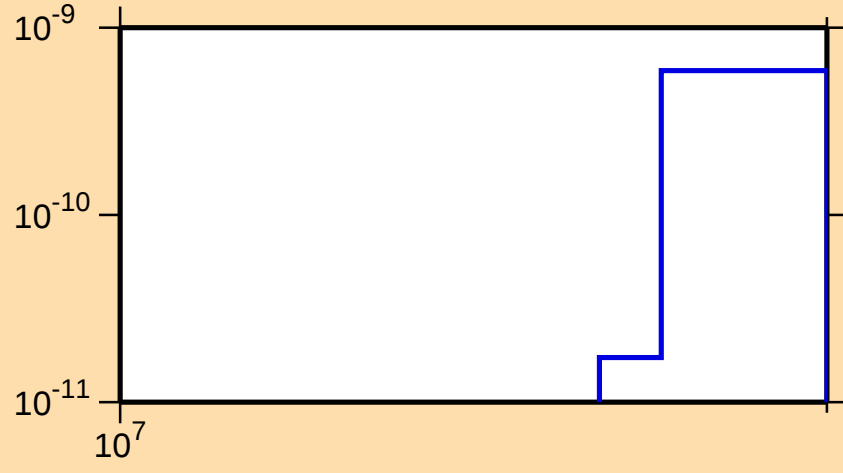
\sigma vs. E for ^{144}\text{Dy} (mt 34)
