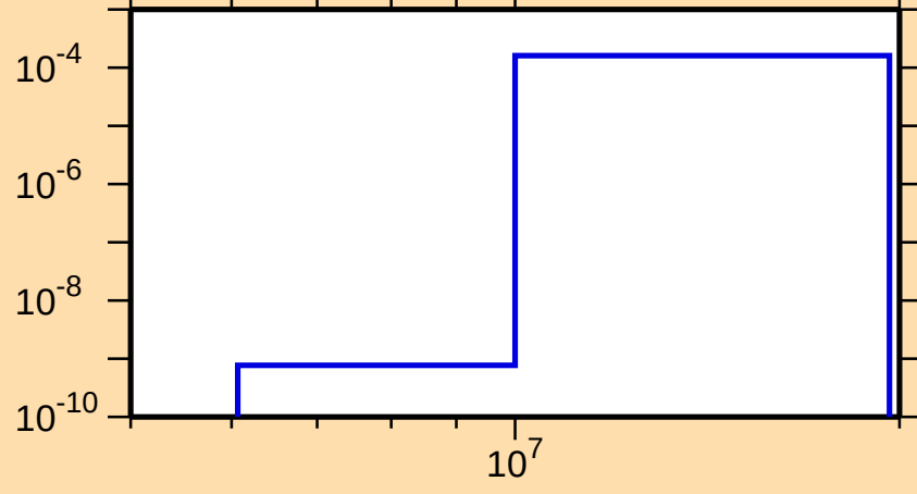
\sigma vs. E for ^{144}\text{Dy}(n,\text{pd})
