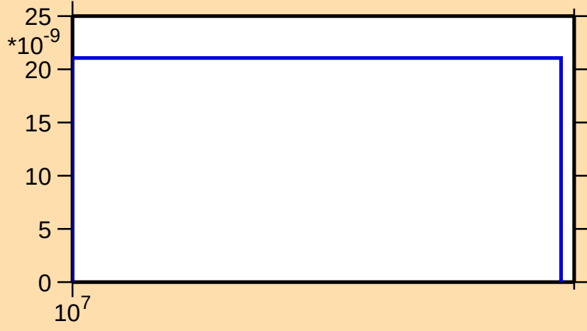
\sigma vs. E for ^{144}\text{Dy}(n,\text{pt})
