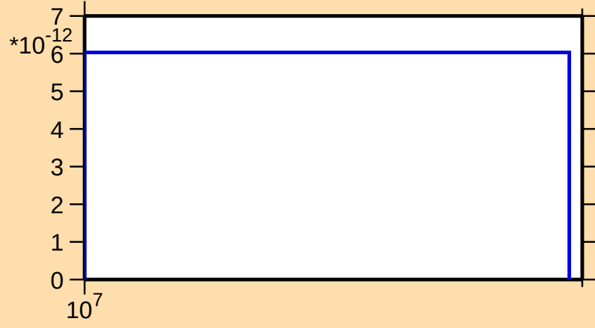
\sigma vs. E for ^{144}\text{Dy} (mt 34)
