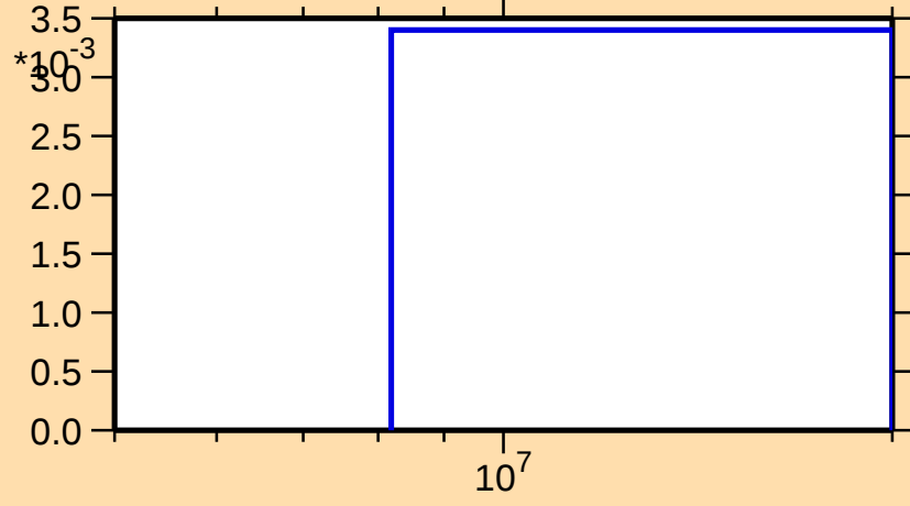
\sigma vs. E for ^{144}\text{Dy}(n,2n)
