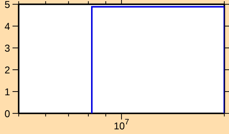
\Delta\sigma/\sigma vs. E for ^{144}\text{Dy}(n,\text{tot.})
