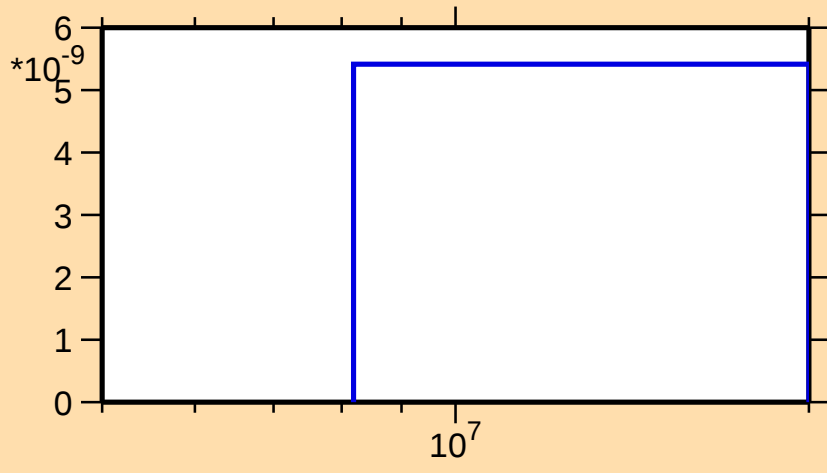
\sigma vs. E for ^{144}\text{Dy}(\text{mt117})
