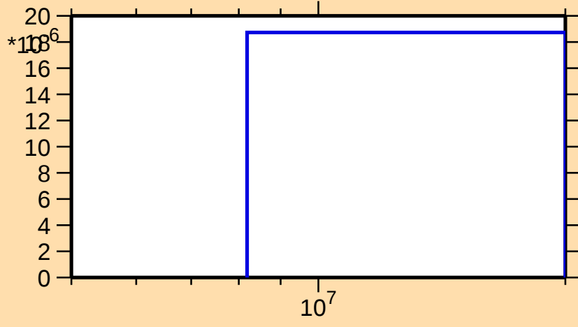
\sigma vs. E for ^{144}\text{Dy}(n,t)
