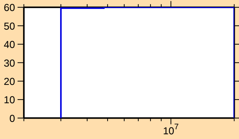
\Delta\sigma/\sigma vs. E for ^{144}\text{Dy}(\text{n},\text{inel.})
