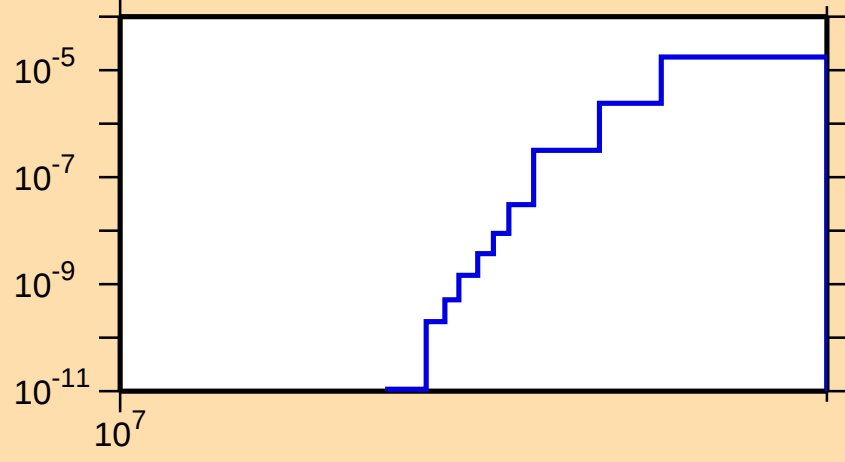
\sigma vs. E for ^{147}\text{Dy}(n,\text{nd})
