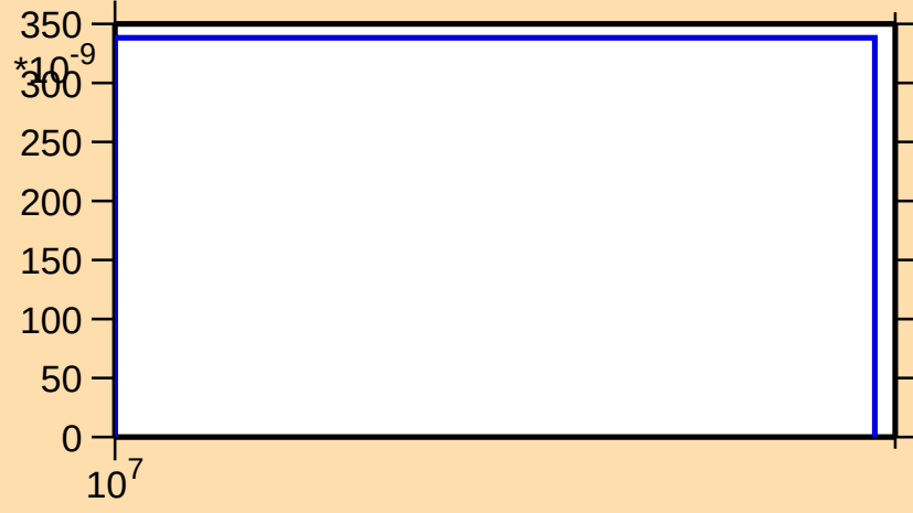
\sigma vs. E for ^{147}\text{Dy}(n,\text{nd})
