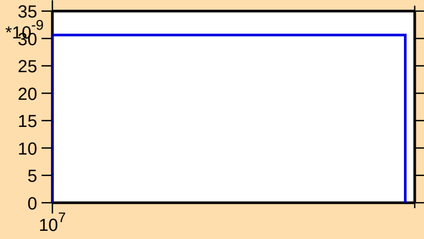
\sigma vs. E for ^{147}\text{Dy}(n,\text{pt})
