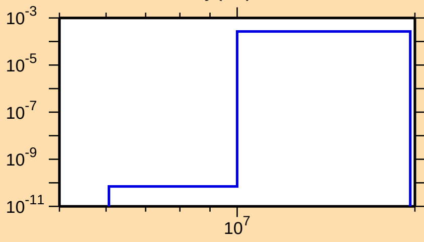
\sigma vs. E for ^{147}\text{Dy}(n,t)
