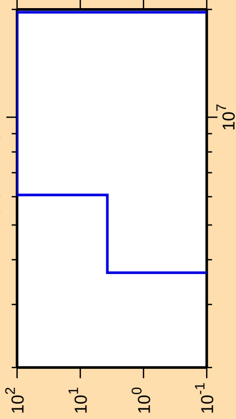
\Delta\sigma/\sigma vs. E for ^{147}\text{Dy}(n,\text{He}3)
