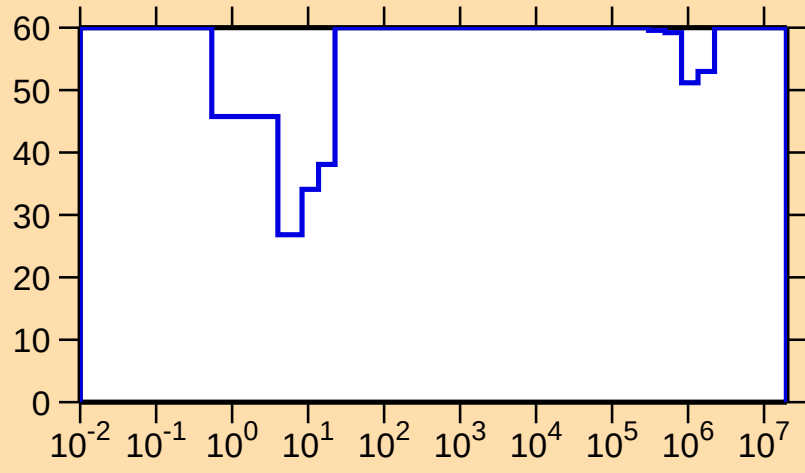
\Delta\sigma/\sigma vs. E for ^{147}\text{Dy}(n,\gamma)
