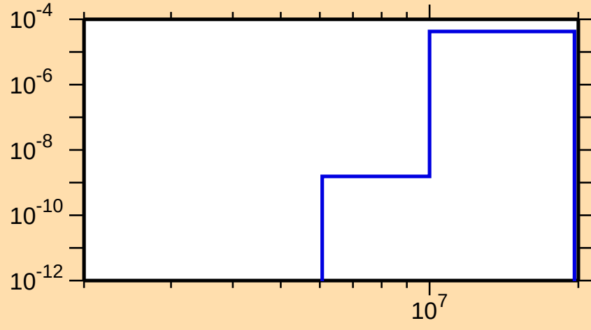
\sigma vs. E for ^{147}\text{Dy}(n,\text{He}3)
