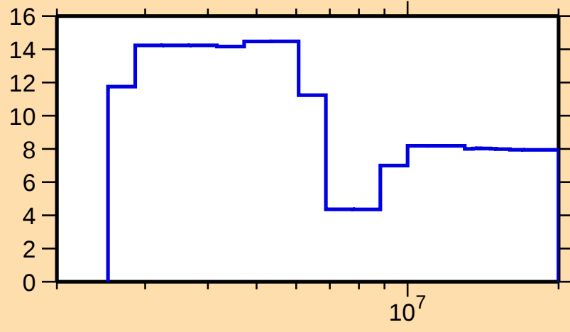
\Delta\sigma/\sigma vs. E for ^{149}\text{Dy}(n,\text{el.})
