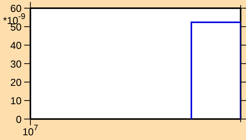
\sigma vs. E for ^{149}\text{Dy}(n,3n)
