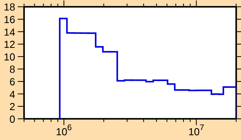
\Delta\sigma/\sigma vs. E for ^{149}\text{Dy}(n,\text{nonel.})
