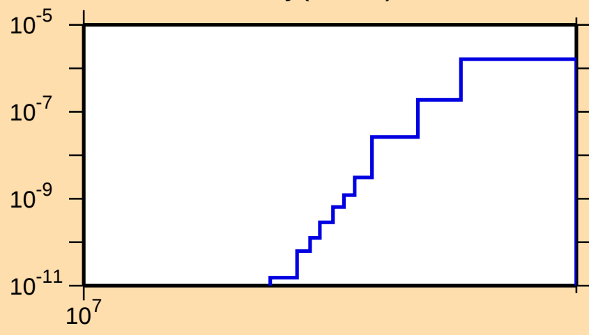
\sigma vs. E for ^{149}\text{Dy}(n,2n\alpha)
