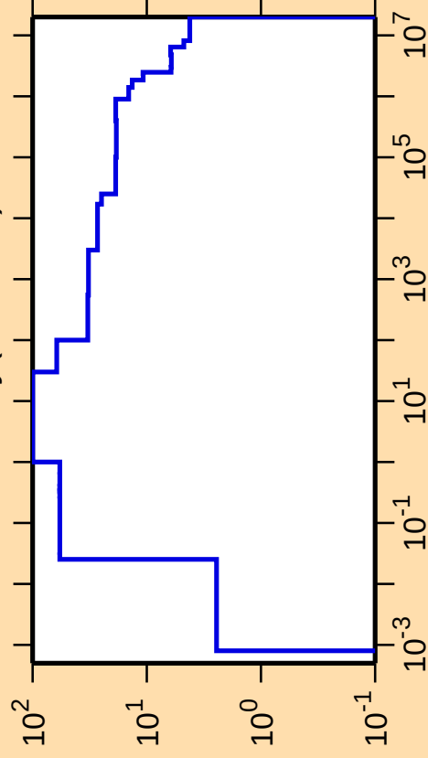
\Delta\sigma/\sigma vs. E for ^{149}\text{Dy}(n,\text{nonel.})
