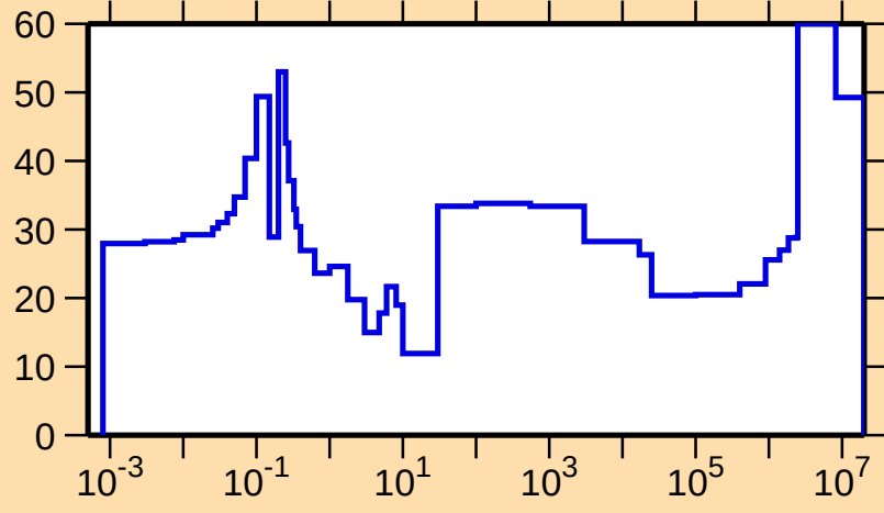
\Delta\sigma/\sigma vs. E for ^{149}\text{Dy}(n,\gamma)
