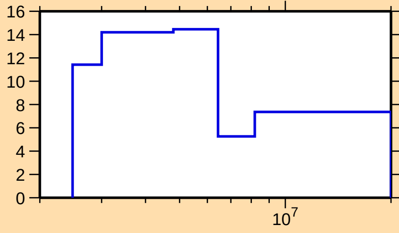
\Delta\sigma/\sigma vs. E for ^{149}\text{Dy}(\text{n},\text{el.})
