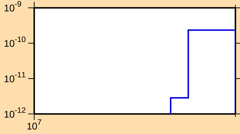
\sigma vs. E for ^{150}\text{Dy} (mt 34)
