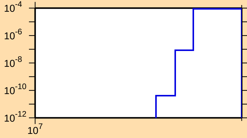
\sigma vs. E for ^{150}\text{Dy}(n,2np)
