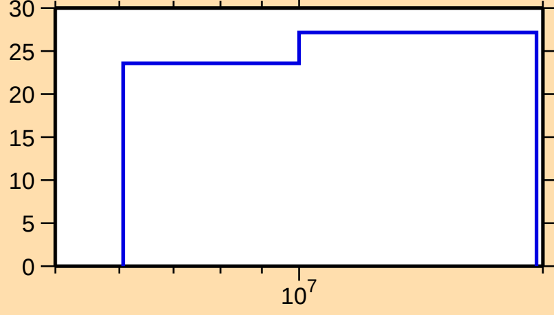
\Delta\sigma/\sigma vs. E for ^{150}\text{Dy}(n,\text{inel.})
