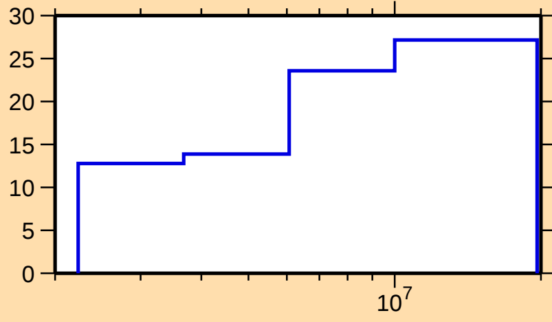
\Delta\sigma/\sigma vs. E for ^{150}\text{Dy}(n,\text{inel.})
