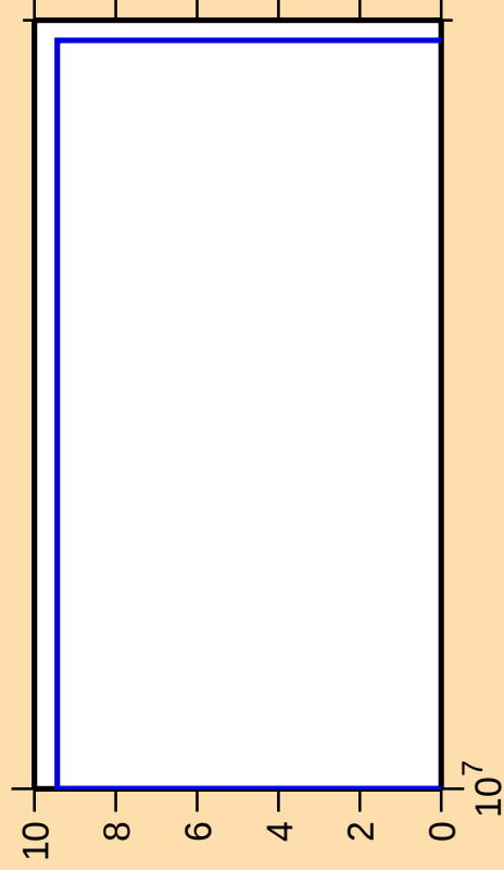
\Delta\sigma/\sigma vs. E for ^{150}\text{Dy} (mt 34)
