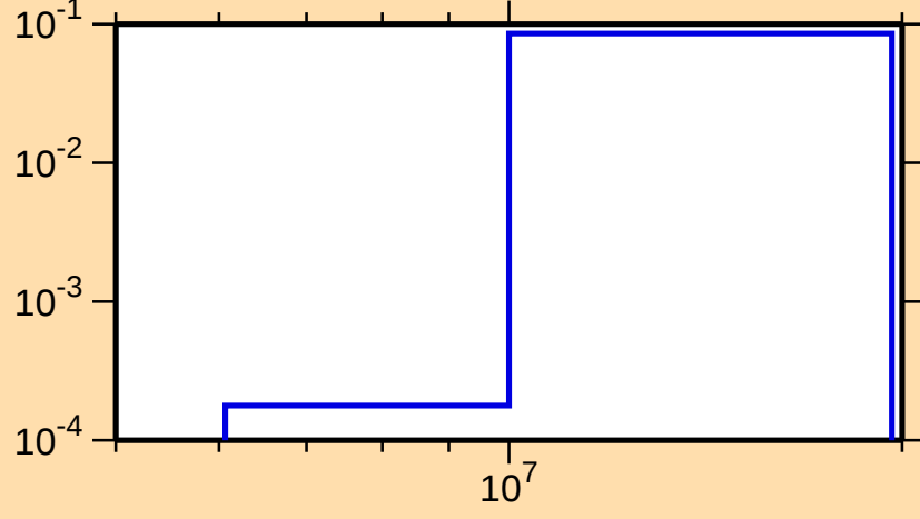
\sigma vs. E for ^{150}\text{Dy}(n,np)
