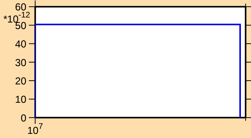
\sigma vs. E for ^{150}\text{Dy}(n,nt)
