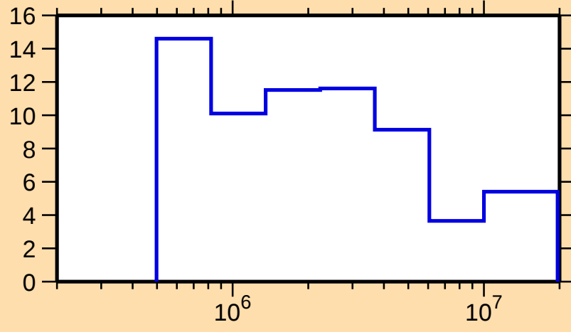
\Delta\sigma/\sigma vs. E for ^{150}\text{Dy}(n,\text{tot.})
