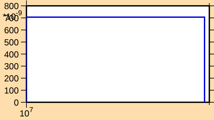
\sigma vs. E for ^{150}\text{Dy}(n,2np)
