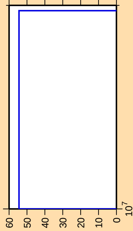
\Delta\sigma/\sigma vs. E for ^{150}\text{Dy}(n,\text{nd})
