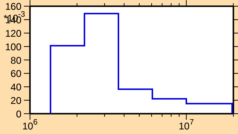
\sigma vs. E for ^{150}\text{Dy}(n,n_3)
