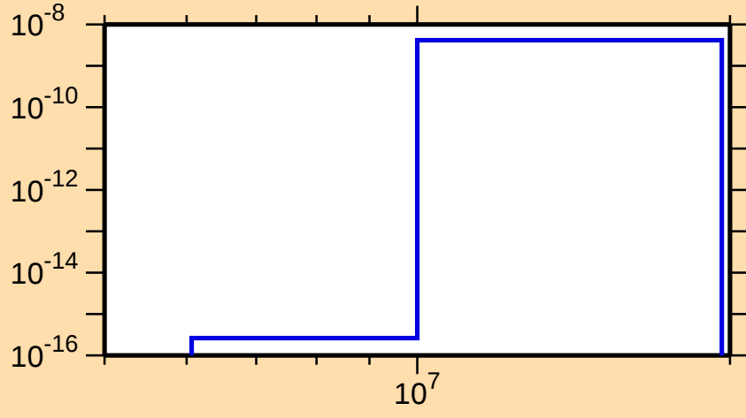
\sigma vs. E for ^{150}\text{Dy}(\text{mt117})
