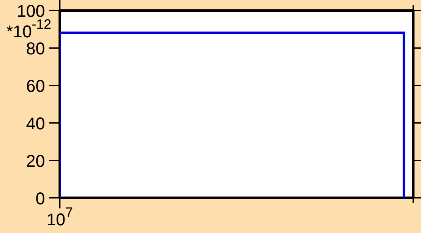
\sigma vs. E for ^{150}\text{Dy}(n,\text{pt})
