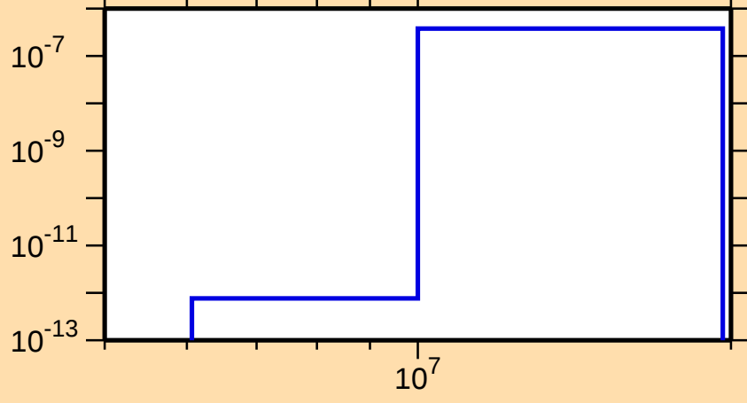
\sigma vs. E for ^{150}\text{Dy}(n,\text{He}3)
