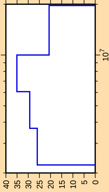
\Delta\sigma/\sigma vs. E for ^{150}\text{Dy}(n,n\text{cont.})
