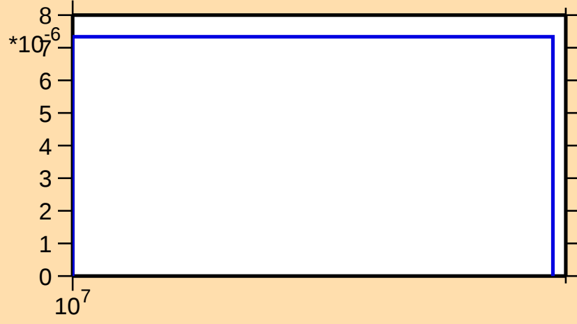
\sigma vs. E for ^{150}\text{Dy}(n,3n)
