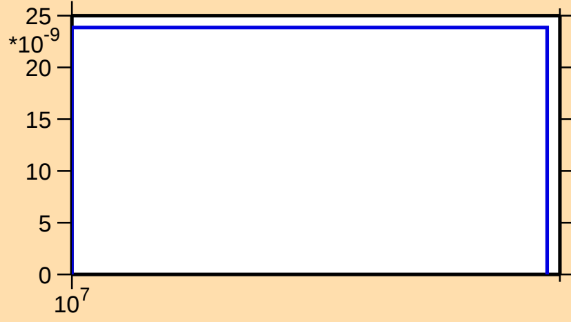
\sigma vs. E for ^{150}\text{Dy}(n,\text{nd})
