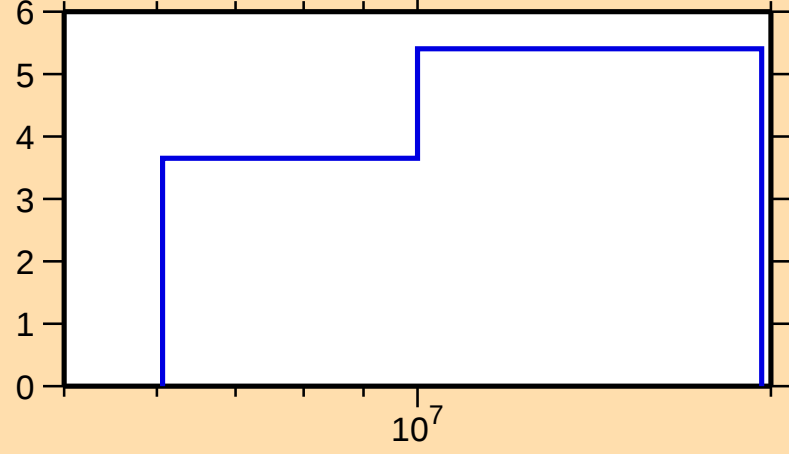
\Delta\sigma/\sigma vs. E for ^{150}\text{Dy}(n,\text{tot.})
