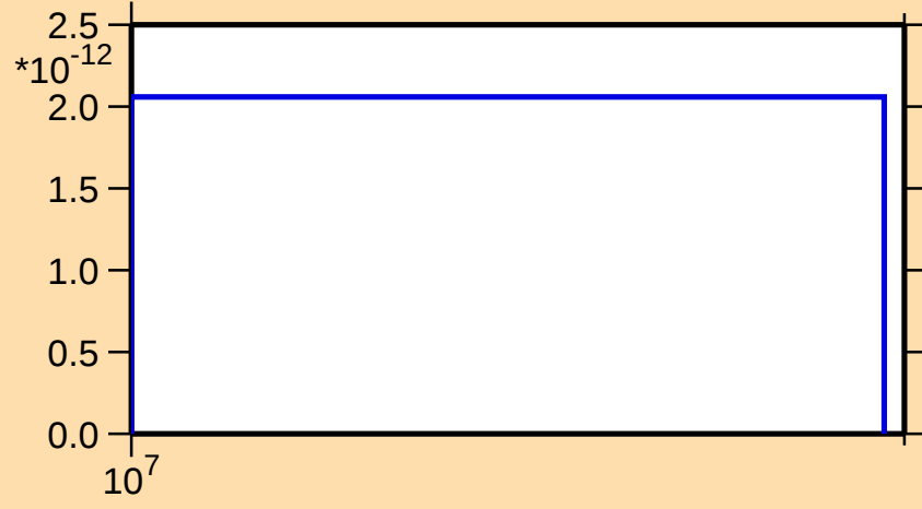
\sigma vs. E for ^{150}\text{Dy} (mt 34)
