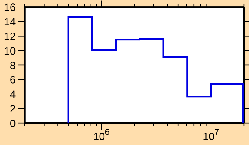
\Delta\sigma/\sigma vs. E for ^{150}\text{Dy}(n,\text{tot.})
