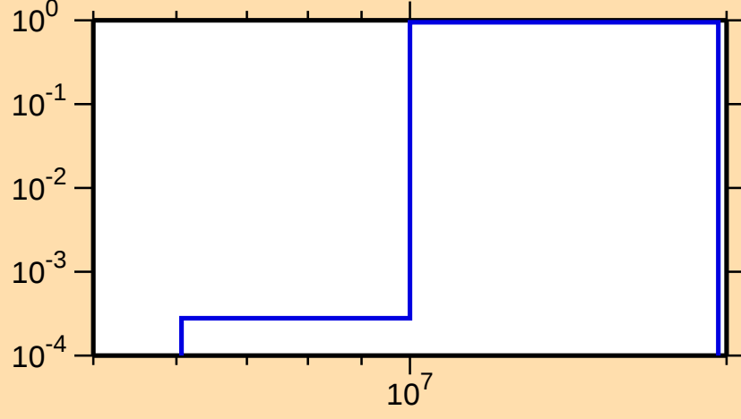
\sigma vs. E for ^{150}\text{Dy}(n,2n)
