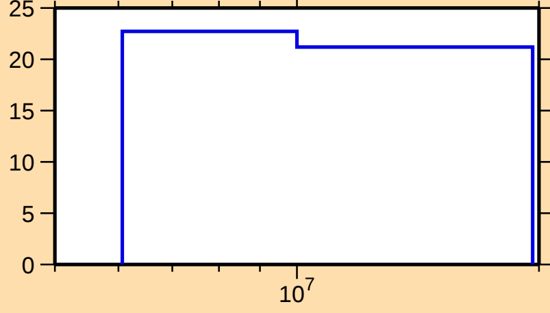
\Delta\sigma/\sigma vs. E for ^{150}\text{Dy}(n,\text{nonel.})
