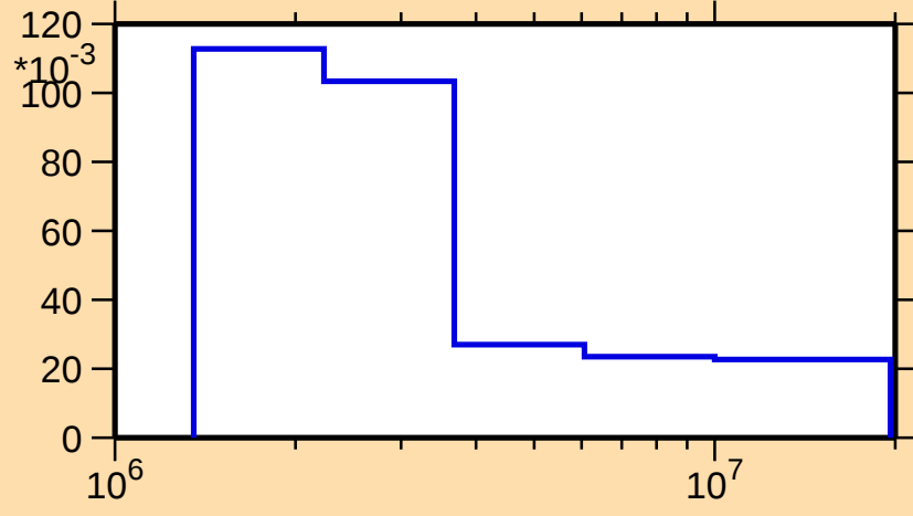
\sigma vs. E for ^{150}\text{Dy}(n,n_2)
