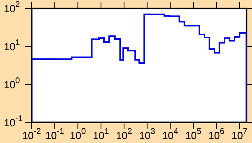
\Delta\sigma/\sigma vs. E for ^{150}\text{Dy}(n,\text{el.})
