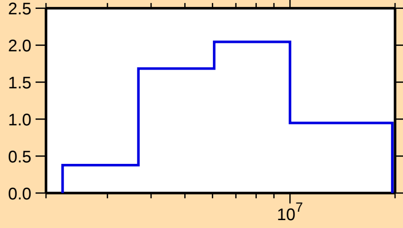
\sigma vs. E for ^{150}\text{Dy}(n,n\text{cont.})
