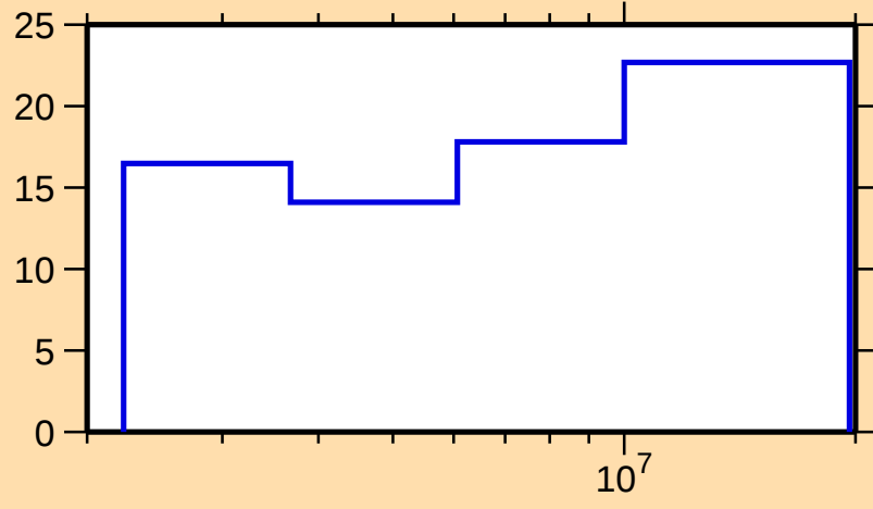
\Delta\sigma/\sigma vs. E for ^{150}\text{Dy}(n,\text{el.})
