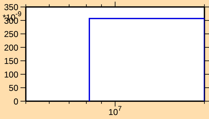
\sigma vs. E for ^{150}\text{Dy}(n,\text{He}3)
