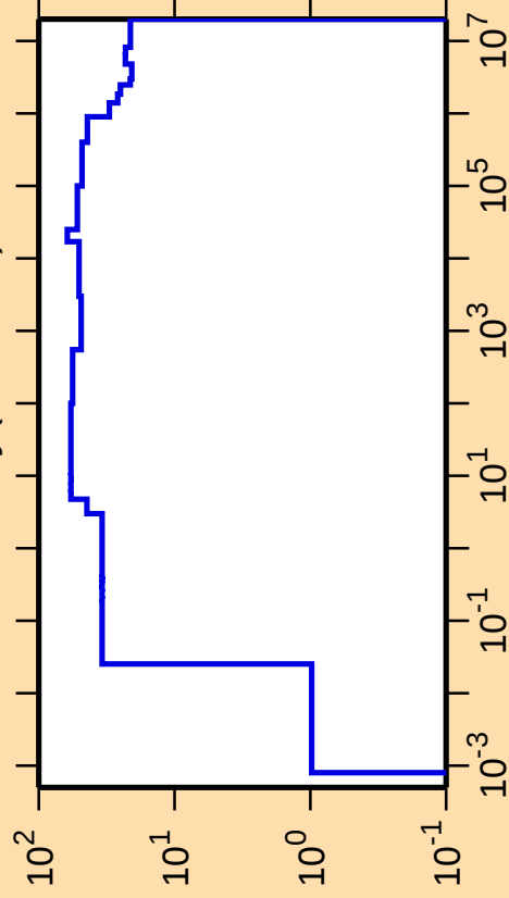
\Delta\sigma/\sigma vs. E for ^{150}\text{Dy}(n,\text{nonel.})
