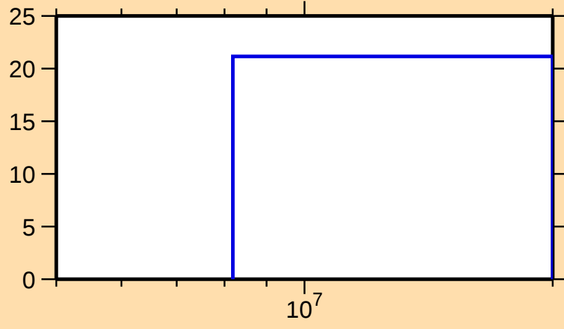
\Delta\sigma/\sigma vs. E for ^{150}\text{Dy}(n,\text{nonel.})
