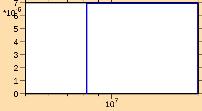
\sigma vs. E for ^{150}\text{Dy}(n,3n)
