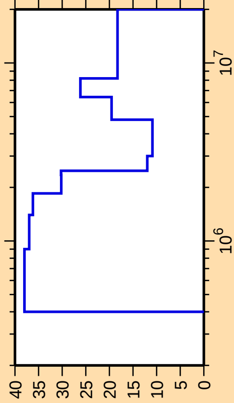
\Delta\sigma/\sigma vs. E for ^{150}\text{Dy}(n,\text{inel.})
