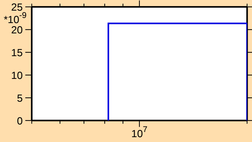
\sigma vs. E for ^{150}\text{Dy}(n,nd)
