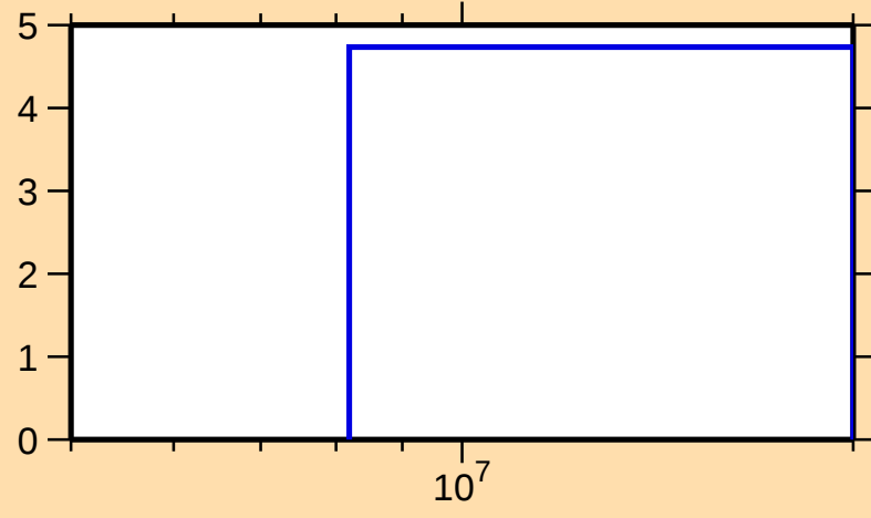
\Delta\sigma/\sigma vs. E for ^{150}\text{Dy}(n,\text{tot.})
