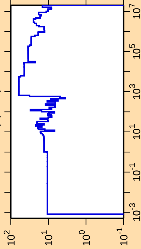
\Delta\sigma/\sigma vs. E for ^{152}\text{Dy}(n,\text{el.})
