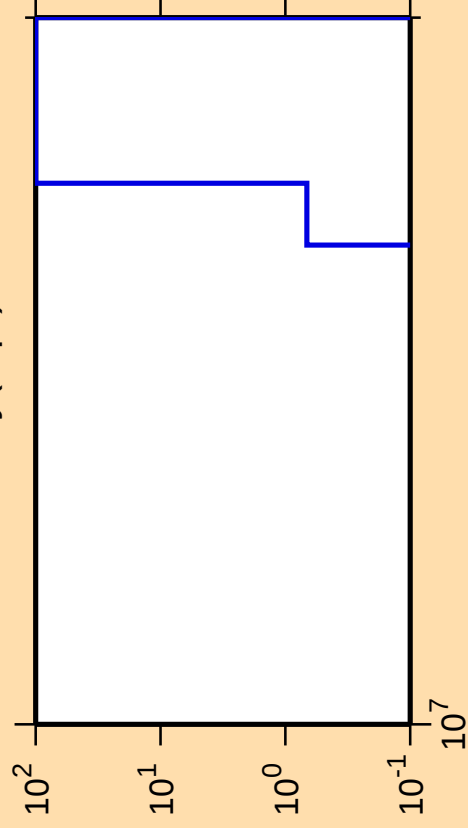
\Delta\sigma/\sigma vs. E for ^{152}\text{Dy}(n,\text{pt})
