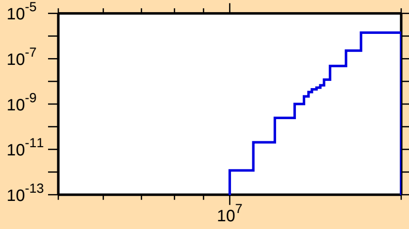
\sigma vs. E for ^{152}\text{Dy}(n,\text{He3})
