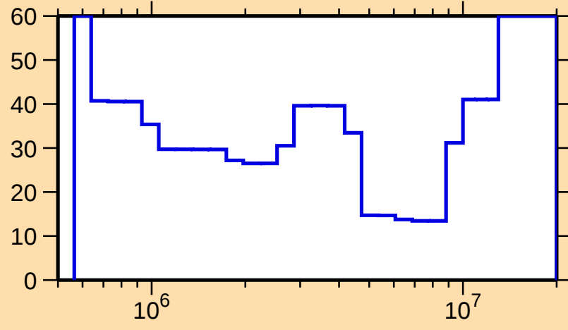
\Delta\sigma/\sigma vs. E for ^{152}\text{Dy}(n,\text{inel.})
