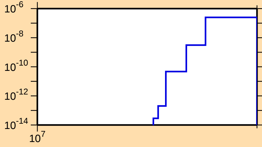
\sigma vs. E for ^{152}\text{Dy}(n,nd)
