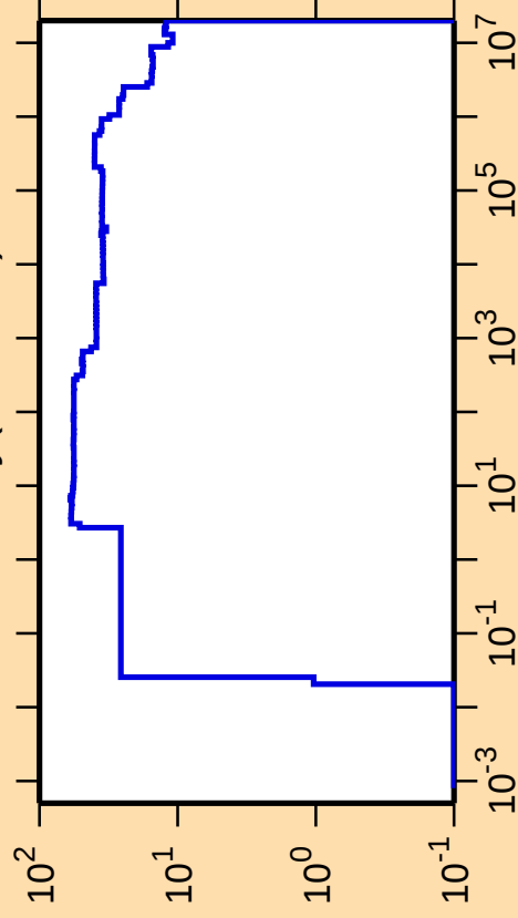
\Delta\sigma/\sigma vs. E for ^{152}\text{Dy}(n,\text{nonel.})
