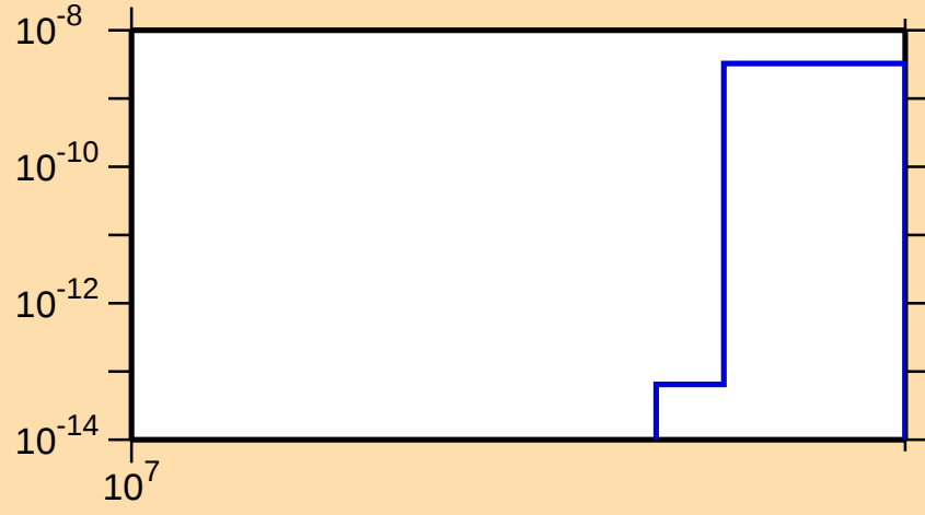
\sigma vs. E for ^{152}\text{Dy}(n,nt)
