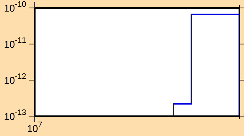
\sigma vs. E for ^{152}\text{Dy}(n,\text{pt})
