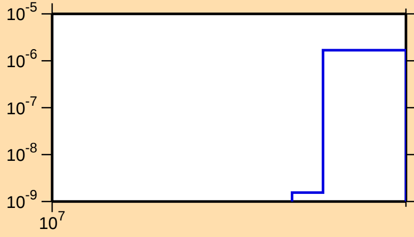
\sigma vs. E for ^{152}\text{Dy}(n,2np)
