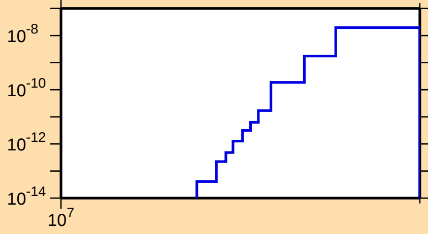
\sigma vs. E for ^{152}\text{Dy}(n,\text{pd})
