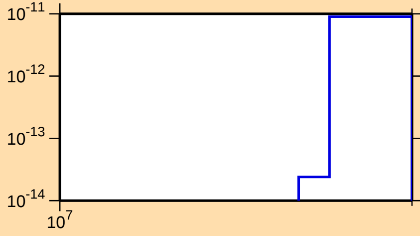
\sigma vs. E for ^{152}\text{Dy} (mt 34)
