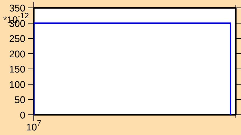
\sigma vs. E for ^{152}\text{Dy}(n,\text{pd})
