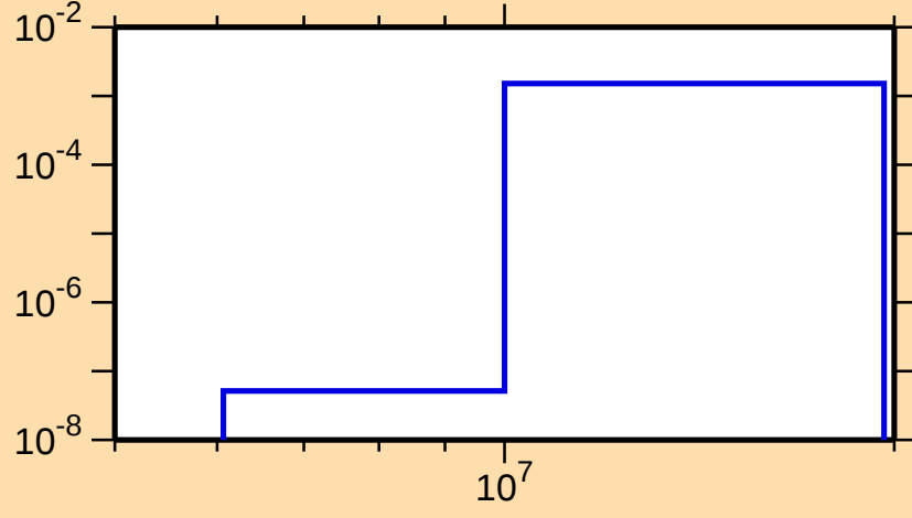
\sigma vs. E for ^{152}\text{Dy}(n,d)
