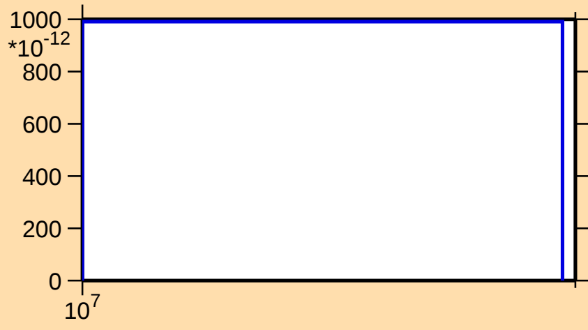
\sigma vs. E for ^{152}\text{Dy} (mt 45)
