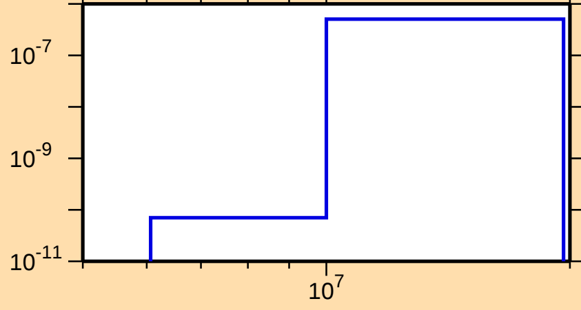
\sigma vs. E for ^{152}\text{Dy}(n,p\alpha)
