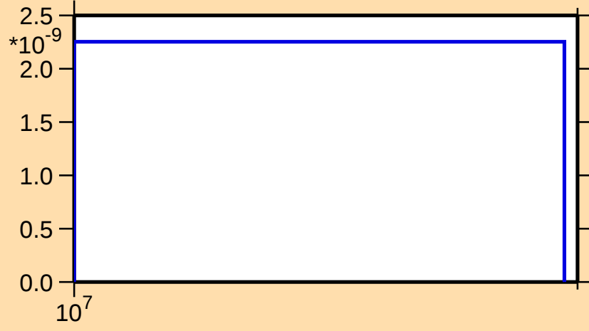
\sigma vs. E for ^{152}\text{Dy}(n,\text{nd})
