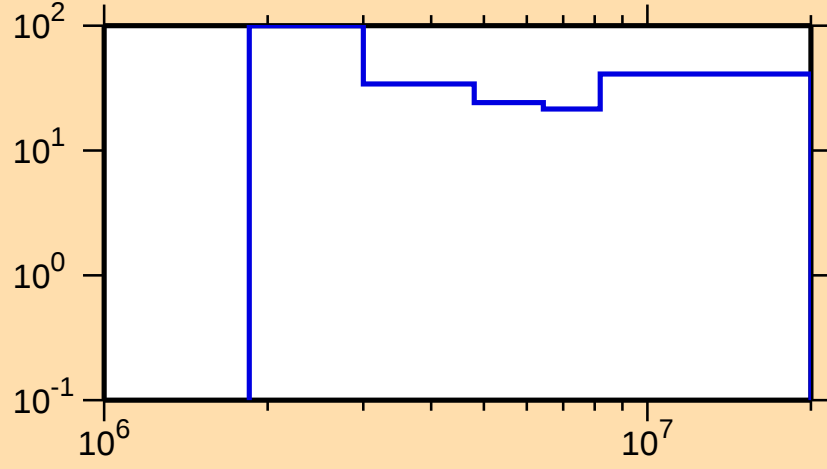
\Delta\sigma/\sigma vs. E for ^{152}\text{Dy}(n,n\text{cont.})
