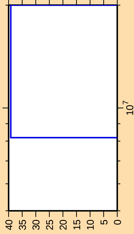
\Delta\sigma/\sigma vs. E for ^{152}\text{Dy}(n,p)
