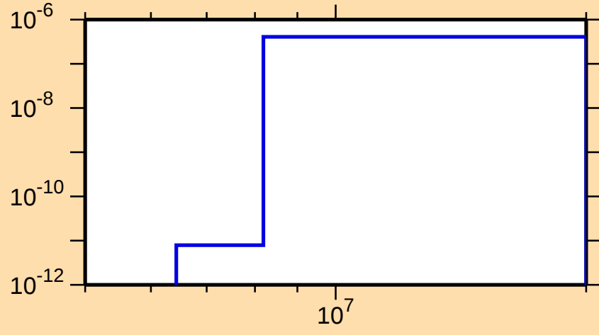
\sigma vs. E for ^{152}\text{Dy}(n,p\alpha)
