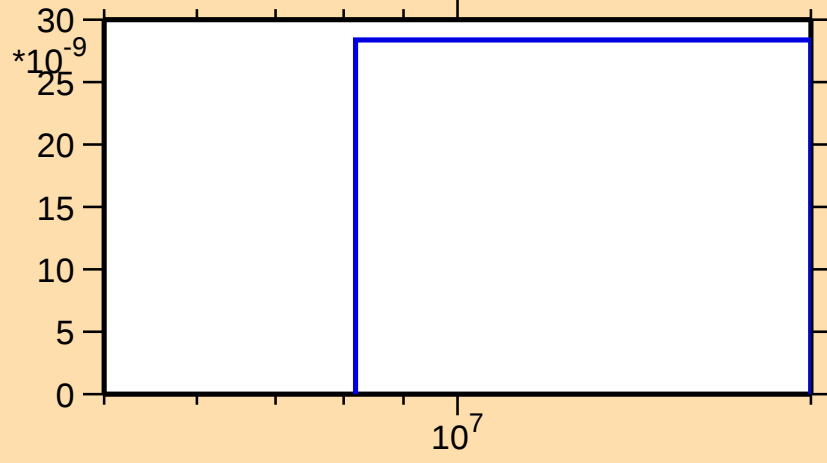
\sigma vs. E for ^{152}\text{Dy}(n,\text{He}3)
