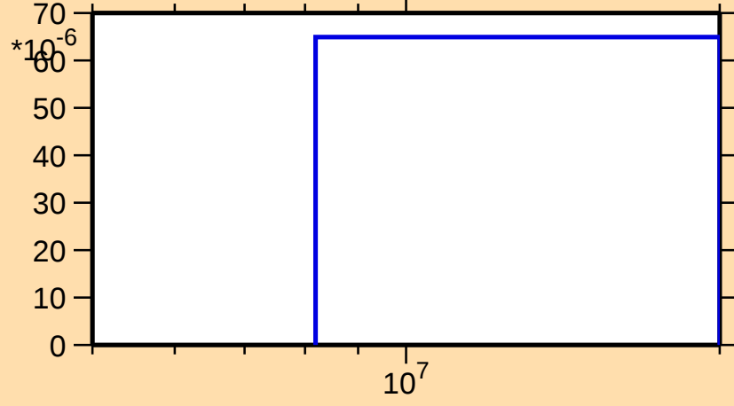
\sigma vs. E for ^{152}\text{Dy}(n,t)
