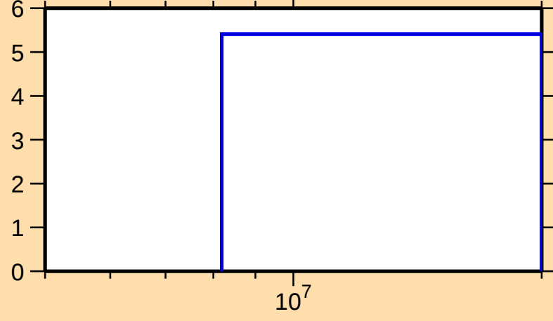
\Delta\sigma/\sigma vs. E for ^{152}\text{Dy}(n,\text{tot.})
