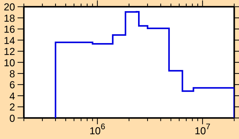
\Delta\sigma/\sigma vs. E for ^{152}\text{Dy}(n,\text{tot.})
