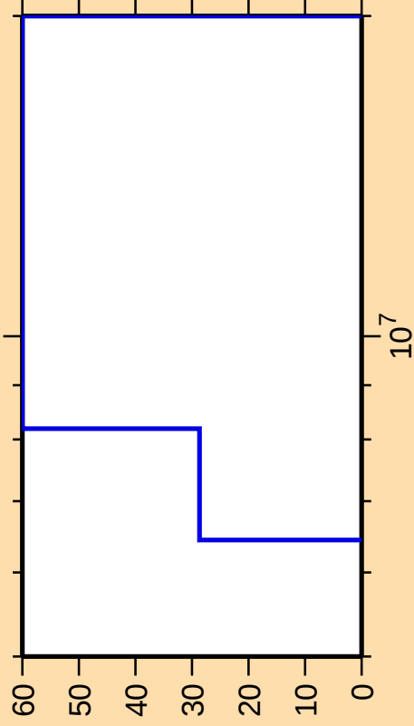
\Delta\sigma/\sigma vs. E for ^{152}\text{Dy}(n,p\alpha)
