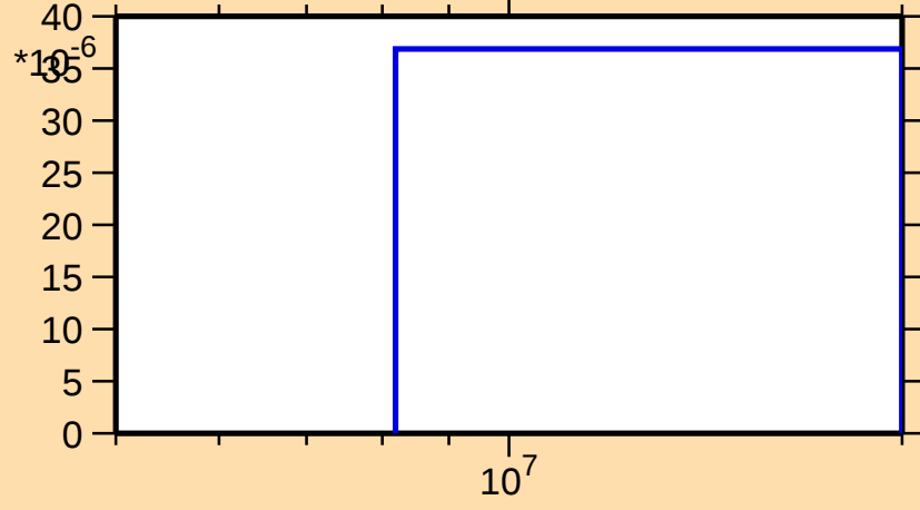
\sigma vs. E for ^{152}\text{Dy}(n,3n)
