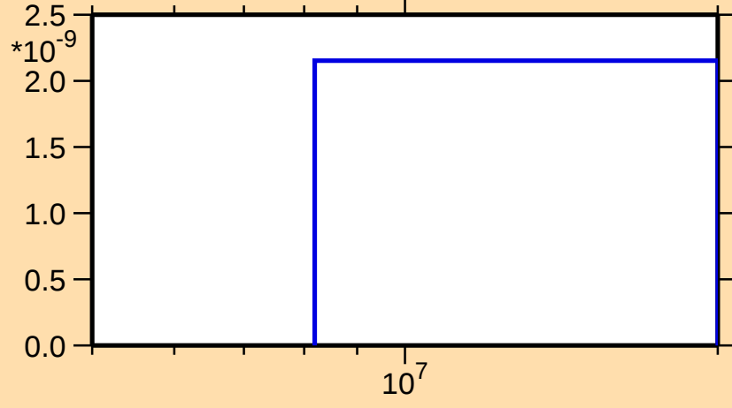
\sigma vs. E for ^{152}\text{Dy}(n,\text{nd})
