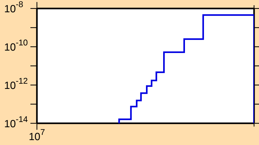
\sigma vs. E for ^{159}\text{Dy}(n,\text{He}3)
