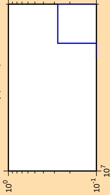
\Delta\sigma/\sigma vs. E for ^{159}\text{Dy} (mt 34)
