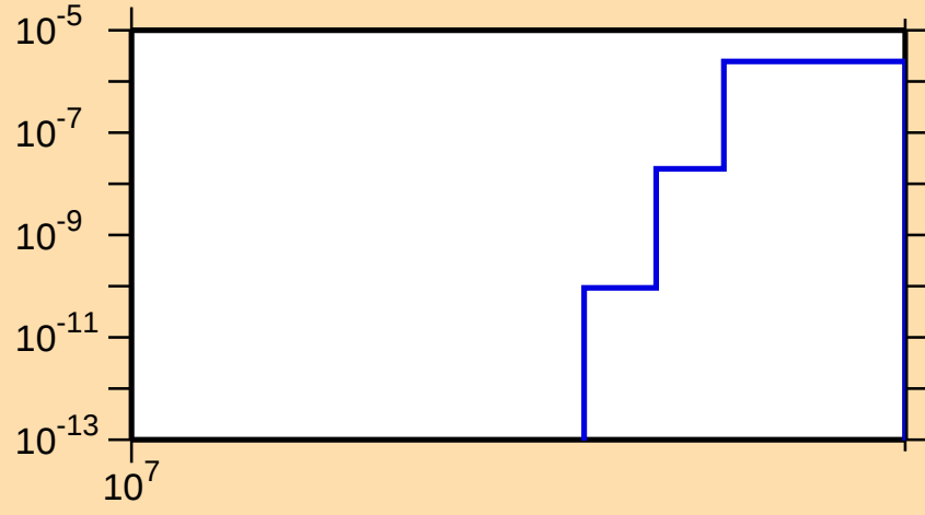
\sigma vs. E for ^{159}\text{Dy}(n,2np)
