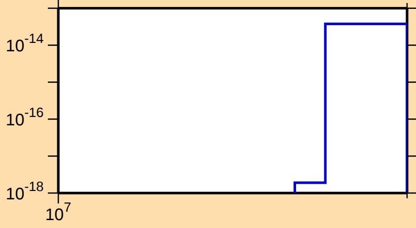
\sigma vs. E for ^{159}\text{Dy} (mt 34)
