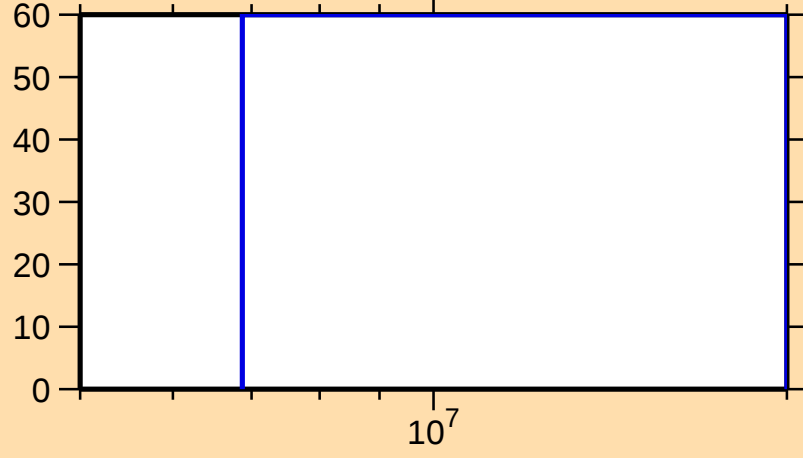
\Delta\sigma/\sigma vs. E for ^{159}\text{Dy}(n,\text{inel.})
