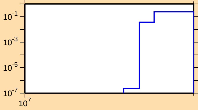
\sigma vs. E for ^{159}\text{Dy}(n,3n)
