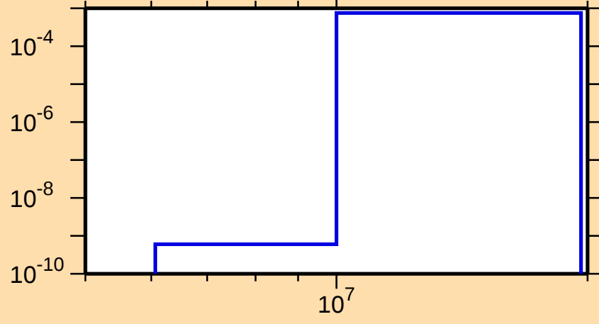
\sigma vs. E for ^{159}\text{Dy}(n,np)
