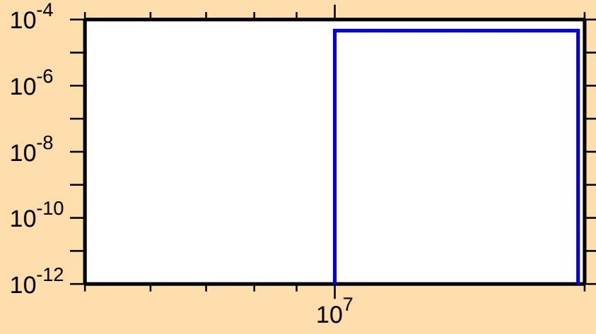
\sigma vs. E for ^{159}\text{Dy}(n,t)
