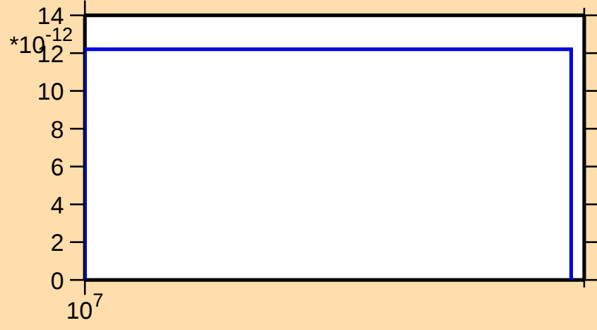
\sigma vs. E for ^{159}\text{Dy}(n,p\alpha)
