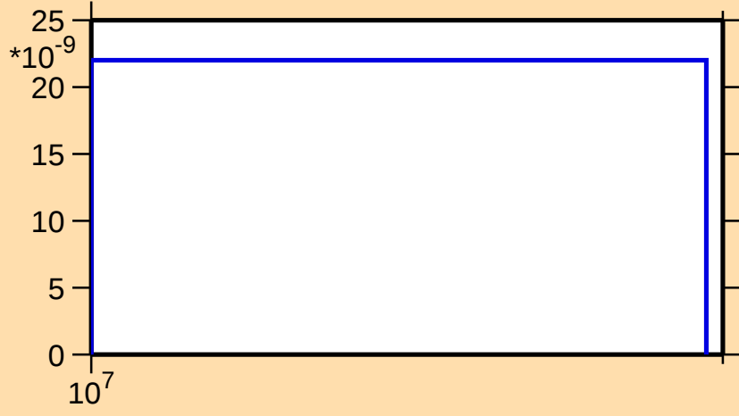
\sigma vs. E for ^{159}\text{Dy}(n,2np)
