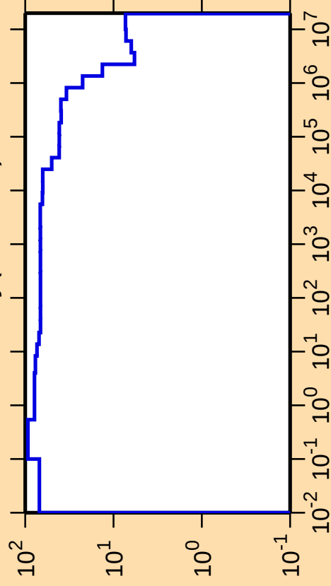
\Delta\sigma/\sigma vs. E for ^{159}\text{Dy}(n,\text{nonel.})
