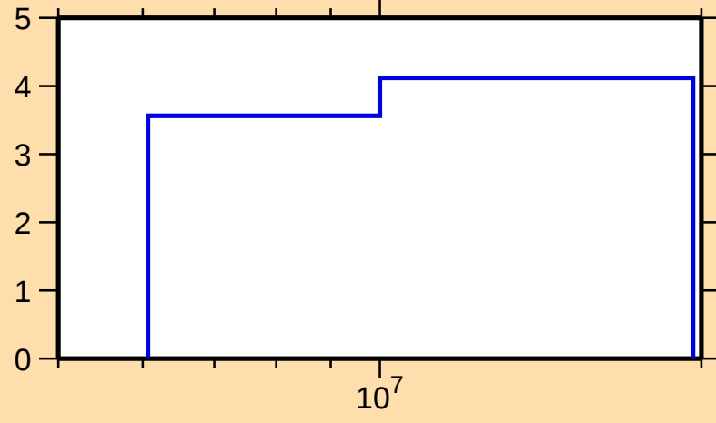
\Delta\sigma/\sigma vs. E for ^{159}\text{Dy}(n,\text{tot.})
