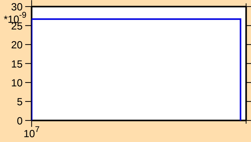
\sigma vs. E for ^{159}\text{Dy}(n,\text{nd})
