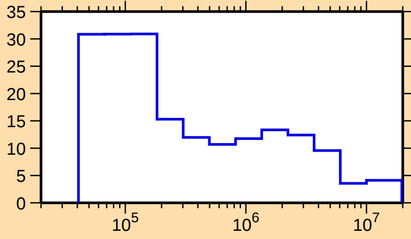
\Delta\sigma/\sigma vs. E for ^{159}\text{Dy}(n,\text{tot.})
