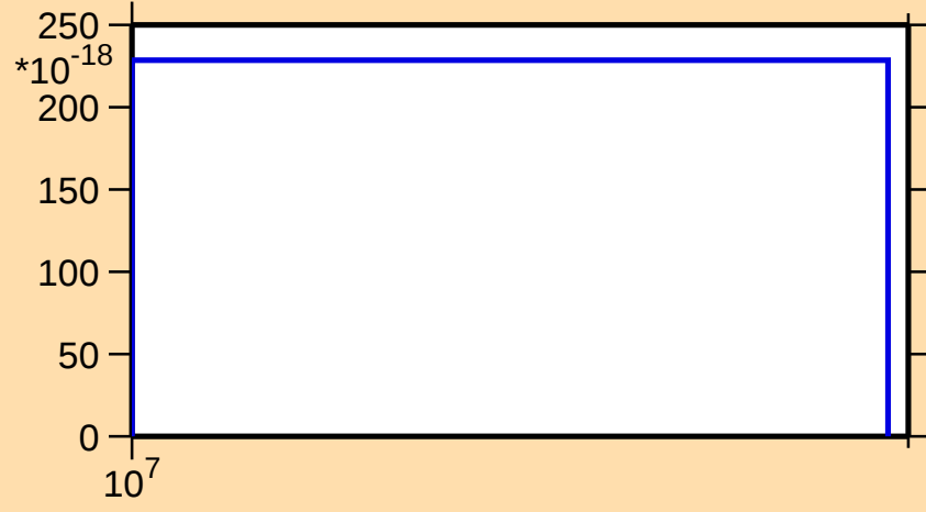
\sigma vs. E for ^{159}\text{Dy}(\text{mt } 34)
