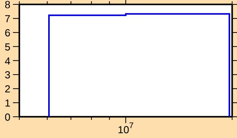
\Delta\sigma/\sigma vs. E for ^{159}\text{Dy}(n,\text{nonel.})
