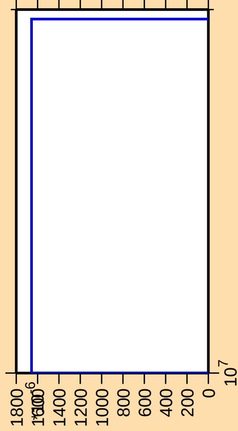
\Delta\sigma/\sigma vs. E for ^{159}\text{Dy}(\text{mt } 34)
