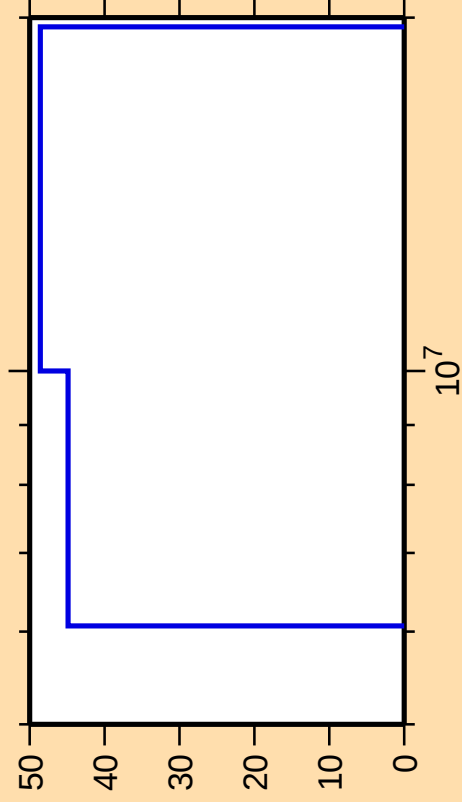
\Delta\sigma/\sigma vs. E for ^{159}\text{Dy}(n,n_1)
