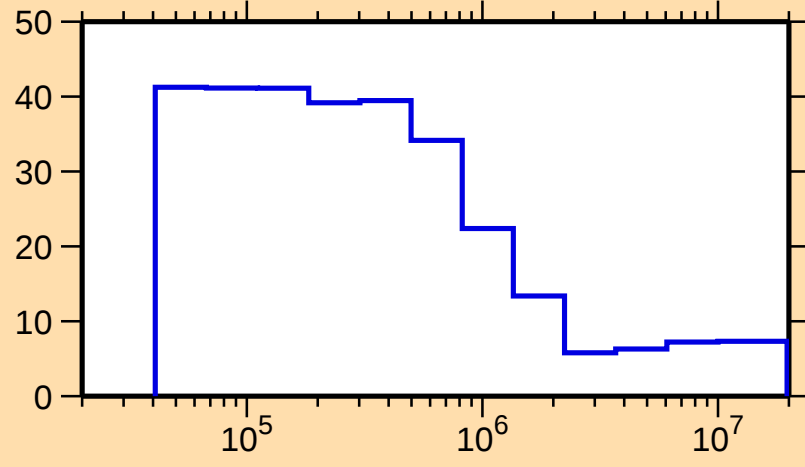
\Delta\sigma/\sigma vs. E for ^{159}\text{Dy}(n,\text{nonel.})
