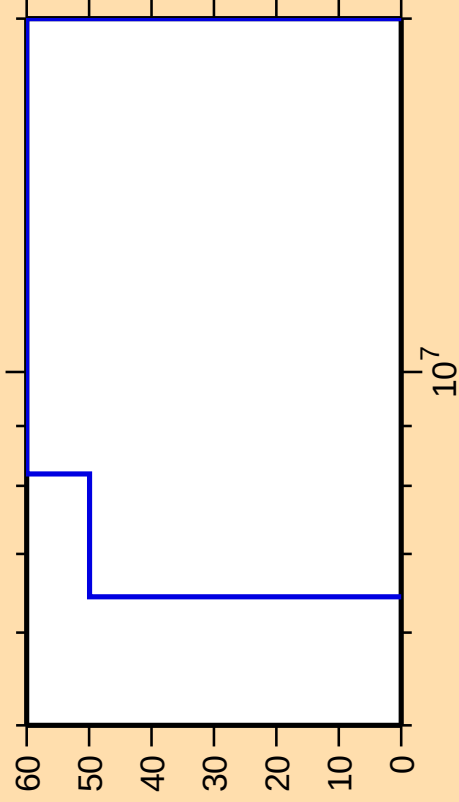
\Delta\sigma/\sigma vs. E for ^{159}\text{Dy}(n,n\text{cont.})
