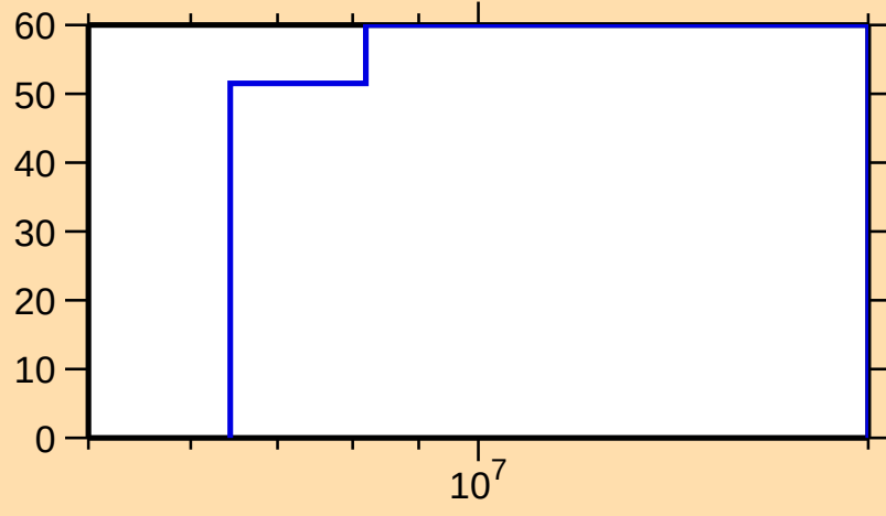
\Delta\sigma/\sigma vs. E for ^{159}\text{Dy}(n,\text{inel.})
