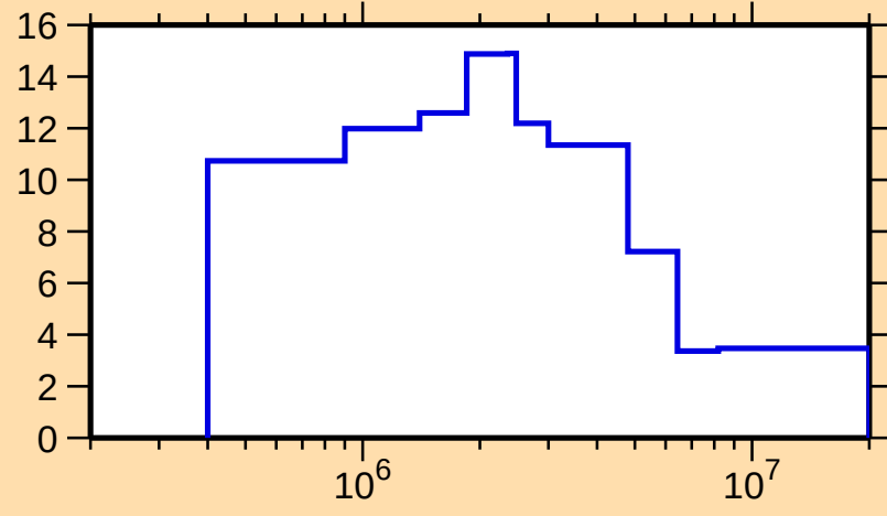
\Delta\sigma/\sigma vs. E for ^{159}\text{Dy}(n,\text{tot.})
