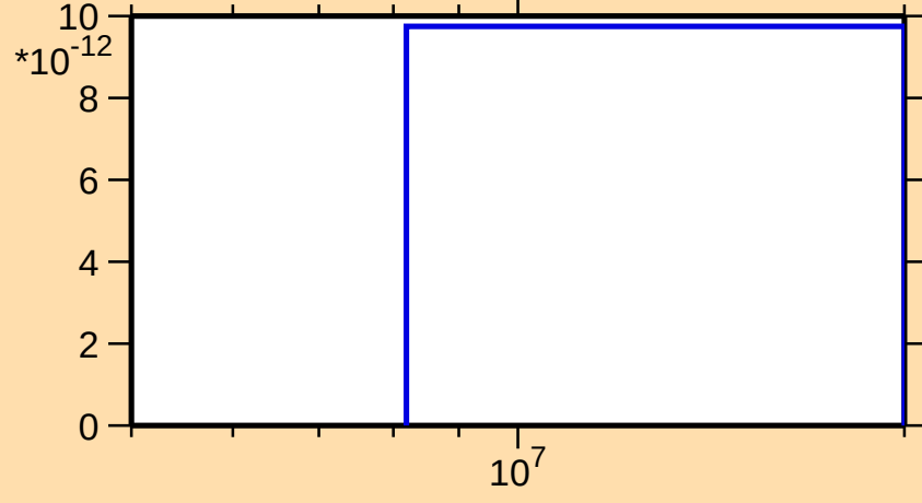
\sigma vs. E for ^{159}\text{Dy}(n,nt)
