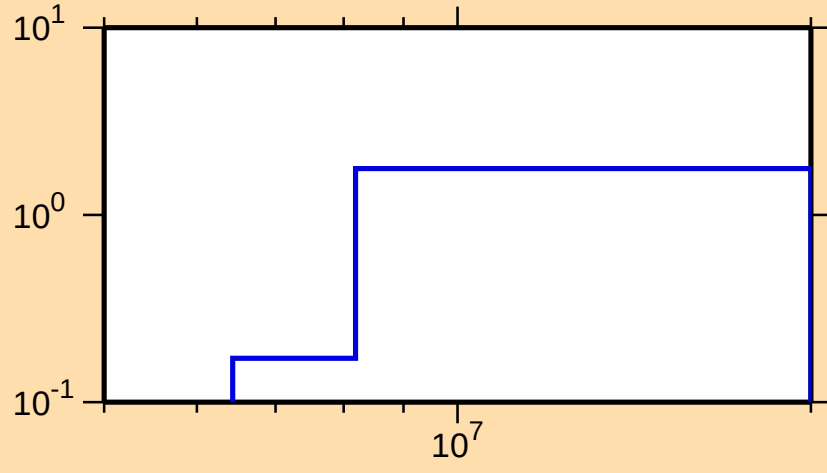
\sigma vs. E for ^{159}\text{Dy}(n,2n)
