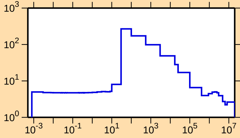
\sigma vs. E for ^{159}\text{Dy}(n,\text{el.})
