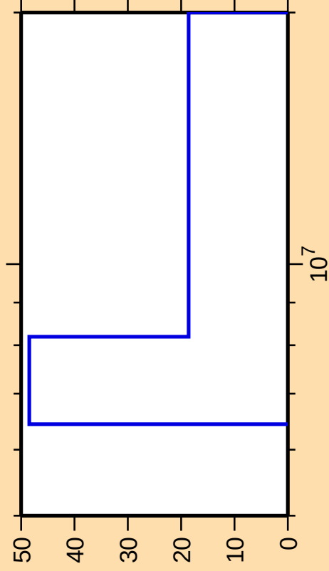
\Delta\sigma/\sigma vs. E for ^{159}\text{Dy}(n,2n)
