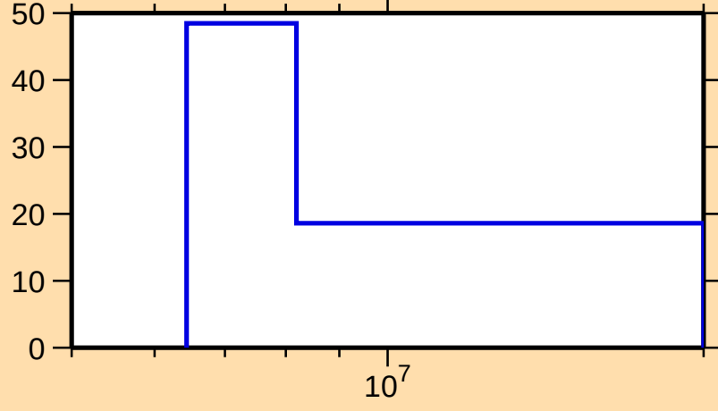
\Delta\sigma/\sigma vs. E for ^{159}\text{Dy}(n,2n)
