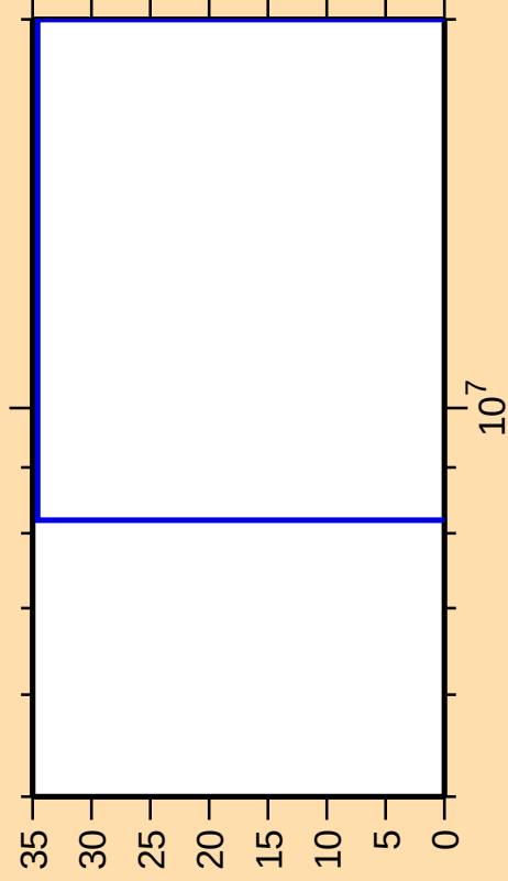
\Delta\sigma/\sigma vs. E for ^{159}\text{Dy}(n,nt)
