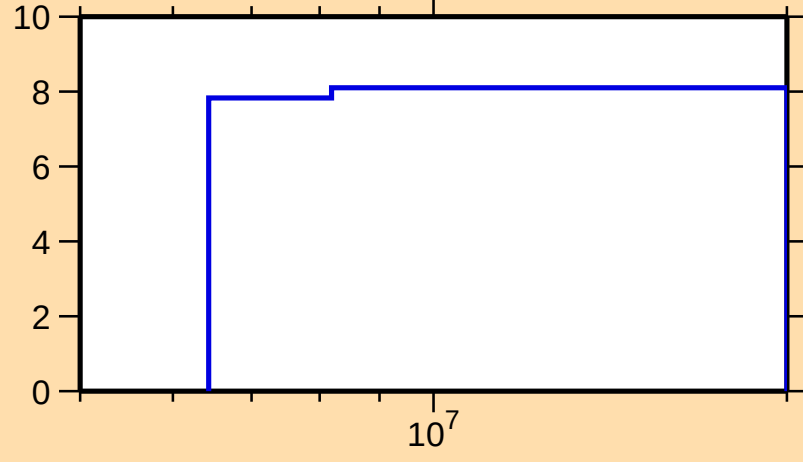
\Delta\sigma/\sigma vs. E for ^{159}\text{Dy}(n,\text{el.})
