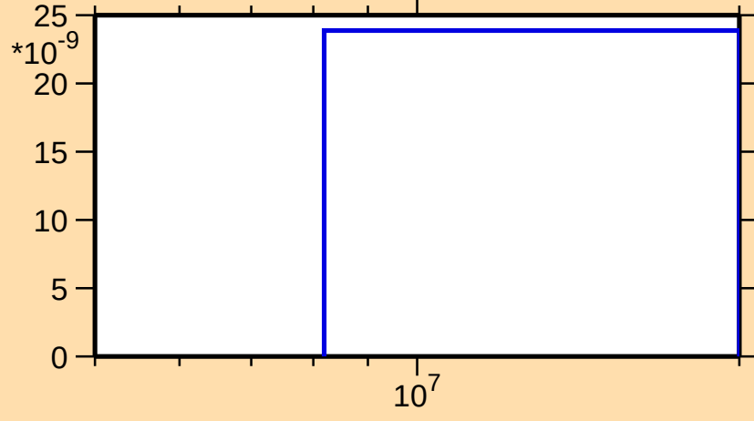
\sigma vs. E for ^{159}\text{Dy}(n,\text{nd})
