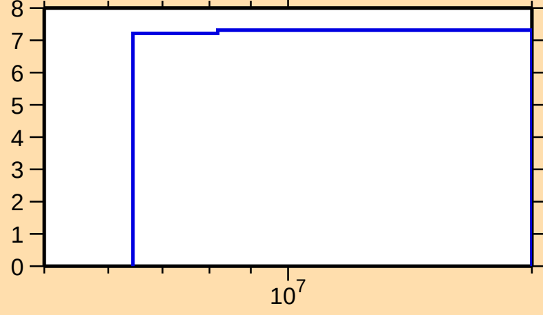
\Delta\sigma/\sigma vs. E for ^{159}\text{Dy}(n,\text{nonel.})
