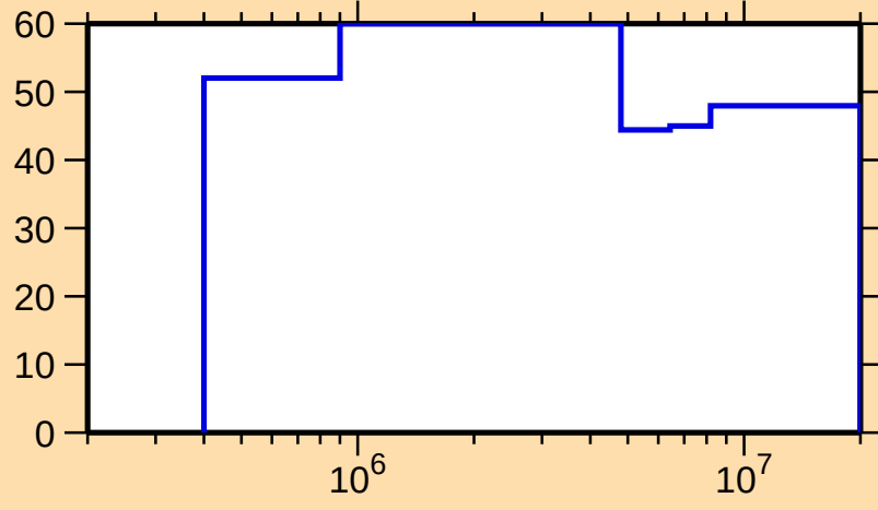
\Delta\sigma/\sigma vs. E for ^{159}\text{Dy}(n,n_1)
