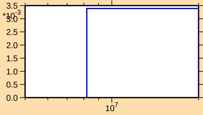
\sigma vs. E for ^{159}\text{Dy}(n,3n)
