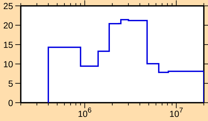
\Delta\sigma/\sigma vs. E for ^{159}\text{Dy}(n,\text{el.})
