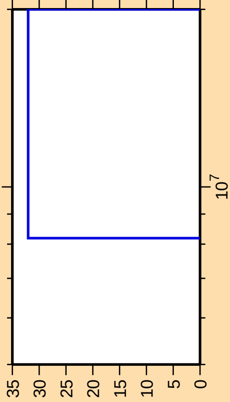
\Delta\sigma/\sigma vs. E for ^{159}\text{Dy}(n,3n)
