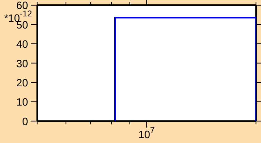
\sigma vs. E for ^{159}\text{Dy}(n,\text{He}3)
