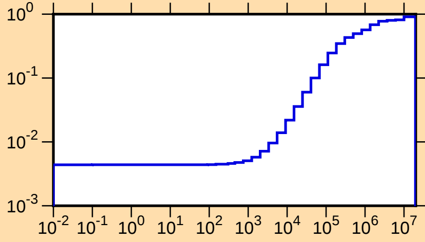
\mu vs. E for ^{161}\text{Dy}(\text{mt251})
