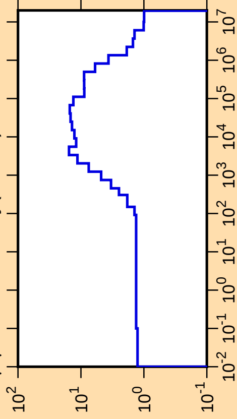
\Delta\mu/\mu vs. E for ^{161}\text{Dy}(\text{mt251})
