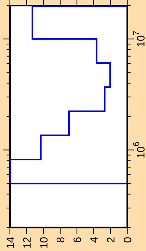
\Delta\sigma/\sigma vs. E for ^{161}\text{Dy}(n,n\text{cont.})
