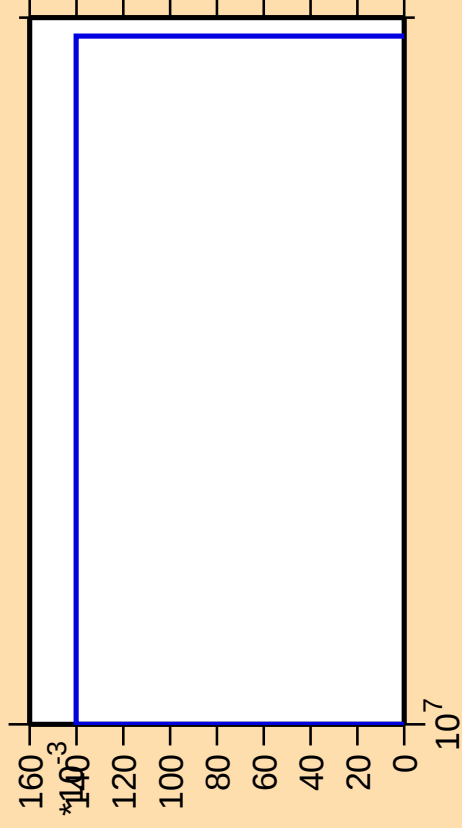
\Delta\sigma/\sigma vs. E for ^{161}\text{Dy}(n,p\alpha)
