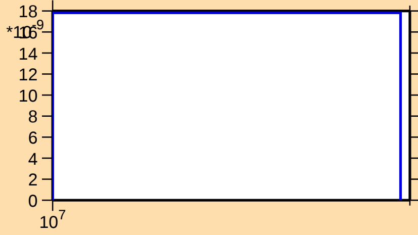
\sigma vs. E for ^{161}\text{Dy}(n,\text{nd})
