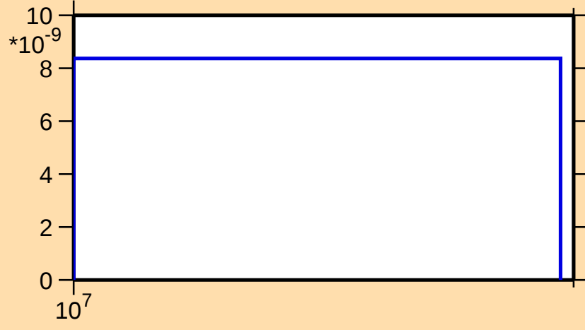
\sigma vs. E for ^{161}\text{Dy}(n,2n\alpha)
