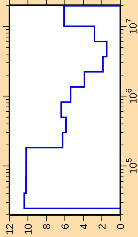
\Delta\sigma/\sigma vs. E for ^{161}\text{Dy}(n,\text{inel.})
