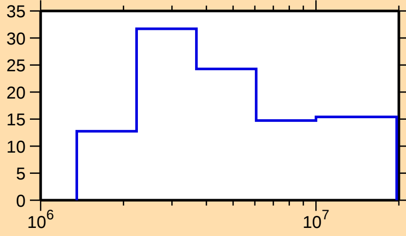
\Delta\sigma/\sigma vs. E for ^{161}\text{Dy}(n,p)
