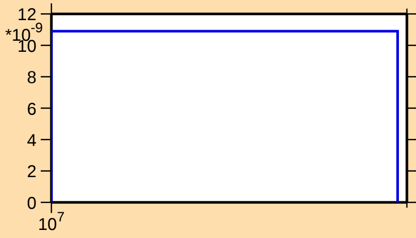
\sigma vs. E for ^{161}\text{Dy}(n,2np)
