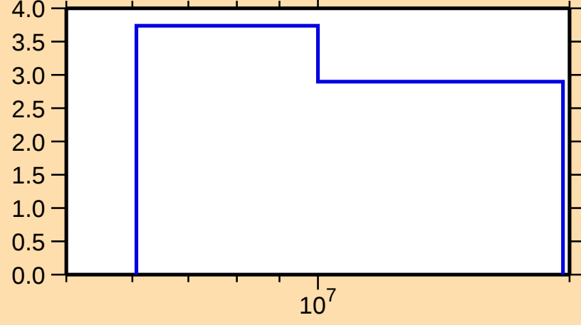
\Delta\sigma/\sigma vs. E for ^{161}\text{Dy}(n,2n)
