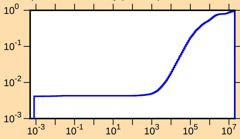
\mu vs. E for ^{163}\text{Dy}(\text{mt251})
