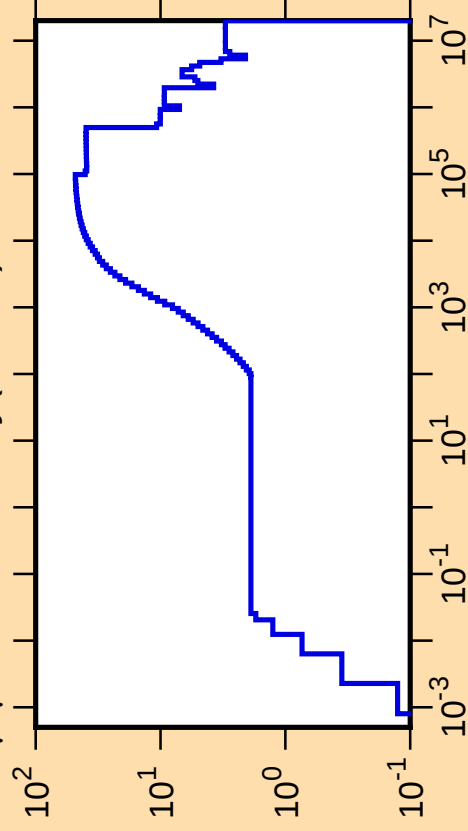
\Delta\mu/\mu vs. E for ^{163}\text{Dy}(\text{mt251})
