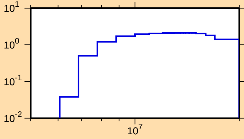
\sigma vs. E for ^{163}\text{Dy}(n,2n)
