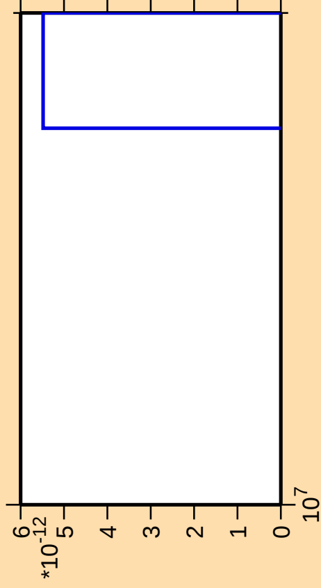
\Delta\sigma/\sigma vs. E for ^{163}\text{Dy} (mt 11)
