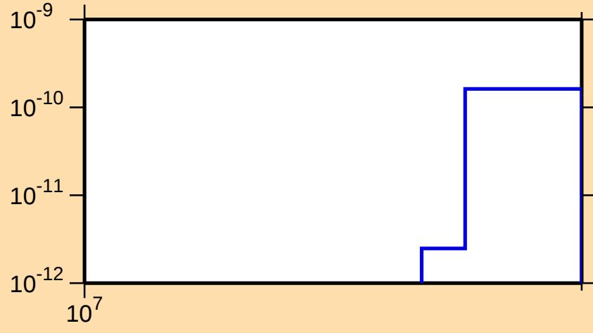
\sigma vs. E for ^{163}\text{Dy}(n,\text{He}3)
