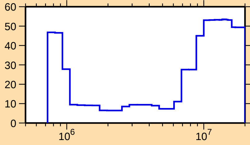
\Delta\sigma/\sigma vs. E for ^{163}\text{Dy}(n,n\text{cont.})
