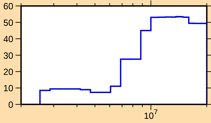
\Delta\sigma/\sigma vs. E for ^{163}\text{Dy}(n,n\text{cont.})
