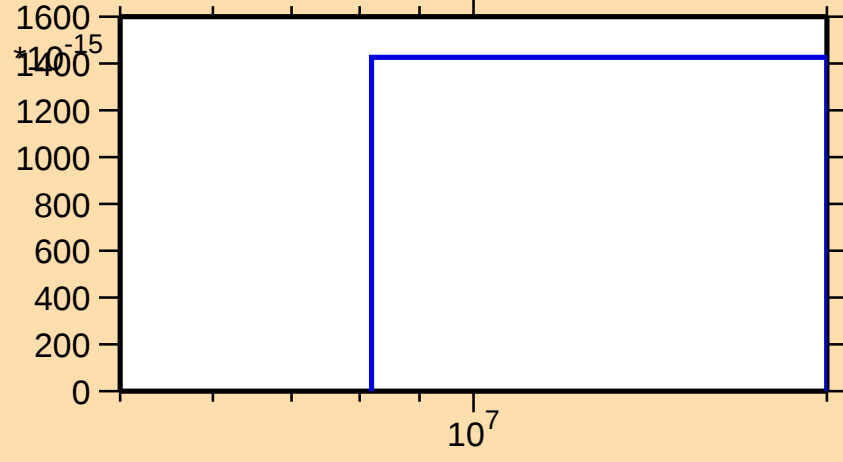
\sigma vs. E for ^{163}\text{Dy}(n,\text{He}3)
