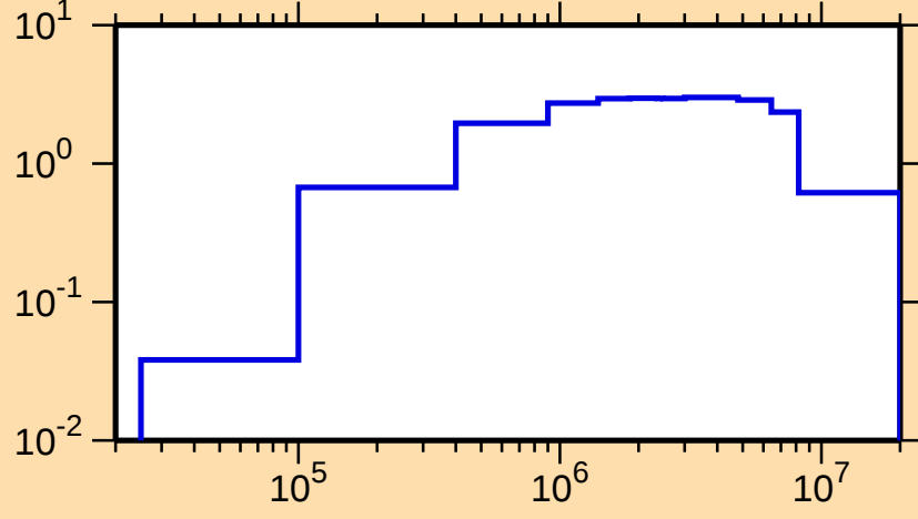
\sigma vs. E for ^{163}\text{Dy}(n,\text{inel.})
