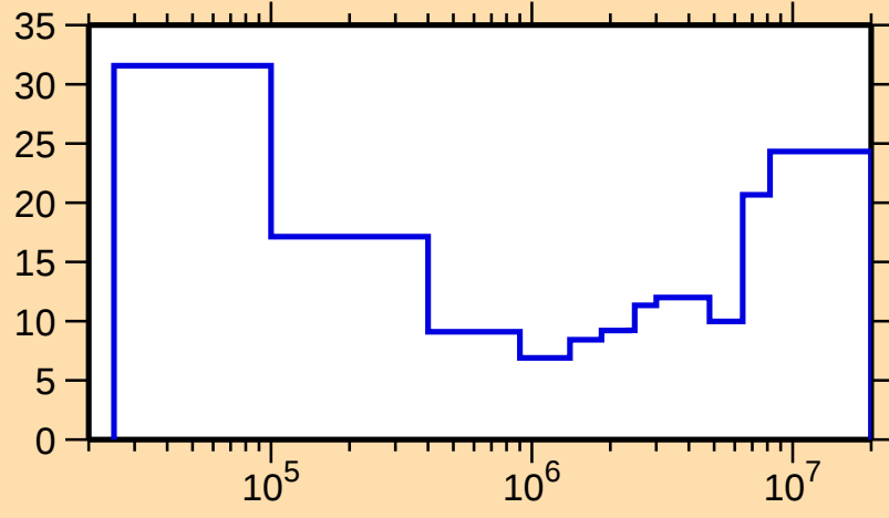
\Delta\sigma/\sigma vs. E for ^{163}\text{Dy}(n,\text{inel.})
