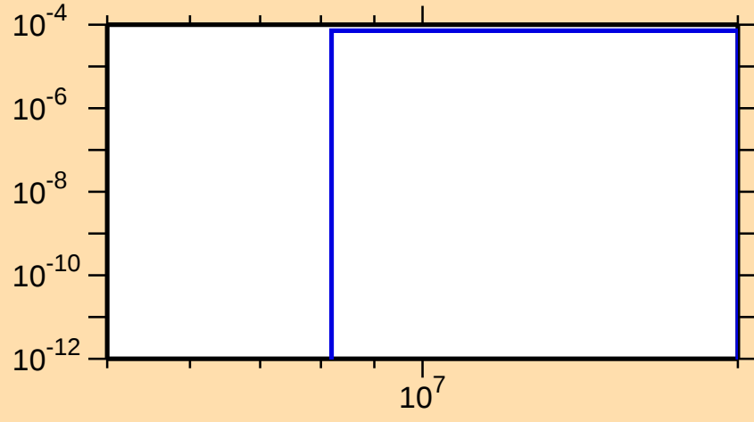
\sigma vs. E for ^{163}\text{Dy}(n,np)
