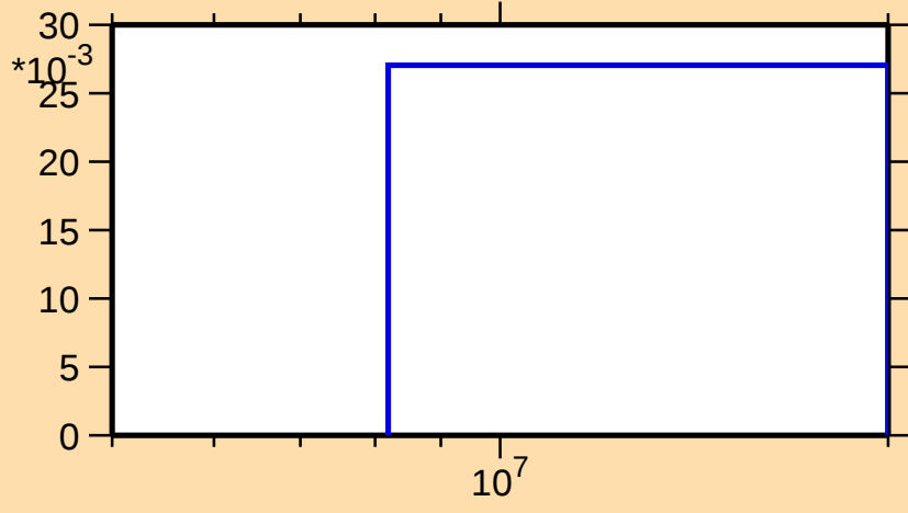
\sigma vs. E for ^{163}\text{Dy}(n,3n)
