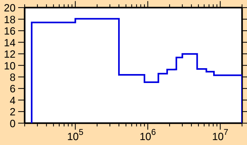
\Delta\sigma/\sigma vs. E for ^{163}\text{Dy}(n,\text{nonel.})
