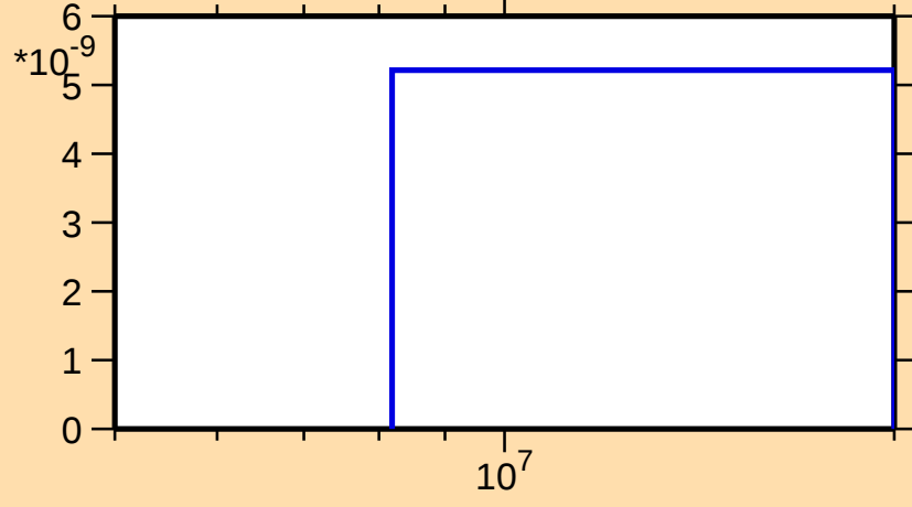
\sigma vs. E for ^{163}\text{Dy}(n,nd)
