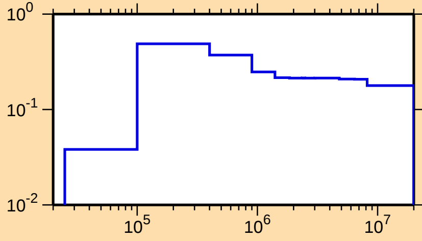
\sigma vs. E for ^{163}\text{Dy}(n,n_1)
