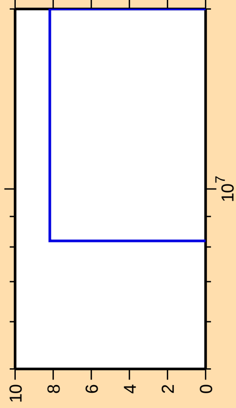
\Delta\sigma/\sigma vs. E for ^{163}\text{Dy}(n,\text{He}3)
