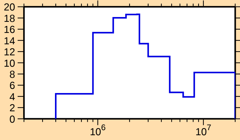
\Delta\sigma/\sigma vs. E for ^{163}\text{Dy}(n,\text{tot.})
