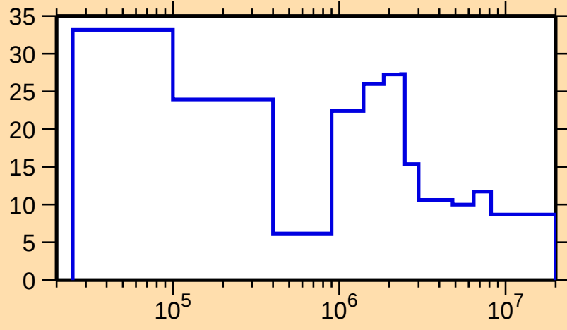
\Delta\sigma/\sigma vs. E for ^{163}\text{Dy}(n,\text{el.})
