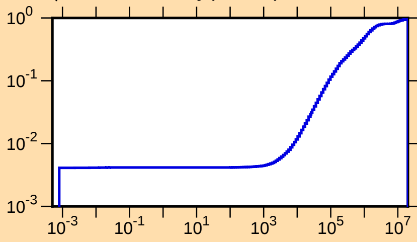
\mu vs. E for ^{164}\text{Dy}(\text{mt251})
