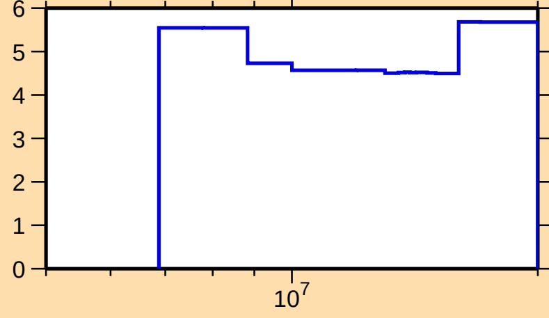
\Delta\sigma/\sigma vs. E for ^{164}\text{Dy}(n,\text{nonel.})
