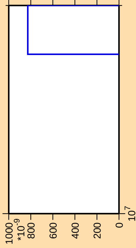
\Delta\sigma/\sigma vs. E for ^{164}\text{Dy}(\text{mt } 11)
