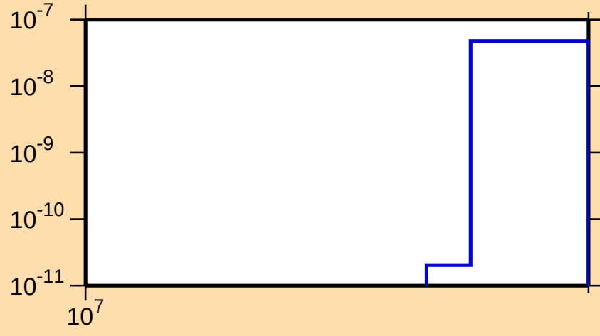
\sigma vs. E for ^{164}\text{Dy}(n,\text{nd})
