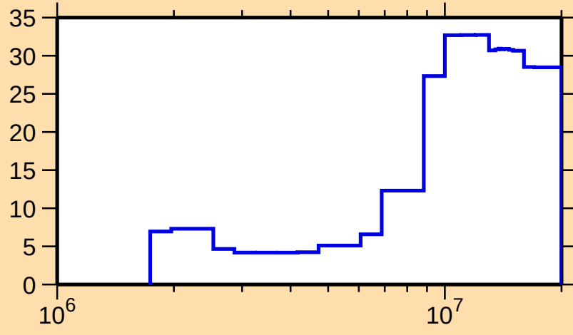
\Delta\sigma/\sigma vs. E for ^{164}\text{Dy}(n,\text{inel.})
