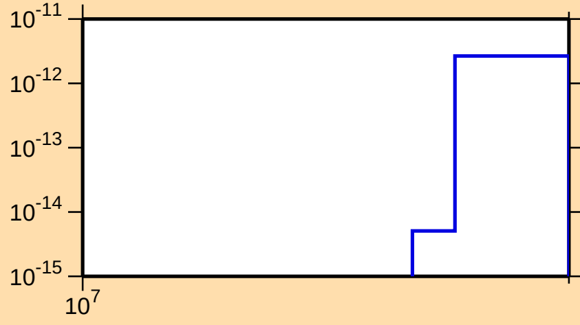
\sigma vs. E for ^{164}\text{Dy}(n,\text{He3})
