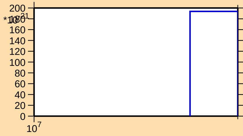
\sigma vs. E for ^{164}\text{Dy}(\text{mt } 11)
