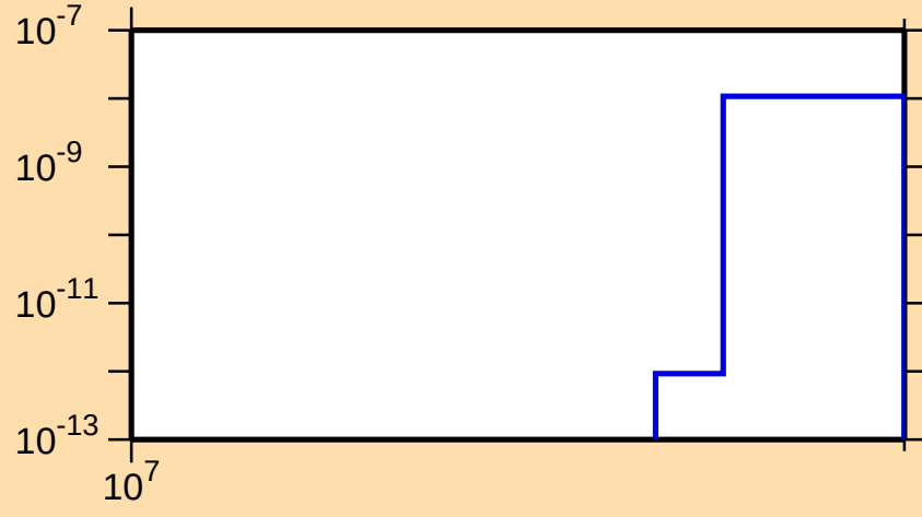
\sigma vs. E for ^{164}\text{Dy}(n,nt)
