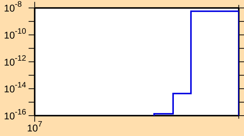
\sigma vs. E for ^{164}\text{Dy}(n,2np)
