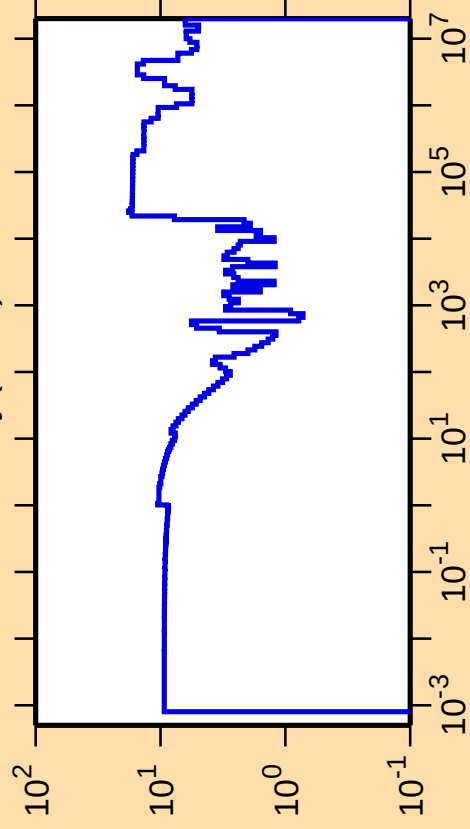
\Delta\sigma/\sigma vs. E for ^{164}\text{Dy}(n,\text{el.})
