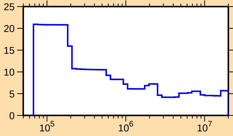
\Delta\sigma/\sigma vs. E for ^{164}\text{Dy}(n,\text{nonel.})
