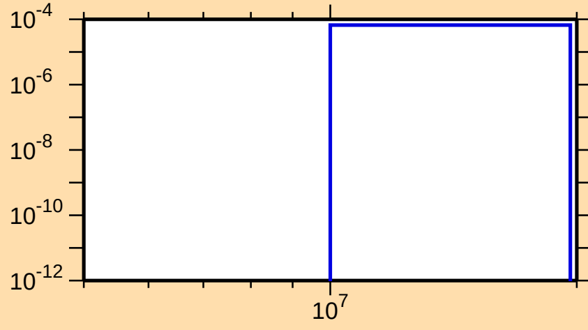
\sigma vs. E for ^{164}\text{Dy}(n,np)
