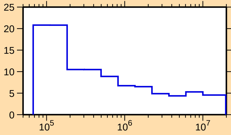
\Delta\sigma/\sigma vs. E for ^{164}\text{Dy}(\text{n,nonel.})
