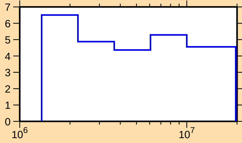
\Delta\sigma/\sigma vs. E for ^{164}\text{Dy}(\text{n},\text{nonel.})
