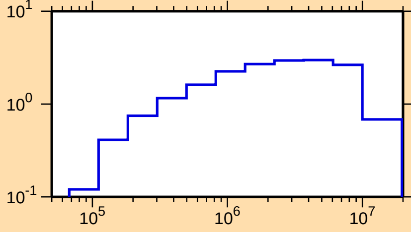
\sigma vs. E for ^{164}\text{Dy}(n,\text{inel.})
