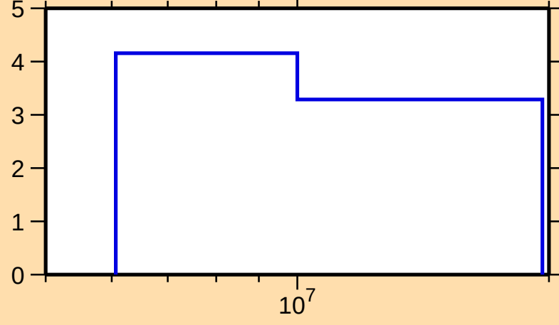
\Delta\sigma/\sigma vs. E for ^{164}\text{Dy}(n,\text{tot.})
