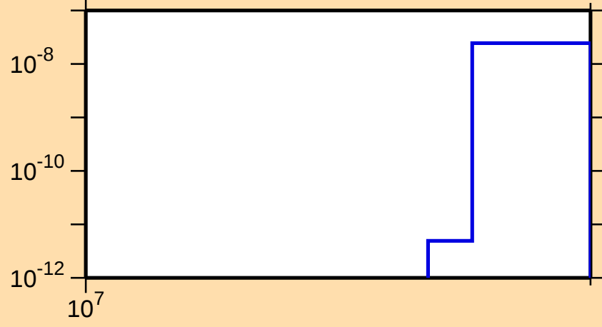
\sigma vs. E for ^{166}\text{Dy}(n,nd)
