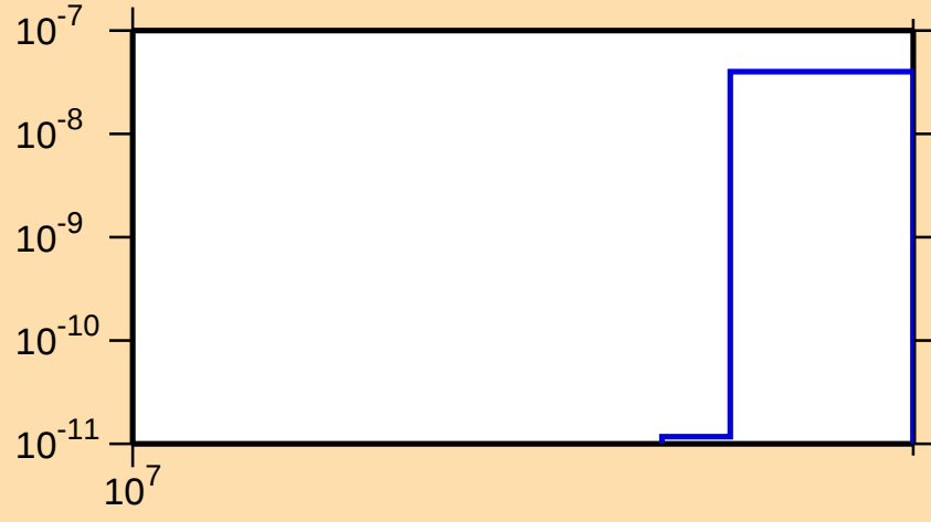
\sigma vs. E for ^{166}\text{Dy}(n,nt)
