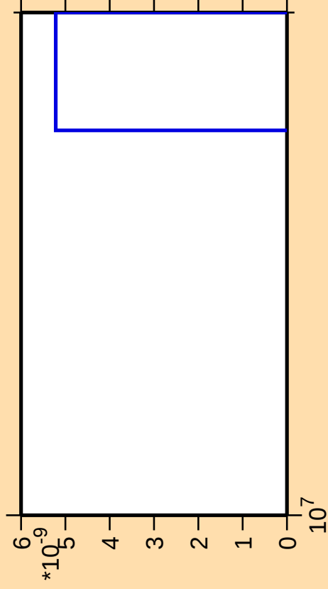
\Delta\sigma/\sigma vs. E for ^{166}\text{Dy} (mt 11)
