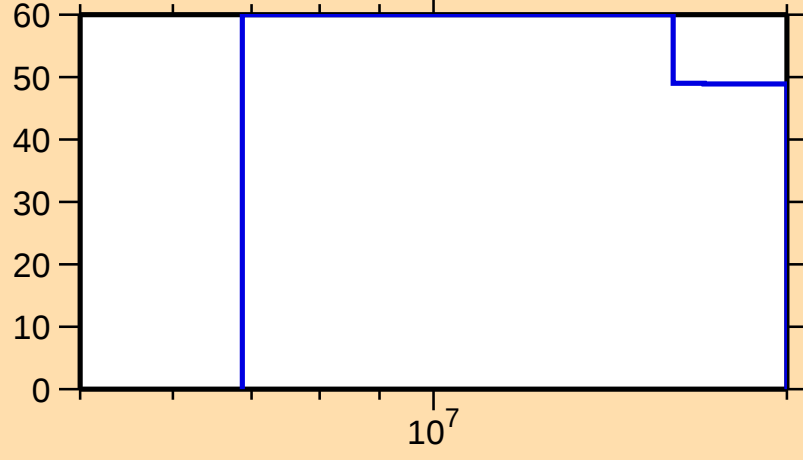
\Delta\sigma/\sigma vs. E for ^{166}\text{Dy}(n,\text{inel.})
