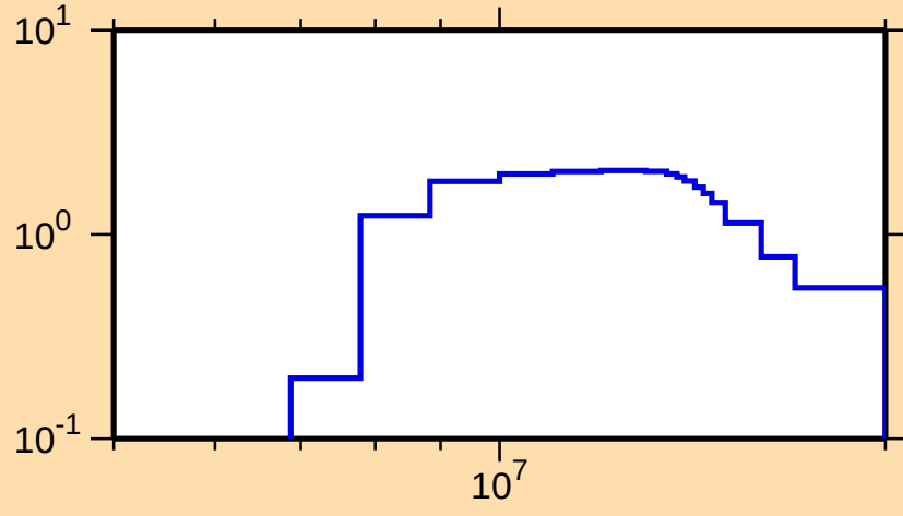
\sigma vs. E for ^{166}\text{Dy}(n,2n)
