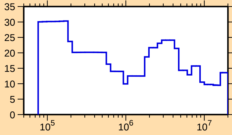
\Delta\sigma/\sigma vs. E for ^{166}\text{Dy}(n,\text{el.})
