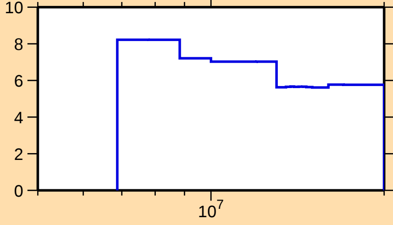
\Delta\sigma/\sigma vs. E for ^{166}\text{Dy}(n,\text{nonel.})
