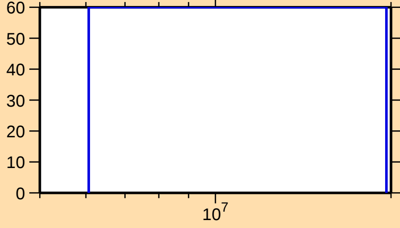
\Delta\sigma/\sigma vs. E for ^{166}\text{Dy}(n,\gamma)
