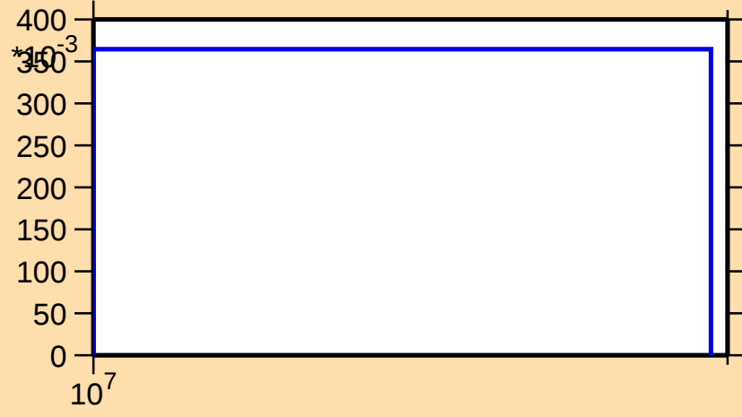
\sigma vs. E for ^{166}\text{Dy}(n,3n)
