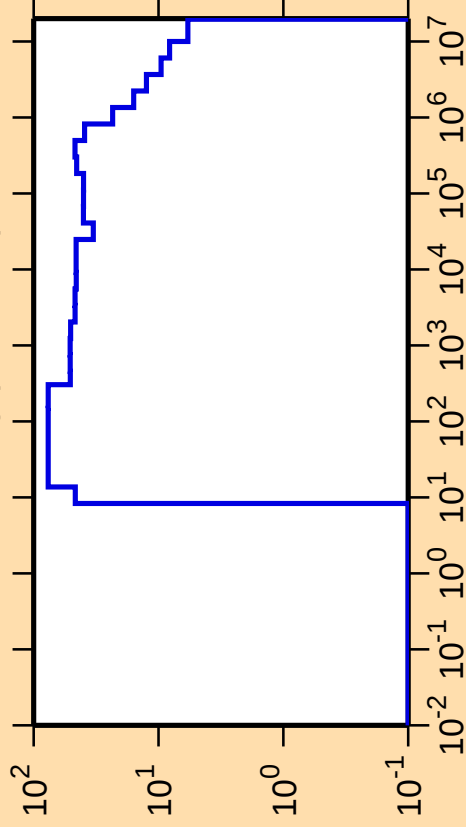
\Delta\sigma/\sigma vs. E for ^{166}\text{Dy}(n,\text{nonel.})
