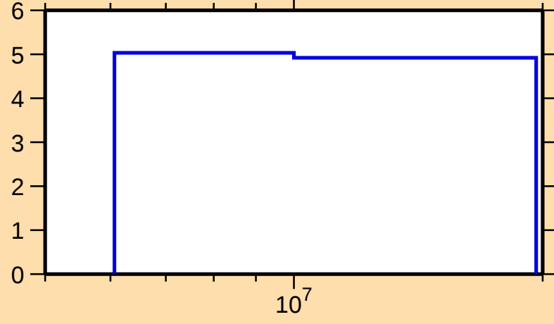
\Delta\sigma/\sigma vs. E for ^{166}\text{Dy}(n,\text{tot.})
