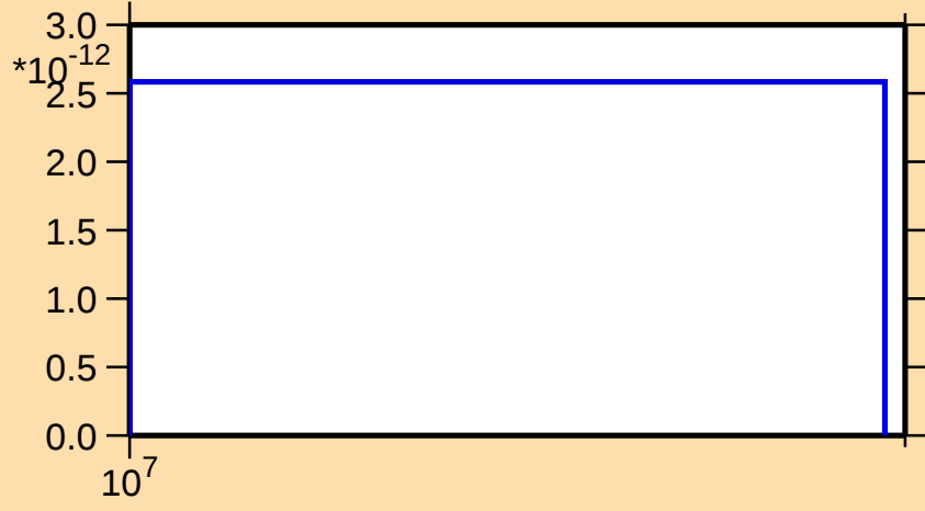
\sigma vs. E for ^{166}\text{Dy}(n,2np)
