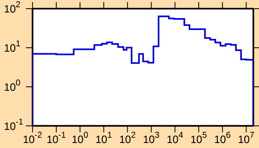
\Delta\sigma/\sigma vs. E for ^{166}\text{Dy}(n,\text{tot.})
