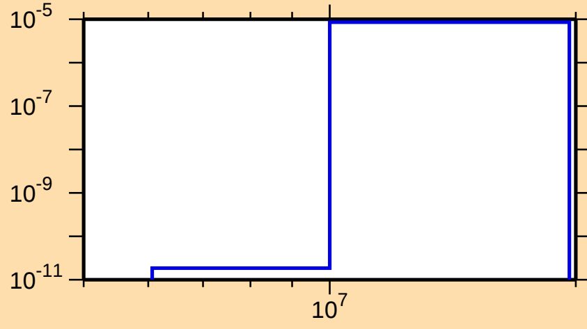
\sigma vs. E for ^{166}\text{Dy}(n,n\alpha)
