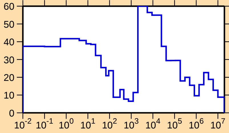
\Delta\sigma/\sigma vs. E for ^{166}\text{Dy}(n,\text{el.})
