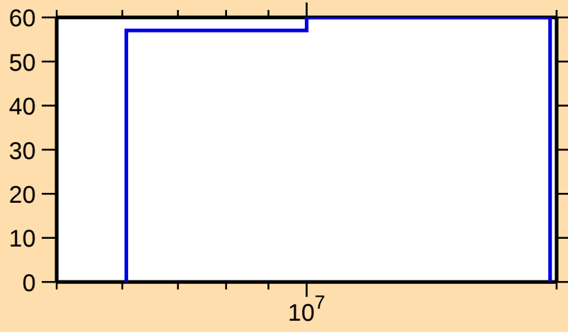
\Delta\sigma/\sigma vs. E for ^{166}\text{Dy}(n,\text{inel.})
