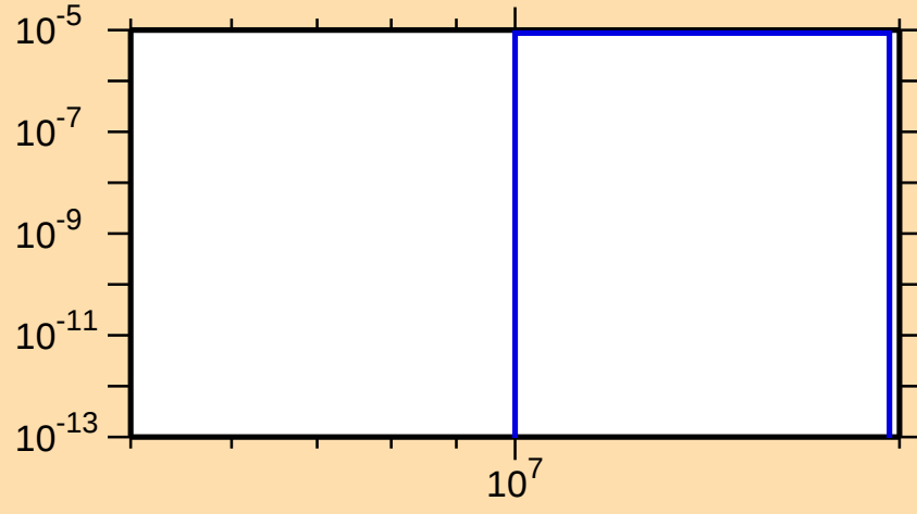
\sigma vs. E for ^{166}\text{Dy}(n,t)
