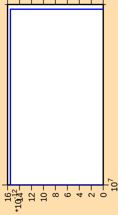
\Delta\sigma/\sigma vs. E for ^{166}\text{Dy}(\text{mt } 11)
