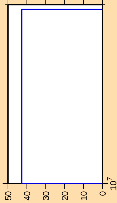
\Delta\sigma/\sigma vs. E for ^{166}\text{Dy}(n,3n)
