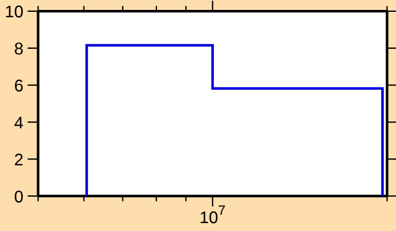
\Delta\sigma/\sigma vs. E for ^{166}\text{Dy}(n,\text{nonel.})
