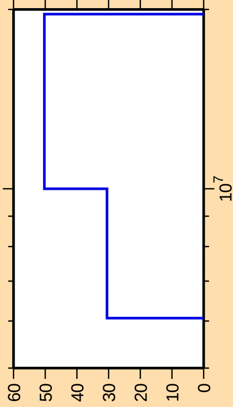
\Delta\sigma/\sigma vs. E for ^{166}\text{Dy}(n,2n)
