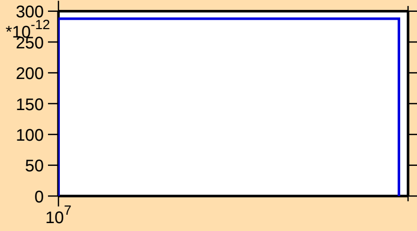
\sigma vs. E for ^{166}\text{Dy}(n,nt)
