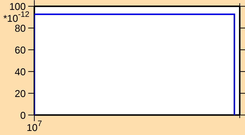
\sigma vs. E for ^{166}\text{Dy}(n,2n\alpha)
