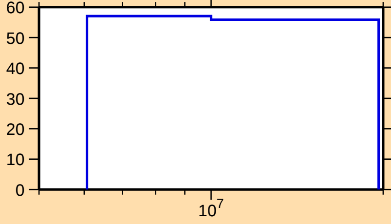
\Delta\sigma/\sigma vs. E for ^{166}\text{Dy}(n,n_1)
