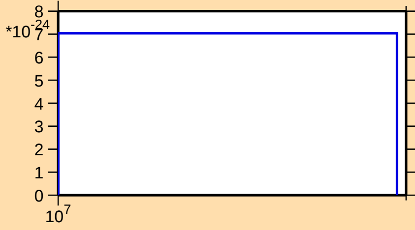
\sigma vs. E for ^{166}\text{Dy}(\text{mt } 11)
