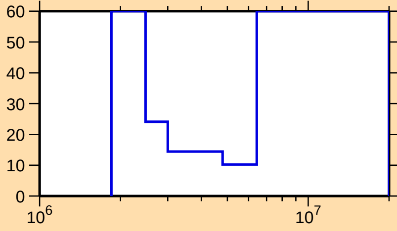
\Delta\sigma/\sigma vs. E for ^{166}\text{Dy}(n,n\text{cont.})
