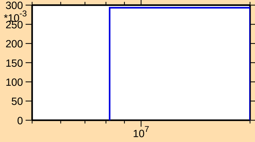
\sigma vs. E for ^{166}\text{Dy}(n,3n)
