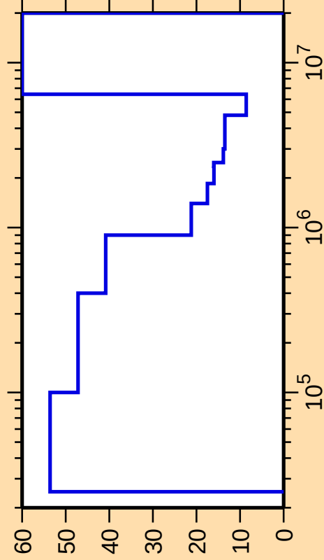
\Delta\sigma/\sigma vs. E for ^{166}\text{Dy}(n,\text{inel.})
