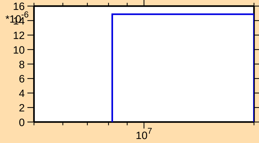
\sigma vs. E for ^{166}\text{Dy}(n,np)
