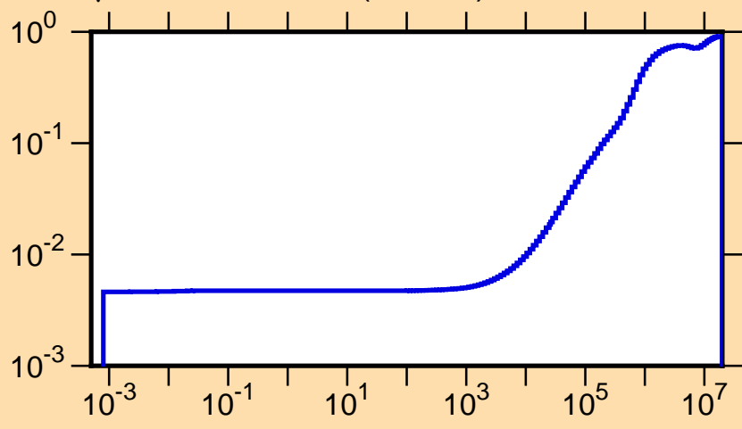
\mu vs. E for ^{146}\text{Er}(\text{mt251})
