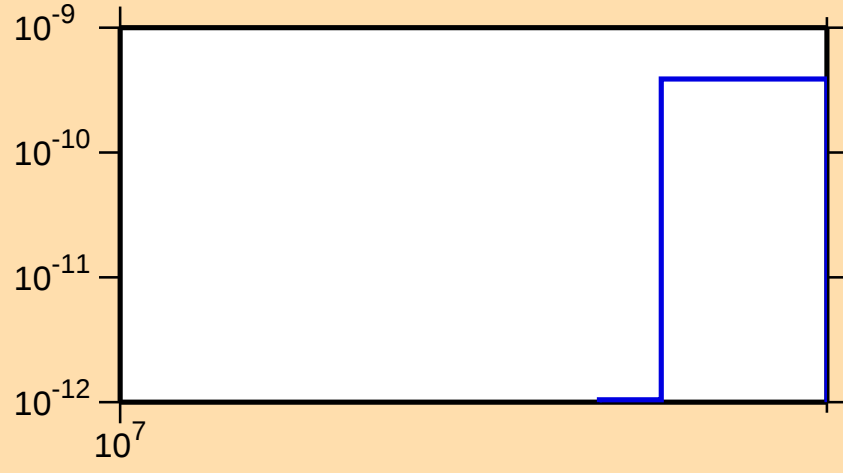
\sigma vs. E for ^{146}\text{Er}(n,\text{nd})
