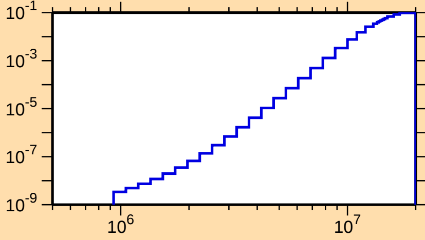
\sigma vs. E for ^{146}\text{Er}(n,p\alpha)
