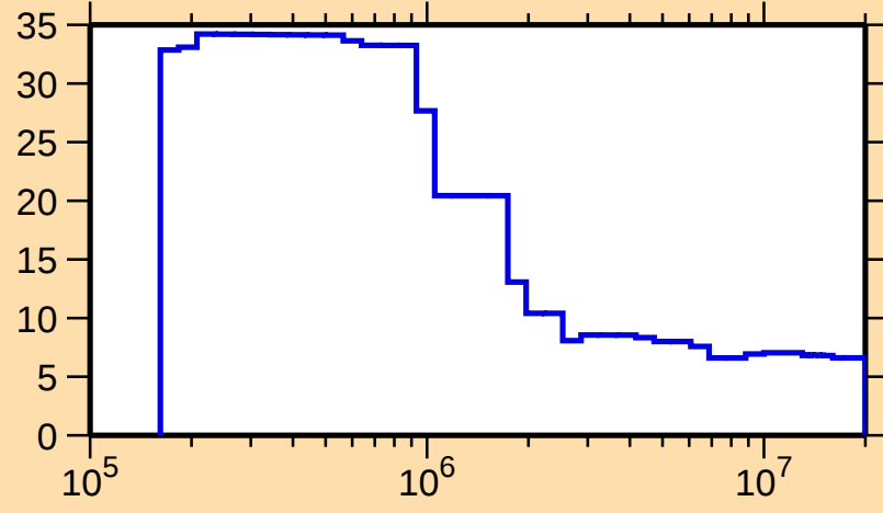
\Delta\sigma/\sigma vs. E for ^{146}\text{Er}(\text{n},\text{nonel.})
