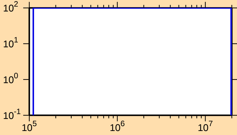
\Delta\sigma/\sigma vs. E for ^{146}\text{Er}(n,\text{ncont.})
