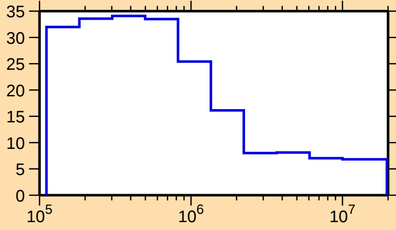
\Delta\sigma/\sigma vs. E for ^{146}\text{Er}(n,\text{nonel.})
