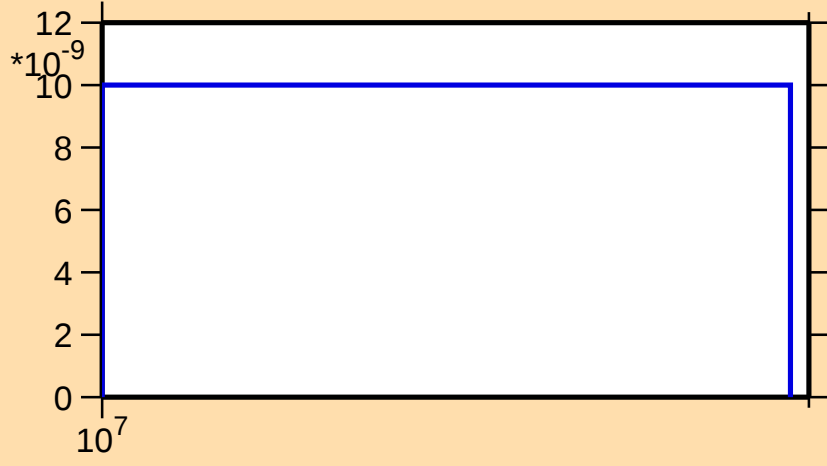
\sigma vs. E for ^{146}\text{Er}(n,2np)
