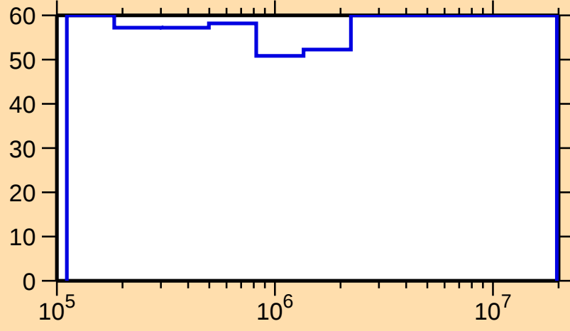
\Delta\sigma/\sigma vs. E for ^{146}\text{Er}(n,n_1)
