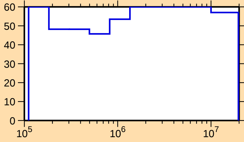
\Delta\sigma/\sigma vs. E for ^{146}\text{Er}(n,\text{inel.})
