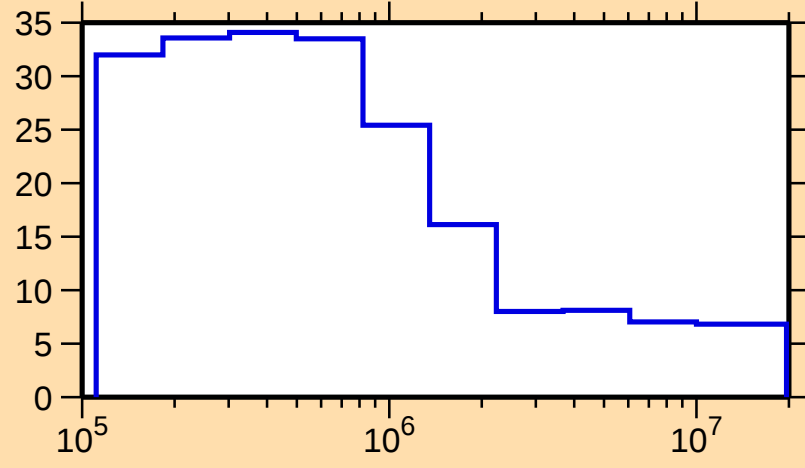
\Delta\sigma/\sigma vs. E for ^{146}\text{Er}(n,n\text{onel.})
