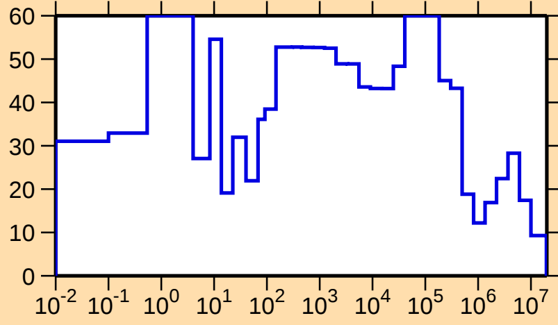
\Delta\sigma/\sigma vs. E for ^{146}\text{Er}(n,\text{el.})
