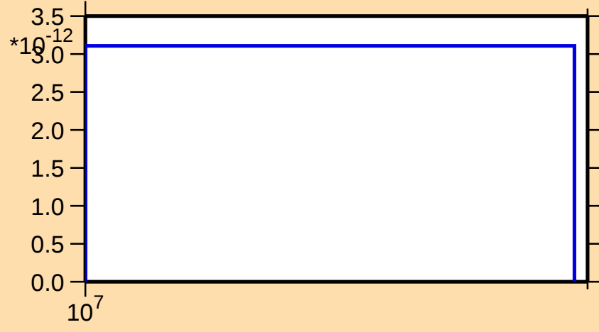
\sigma vs. E for ^{146}\text{Er}(n,\text{nd})
