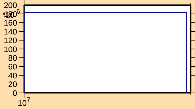
\sigma vs. E for ^{146}\text{Er}(n,2n)
