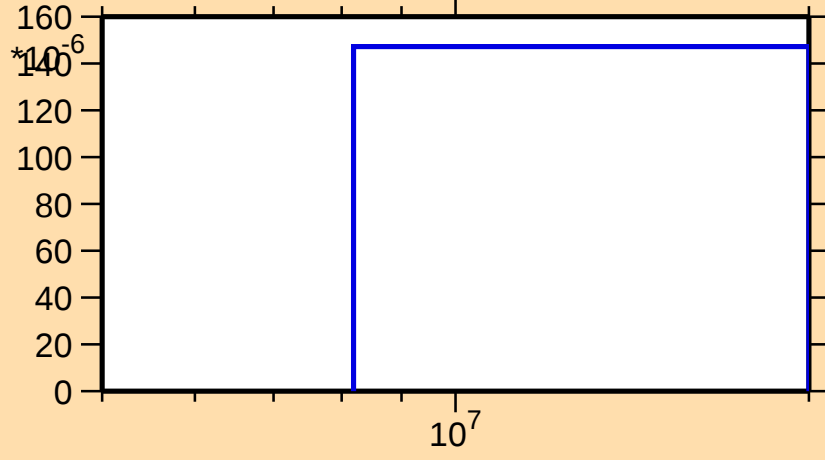
\sigma vs. E for ^{146}\text{Er}(n,2n)
