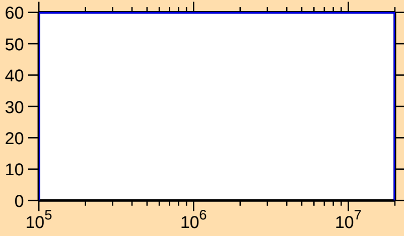
\Delta\sigma/\sigma vs. E for ^{146}\text{Er}(n,\text{ncont.})
