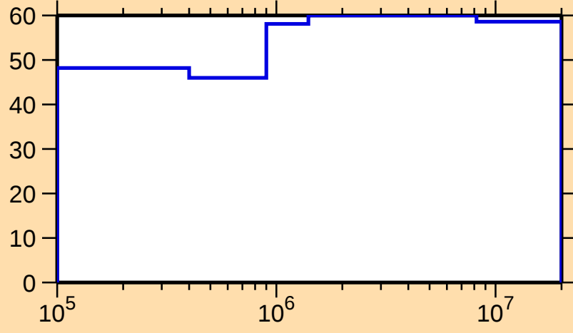
\Delta\sigma/\sigma vs. E for ^{146}\text{Er}(\text{n},\text{inel.})
