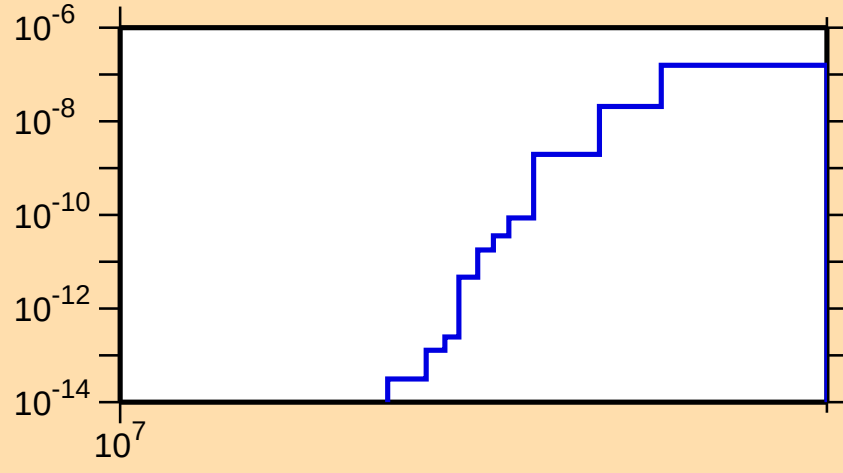
\sigma vs. E for ^{147}\text{Er}(n,\text{nd})
