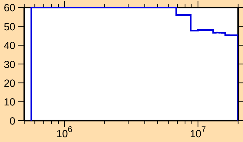
\Delta\sigma/\sigma vs. E for ^{147}\text{Er}(n,n\text{cont.})
