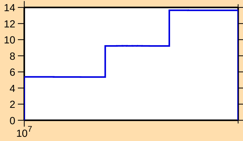
\Delta\sigma/\sigma vs. E for ^{147}\text{Er}(n,\text{el.})
