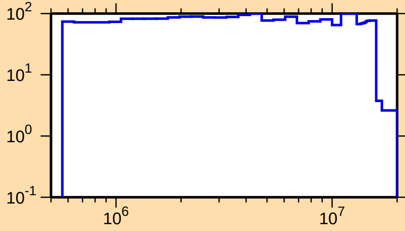
\Delta\sigma/\sigma vs. E for ^{147}\text{Er}(n,n_1)
