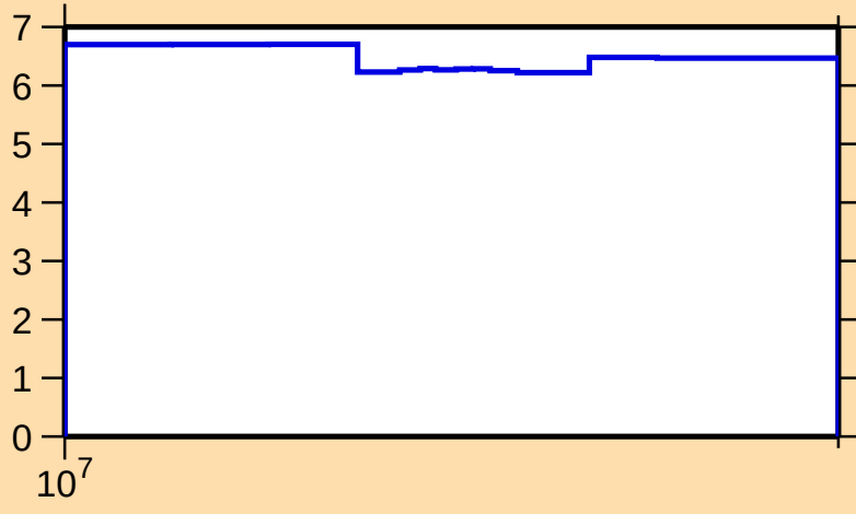
\Delta\sigma/\sigma vs. E for ^{147}\text{Er}(n,\text{nonel.})
