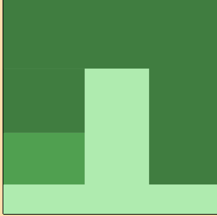
\Delta\sigma/\sigma vs. E for ^{147}\text{Er}(n,\text{tot.})
