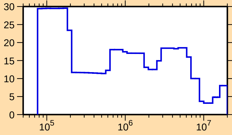
\Delta\sigma/\sigma vs. E for ^{147}\text{Er}(n,\text{tot.})
