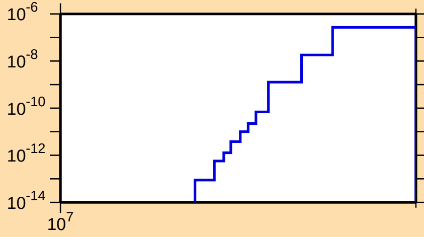
\sigma vs. E for ^{147}\text{Er}(n,2n\alpha)
