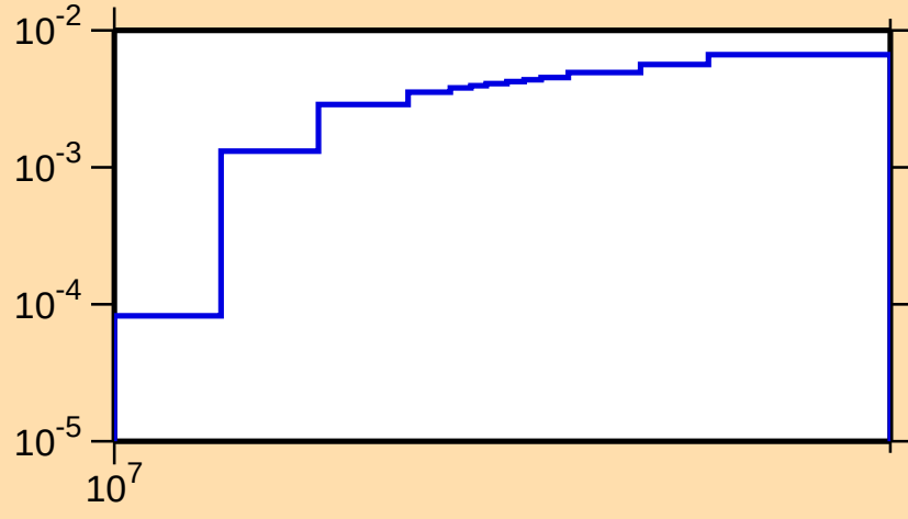
\sigma vs. E for ^{147}\text{Er}(n,2n)
