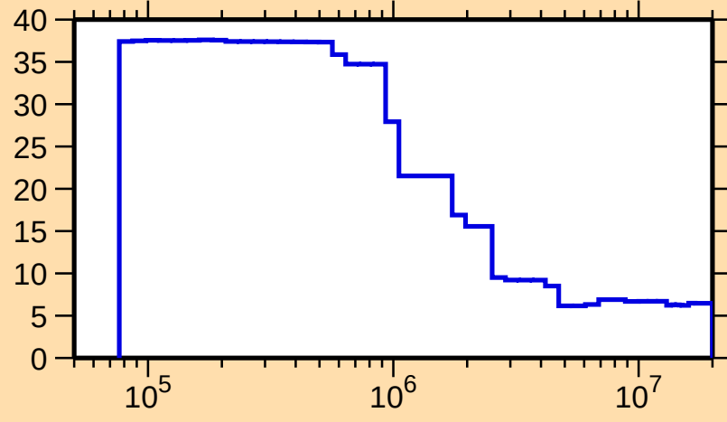
\Delta\sigma/\sigma vs. E for ^{147}\text{Er}(n,\text{nonel.})
