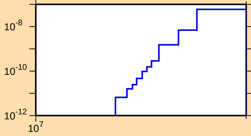
\sigma vs. E for ^{147}\text{Er}(\text{mt } 34)
