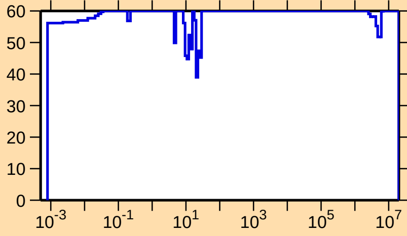
\Delta\sigma/\sigma vs. E for ^{147}\text{Er}(n,\gamma)
