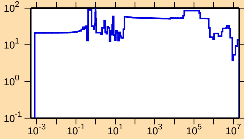
\Delta\sigma/\sigma vs. E for ^{147}\text{Er}(n,\text{el.})
