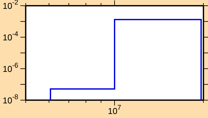
\sigma vs. E for ^{147}\text{Er}(n,\text{pd})
