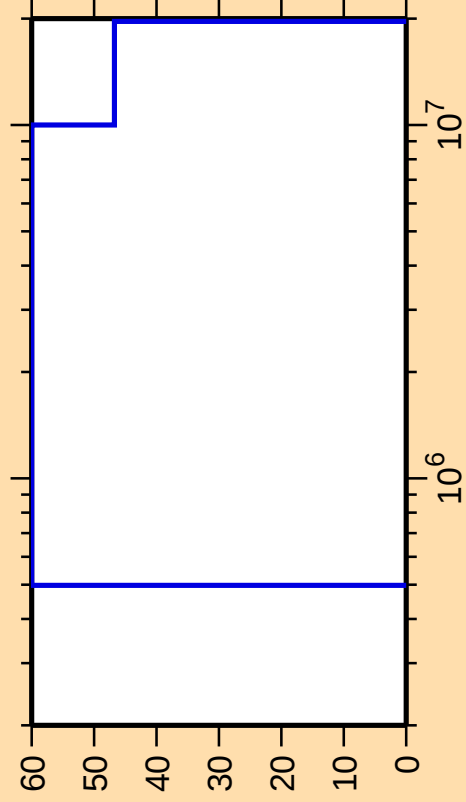
\Delta\sigma/\sigma vs. E for ^{147}\text{Er}(\text{n},\text{ncont.})
