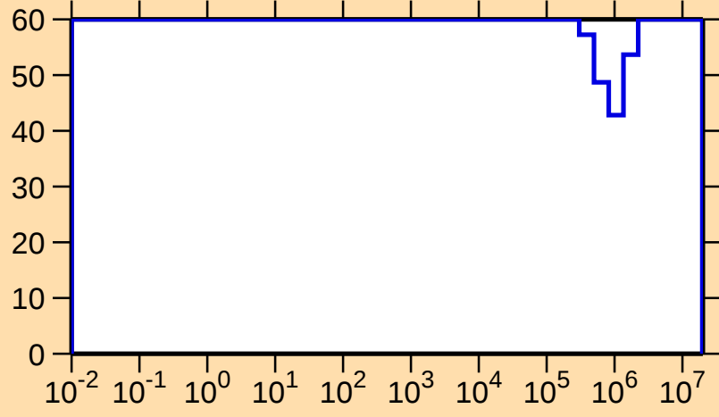
\Delta\sigma/\sigma vs. E for ^{147}\text{Er}(n,p)
