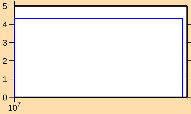
\Delta\sigma/\sigma vs. E for ^{147}\text{Er}(n,\text{tot.})
