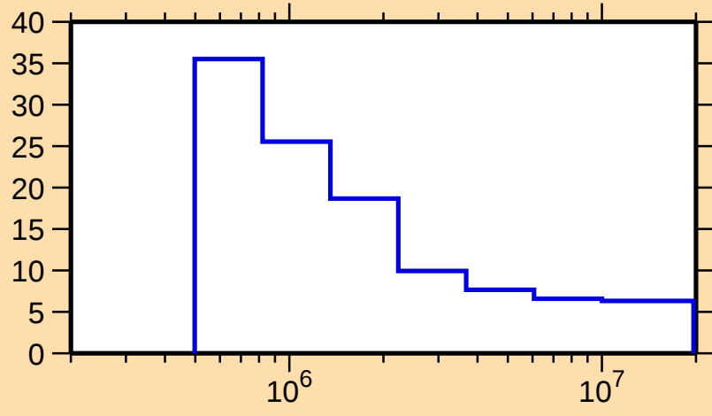
\Delta\sigma/\sigma vs. E for ^{147}\text{Er}(\text{n},\text{nonel.})
