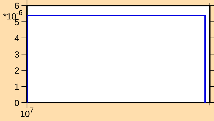
\sigma vs. E for ^{147}\text{Er}(n,2np)
