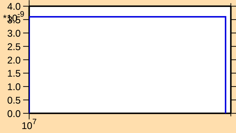
\sigma vs. E for ^{147}\text{Er}(n,2n\alpha)
